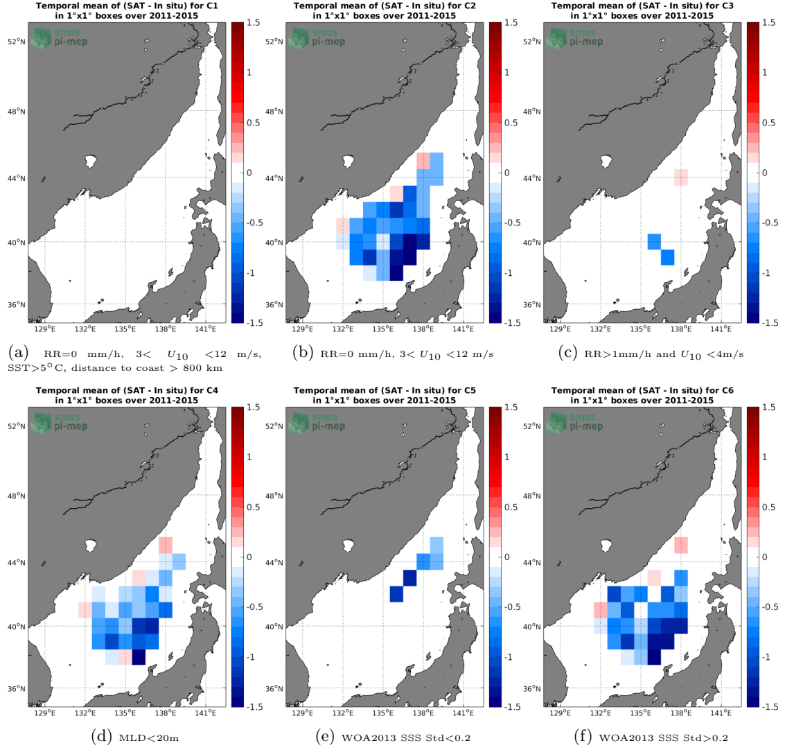
Figure 12: Temporal mean gridded over spatial boxes of size 1^\circ \times 1^\circ of \Delta SSS (Aquarius-L3-JPL-V5-7DAY-RUNNING - Argo) for 6 different subdatasets corresponding to:RR=0 mm/h, 3 < U_{10} < 12 m/s, SST>5°C, distance to coast > 800 km (a), RR=0 mm/h, 3 < U_{10} < 12 m/s (b), RR>1mm/h and U_{10} < 4 m/s (c),MLD<20m (d),WOA2013 SSS Std<0.2 (e),WOA2013 SSS Std>0.2 (f).
