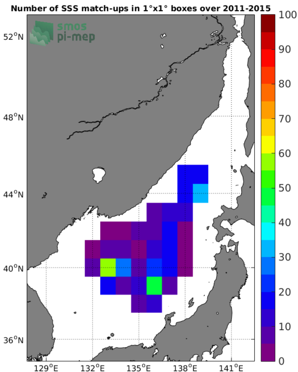
Figure 4: Number of SSS match-ups between Argo SSS and the Aquarius-L3-JPL-V5-7DAY-RUNNING SSS product for the Sea of Japan Pi-MEP region over 1°x1° boxes and for the full satellite product period.
