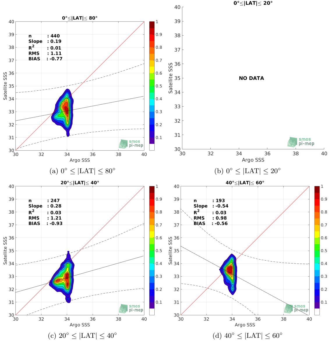
Figure 9: Contour maps of the concentration of Aquarius-L3-JPL-V5-7DAY-RUNNING SSS (y-axis) versus Argo SSS (x-axis) at match-up pairs for different latitudinal bands. For each plot, the red line shows x=y . The black thin and dashed lines indicate a linear fit through the data cloud and the \pm 95\% confidence levels, respectively. The number match-up pairs n , the slope and R^2 coefficient of the linear fit, the root mean square (RMS) and the mean bias between satellite and in situ data are indicated for each latitude band in each plots.
