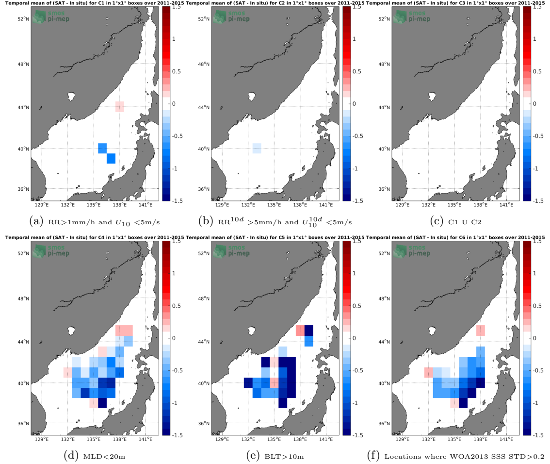
Figure 12: Temporal mean gridded over spatial boxes of size 1^\circ \times 1^\circ of \Delta\text{SSS} (Aquarius-L3-JPL-V5-7DAY-RUNNING - Argo) for 6 different subdatasets corresponding to: \text{RR} > 1\text{mm/h} and U_{10} < 5\text{m/s} (a), \text{RR}^{10d} > 5\text{mm/h} and U_{10}^{10d} < 5\text{m/s} (b), C1 U C2 (c), \text{MLD} < 20\text{m} (d), \text{BLT} > 10\text{m} (e), Locations where WOA2013 SSS STD > 0.2 (f).
