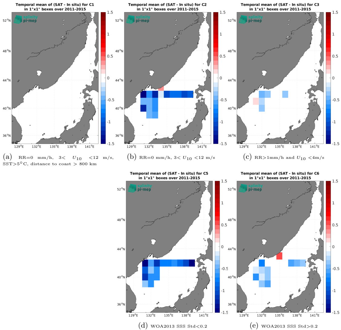
Figure 14: Temporal mean gridded over spatial boxes of size 1^\circ \times 1^\circ of \Delta\text{SSS} (Aquarius SSS L3 CAP v5 - Monthly (JPL) - TSG (LEGOS-DM)) for 5 different subdatasets corresponding to: RR=0 mm/h, 3 < U_{10} < 12 m/s, SST > 5^\circ\text{C} , distance to coast > 800 km (a), RR=0 mm/h, 3 < U_{10} < 12 m/s (b), RR > 1 mm/h and U_{10} < 4 m/s (c), WOA2013 SSS Std < 0.2 (d), WOA2013 SSS Std > 0.2 (e).
