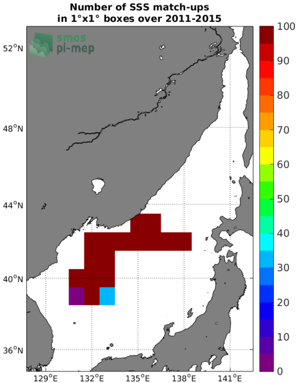
Figure 4: Number of SSS match-ups between TSG-LEGOS-DM SSS and the Aquarius-L3-JPL-V5-MONTHLY SSS product for the Sea of Japan Pi-MEP region over 1°x1° boxes and for the full satellite product period.
