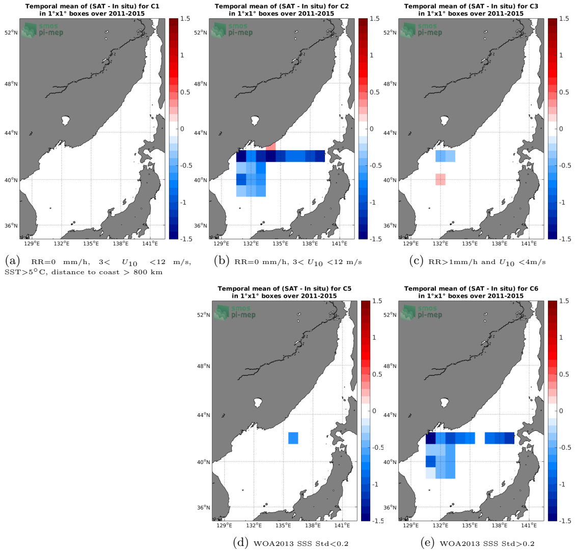
Figure 12: Temporal mean gridded over spatial boxes of size 1^\circ \times 1^\circ of \Delta\text{SSS} (Aquarius-L3-JPL-V5-MONTHLY - TSG-LEGOS-DM) for 5 different subdatasets corresponding to: RR=0 mm/h, 3 < U_{10} < 12 m/s, SST > 5^\circ\text{C} , distance to coast > 800 km (a), RR=0 mm/h, 3 < U_{10} < 12 m/s (b), RR > 1 mm/h and U_{10} < 4 m/s (c), WOA2013 SSS Std < 0.2 (d), WOA2013 SSS Std > 0.2 (e).
