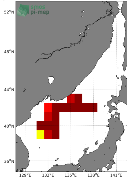
(c) MEAN(TSG-LEGOS-DM SSS)
