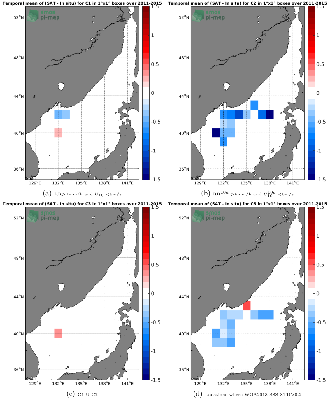
Figure 12: Temporal mean gridded over spatial boxes of size 1°x1° of \Delta\text{SSS} (Aquarius-L3-JPL-V5-MONTHLY - TSG-LEGOS-DM) for 4 different subdatasets corresponding to: RR > 1\text{mm/h} and U_{10} < 5\text{m/s} (a), RR^{10d} > 5\text{mm/h} and U_{10}^{10d} < 5\text{m/s} (b), C1 U C2 (c), Locations where WOA2013 SSS STD > 0.2 (d).
