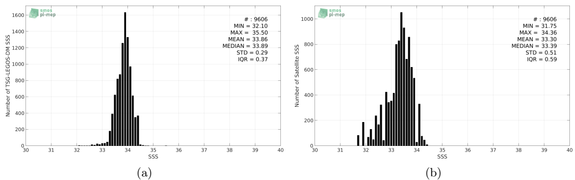
Figure 2: Histograms of SSS from TSG-LEGOS-DM (a) and Aquarius-L3-JPL-V5-MONTHLY (b) considering all match-up pairs per bins of 0.1 over the Sea of Japan Pi-MEP region and for the full satellite product period.
