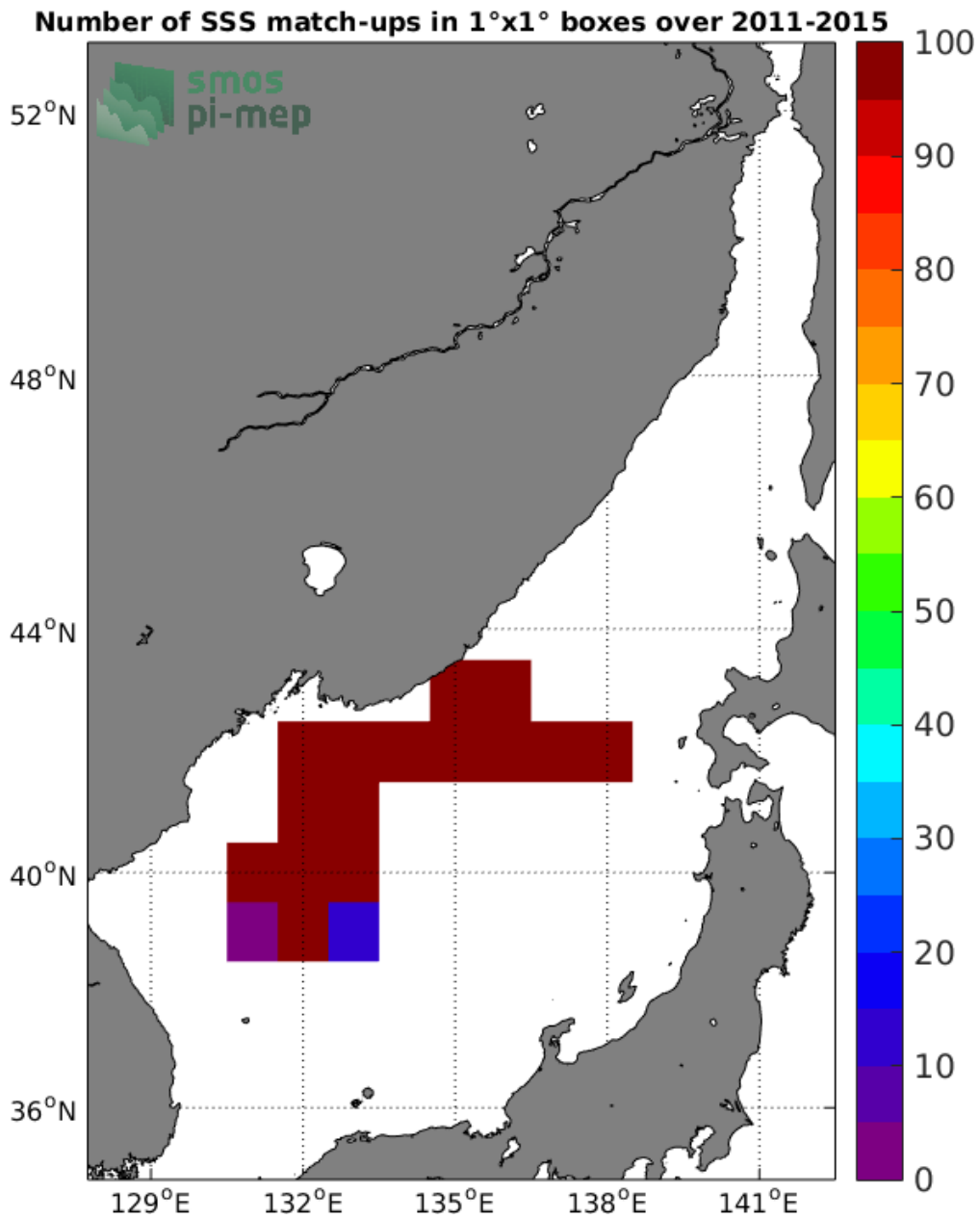
Figure 4: Number of SSS match-ups between TSG-LEGOS-DM SSS and the Aquarius-L3-JPL-V5-MONTHLY SSS product for the Sea of Japan Pi-MEP region over 1°x1° boxes and for the full satellite product period.
