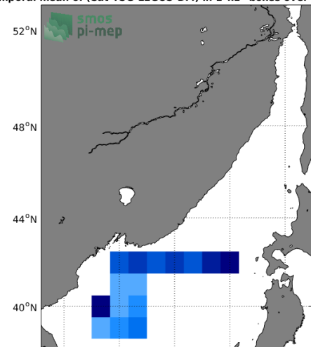
Temporal mean of (Sat-TSG-LEGOS-DM) in 1°x1° boxes over 2011-2015
