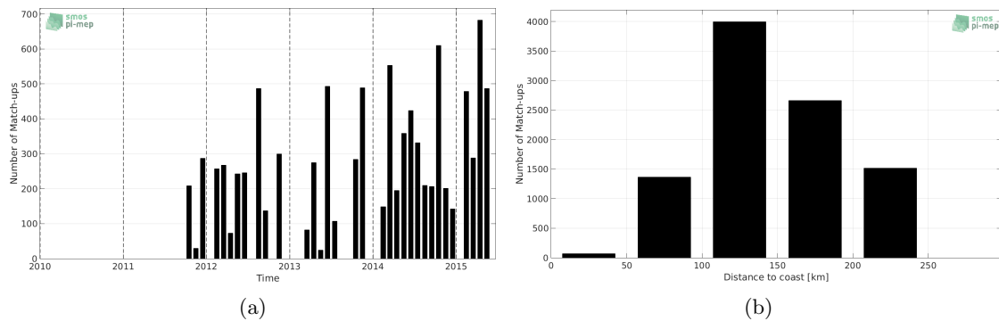
Figure 1: Number of match-ups between TSG-LEGOS-DM and Aquarius-L3-JPL-V5-MONTHLY SSS as a function of time (a) and as function of the distance to coast (b) over the Sea of Japan Pi-MEP region and for the full satellite product period.
