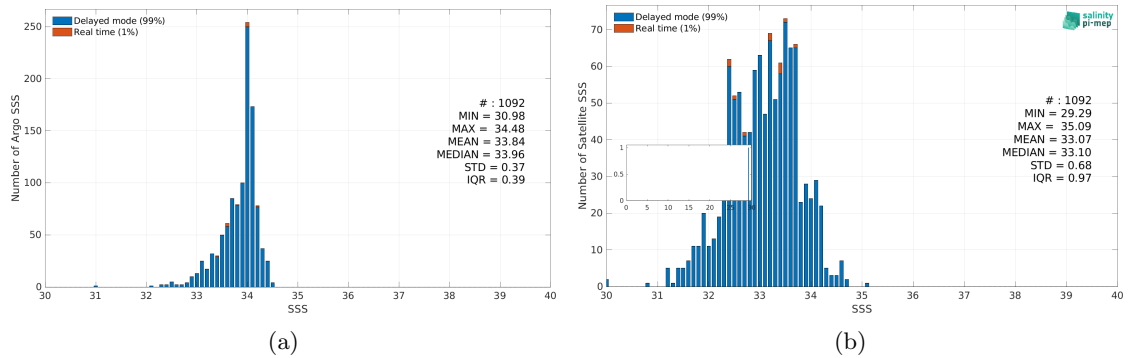
Figure 3: Histograms of SSS from Argo (a) and Aquarius SSS L3 CAP v5 - Monthly (JPL) (b) considering all match-up pairs per bins of 0.1 over the Sea of Japan Pi-MEP region and for the full satellite product period.
