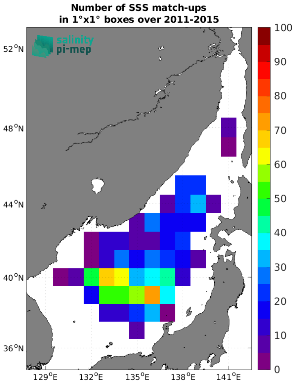
Figure 5: Number of SSS match-ups between Argo SSS and the Aquarius SSS L3 CAP v5 - Monthly (JPL) SSS product for the Sea of Japan Pi-MEP region over 1°x1° boxes and for the full satellite product period.
