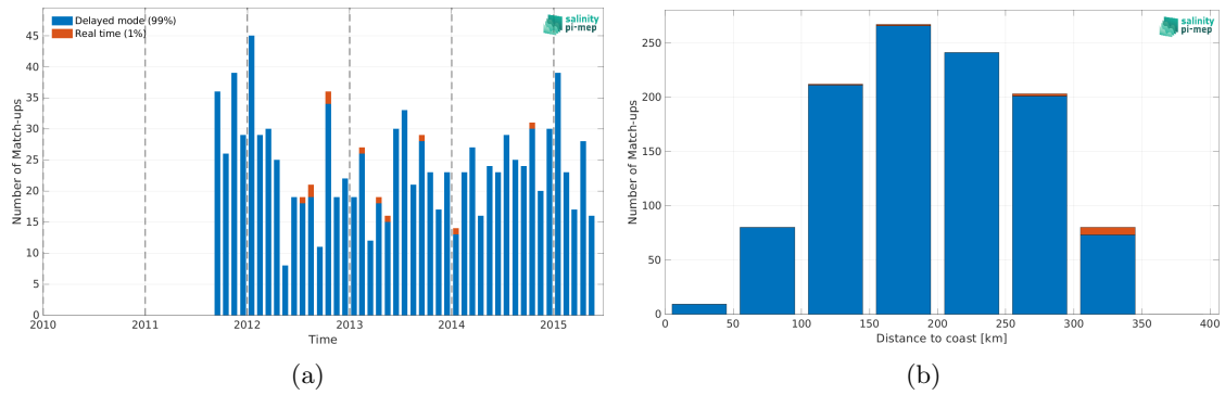
Figure 2: Number of match-ups between Argo and Aquarius SSS L3 CAP v5 - Monthly (JPL) SSS as a function of time (a) and as function of the distance to coast (b) over the Sea of Japan Pi-MEP region and for the full satellite product period.
