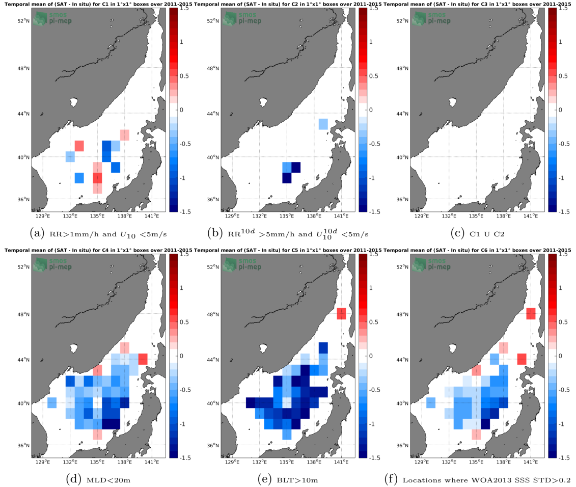
Figure 12: Temporal mean gridded over spatial boxes of size 1°x1° of \Delta SSS (Aquarius-L3-JPL-V5-MONTHLY - Argo) for 6 different subdatasets corresponding to: RR > 1\text{mm/h} and U_{10} < 5\text{m/s} (a), RR^{10d} > 5\text{mm/h} and U_{10}^{10d} < 5\text{m/s} (b), C1 U C2 (c), MLD < 20\text{m} (d), BLT > 10\text{m} (e), Locations where WOA2013 SSS STD > 0.2 (f).
