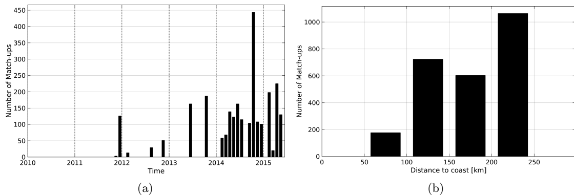
Figure 1: Number of match-ups between TSG-LEGOS-DM and Aquarius-L3-JPL-V4-7DAY-RUNNING SSS as a function of time (a) and as function of the distance to coast (b) over the Sea of Japan Pi-MEP region and for the full satellite product period.
