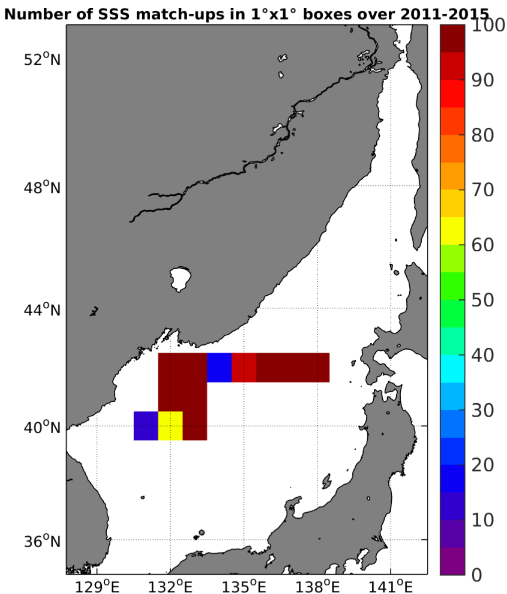
Figure 4: Number of SSS match-ups between TSG-LEGOS-DM SSS and the Aquarius-L3-JPL-V4-7DAY-RUNNING SSS product for the Sea of Japan Pi-MEP region over 1°x1° boxes and for the full satellite product period.
