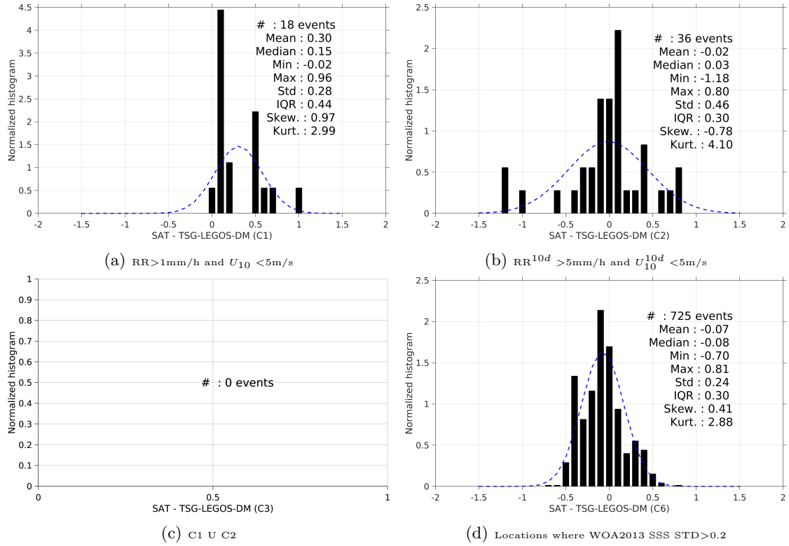
Figure 13: Normalized histogram of \Delta\text{SSS} (Aquarius-L3-JPL-V4-7DAY-RUNNING - TSG-LEGOS-DM) for 6 different subdatasets corresponding to: RR>1mm/h and U_{10} < 5\text{m/s} (a), RR^{10d} > 5\text{mm/h} and U_{10}^{10d} < 5\text{m/s} (b), C1 U C2 (c), Locations where WOA2013 SSS STD>0.2 (d).
