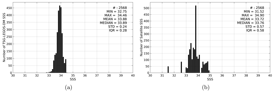
Figure 2: Histograms of SSS from TSG-LEGOS-DM (a) and Aquarius-L3-JPL-V4-7DAY-RUNNING (b) considering all match-up pairs per bins of 0.1 over the Sea of Japan Pi-MEP region and for the full satellite product period.
