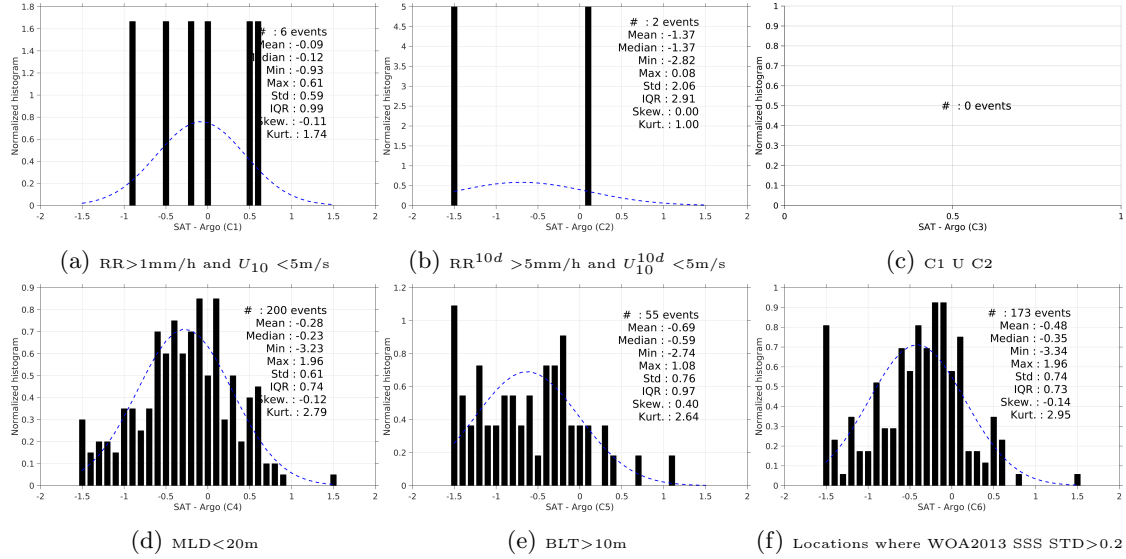
Figure 13: Normalized histogram of \Delta SSS (Aquarius-L3-JPL-V4-7DAY-RUNNING - Argo) for 6 different subdatasets corresponding to: RR > 1\text{mm/h} and U_{10} < 5\text{m/s} (a), RR^{10d} > 5\text{mm/h} and U_{10}^{10d} < 5\text{m/s} (b), C1 \cup C2 (c), MLD < 20\text{m} (d), BLT > 10\text{m} (e), Locations where WOA2013 SSS STD > 0.2 (f).
