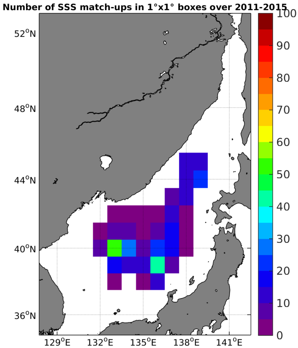
Figure 4: Number of SSS match-ups between Argo SSS and the Aquarius-L3-JPL-V4-7DAY-RUNNING SSS product for the Sea of Japan Pi-MEP region over 1°x1° boxes and for the full satellite product period.
