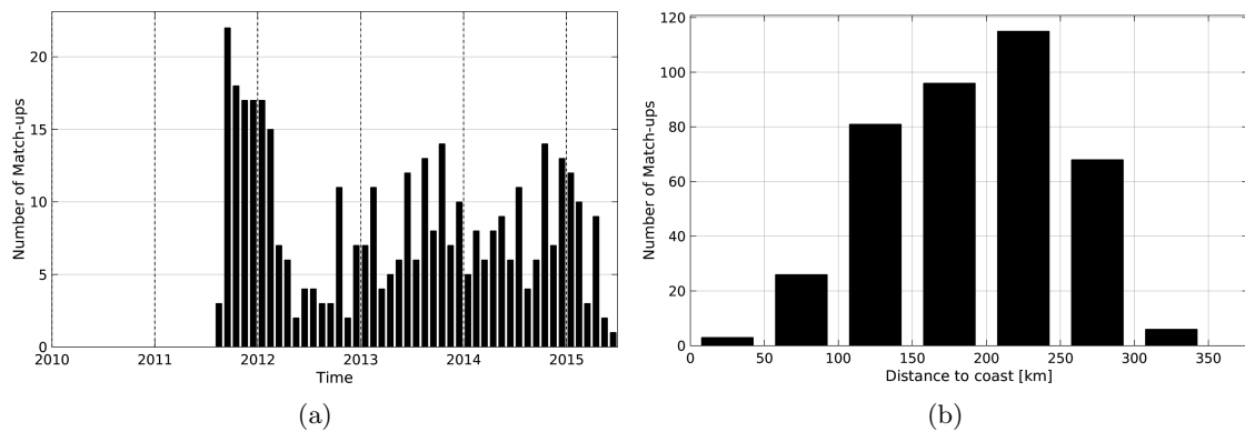
Figure 1: Number of match-ups between Argo and Aquarius-L3-JPL-V4-7DAY-RUNNING SSS as a function of time (a) and as function of the distance to coast (b) over the Sea of Japan Pi-MEP region and for the full satellite product period.
