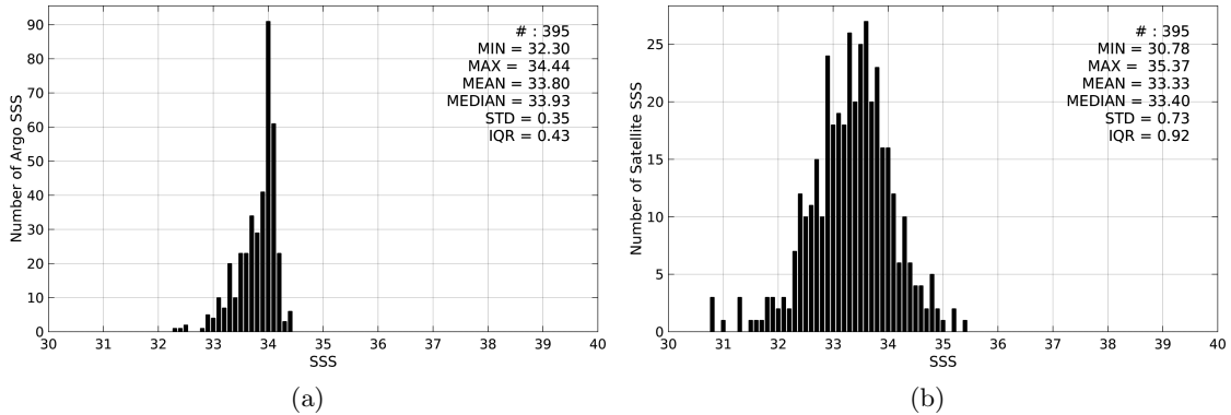
Figure 2: Histograms of SSS from Argo (a) and Aquarius-L3-JPL-V4-7DAY-RUNNING (b) considering all match-up pairs per bins of 0.1 over the Sea of Japan Pi-MEP region and for the full satellite product period.
