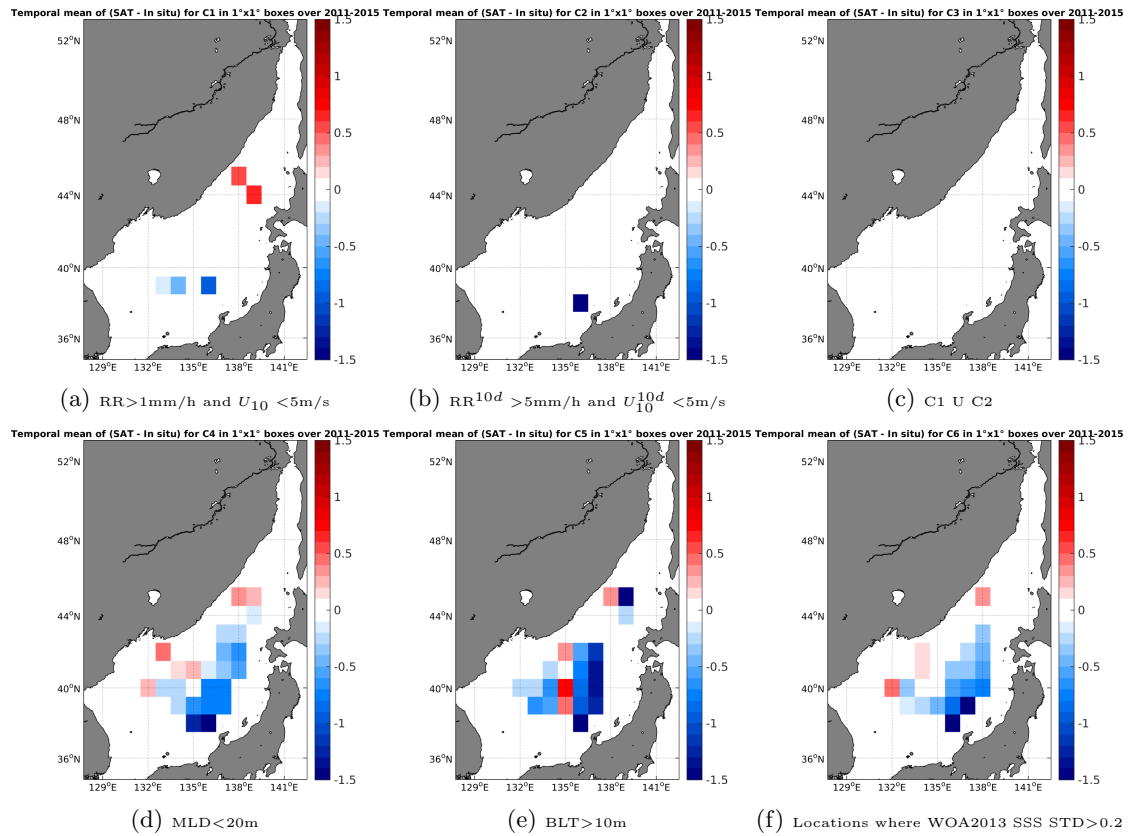
Figure 12: Temporal mean gridded over spatial boxes of size 1^\circ \times 1^\circ of \Delta SSS (Aquarius-L3-JPL-V4-7DAY-RUNNING - Argo) for 6 different subdatasets corresponding to: RR > 1\text{mm/h} and U_{10} < 5\text{m/s} (a), RR^{10d} > 5\text{mm/h} and U_{10}^{10d} < 5\text{m/s} (b), C1 U C2 (c), MLD < 20\text{m} (d), BLT > 10\text{m} (e), Locations where WOA2013 SSS STD > 0.2 (f).
