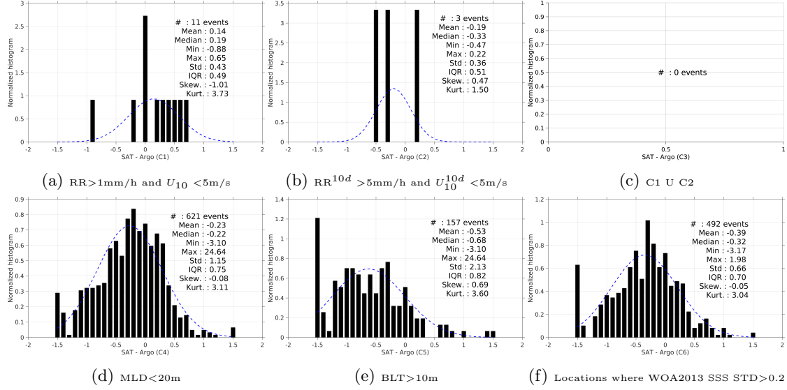
Figure 13: Normalized histogram of \Delta SSS (Aquarius-L3-JPL-V4-MONTHLY - Argo) for 6 different subdatasets corresponding to: RR > 1\text{mm/h} and U_{10} < 5\text{m/s} (a), RR^{10d} > 5\text{mm/h} and U_{10}^{10d} < 5\text{m/s} (b), C1 \cup C2 (c), MLD < 20\text{m} (d), BLT > 10\text{m} (e), Locations where WOA2013 SSS STD > 0.2 (f).
