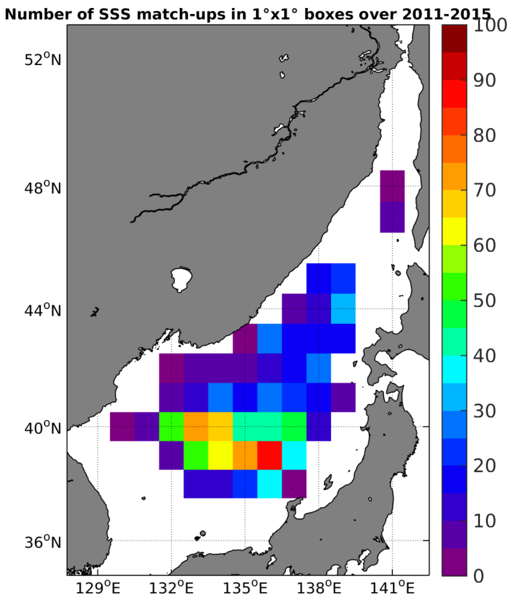
Figure 4: Number of SSS match-ups between Argo SSS and the Aquarius-L3-JPL-V4-MONTHLY SSS product for the Sea of Japan Pi-MEP region over 1°x1° boxes and for the full satellite product period.
