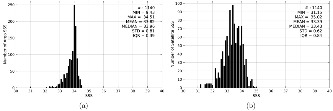
Figure 2: Histograms of SSS from Argo (a) and Aquarius-L3-JPL-V4-MONTHLY (b) considering all match-up pairs per bins of 0.1 over the Sea of Japan Pi-MEP region and for the full satellite product period.
