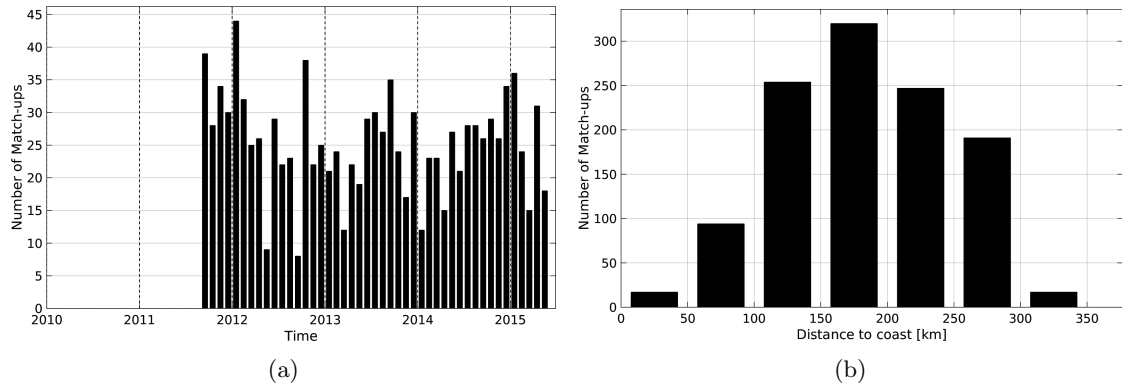
Figure 1: Number of match-ups between Argo and Aquarius-L3-JPL-V4-MONTHLY SSS as a function of time (a) and as function of the distance to coast (b) over the Sea of Japan Pi-MEP region and for the full satellite product period.
