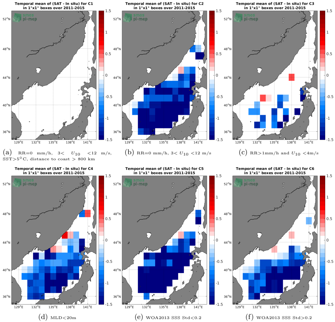
Figure 12: Temporal mean gridded over spatial boxes of size 1°x1° of \Delta SSS (Aquarius SSS L2-AVERAGED OR v5 (NASA-GSFC) - Argo) for 6 different subdatasets corresponding to:RR=0 mm/h, 3 < U_{10} < 12 m/s, SST > 5°C, distance to coast > 800 km (a), RR=0 mm/h, 3 < U_{10} < 12 m/s (b), RR > 1mm/h and U_{10} < 4 m/s (c),MLD < 20m (d),WOA2013 SSS Std < 0.2 (e),WOA2013 SSS Std > 0.2 (f).
