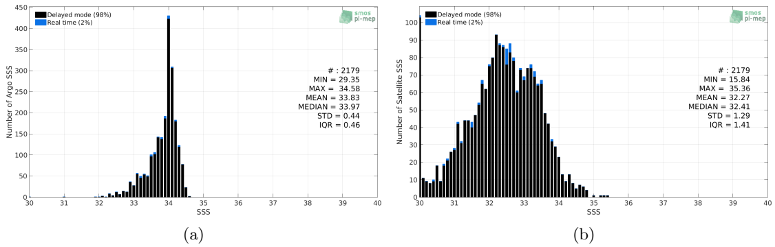
Figure 2: Histograms of SSS from Argo (a) and Aquarius SSS L2-AVERAGED OR v5 (NASA-GSFC) (b) considering all match-up pairs per bins of 0.1 over the Sea of Japan Pi-MEP region and for the full satellite product period.
