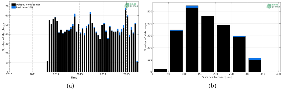
Figure 1: Number of match-ups between Argo and Aquarius SSS L2-AVERAGED OR v5 (NASA-GSFC) SSS as a function of time (a) and as function of the distance to coast (b) over the Sea of Japan Pi-MEP region and for the full satellite product period.
