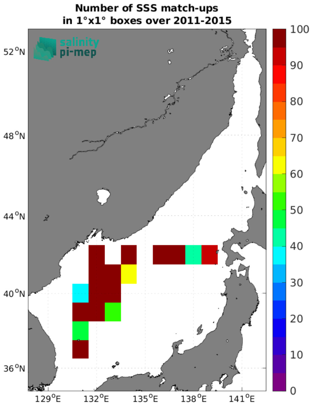
Figure 5: Number of SSS match-ups between TSG (LEGOS-DM) SSS and the Aquarius SSS L2 OR v5 (NASA-GSFC) SSS product for the Sea of Japan Pi-MEP region over 1°×1° boxes and for the full satellite product period.
