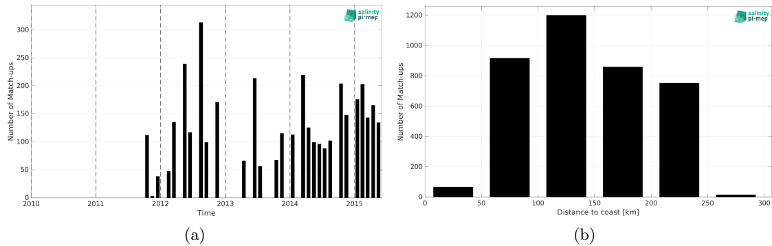
Figure 2: Number of match-ups between TSG (LEGOS-DM) and Aquarius SSS L2 OR v5 (NASA-GSFC) SSS as a function of time (a) and as function of the distance to coast (b) over the Sea of Japan Pi-MEP region and for the full satellite product period.
