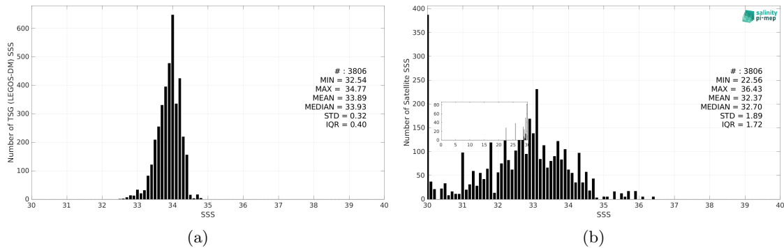
Figure 3: Histograms of SSS from TSG (LEGOS-DM) (a) and Aquarius SSS L2 OR v5 (NASA-GSFC) (b) considering all match-up pairs per bins of 0.1 over the Sea of Japan Pi-MEP region and for the full satellite product period.
