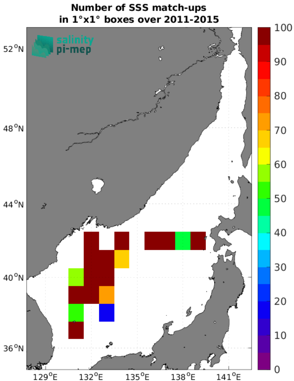
Figure 4: Number of SSS match-ups between TSG (LEGOS-DM) SSS and the Aquarius SSS L2 OR v5 (NASA-GSFC) SSS product for the Sea of Japan Pi-MEP region over 1°×1° boxes and for the full satellite product period.
