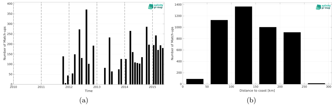
Figure 1: Number of match-ups between TSG (LEGOS-DM) and Aquarius SSS L2 OR v5 (NASA-GSFC) SSS as a function of time (a) and as function of the distance to coast (b) over the Sea of Japan Pi-MEP region and for the full satellite product period.
