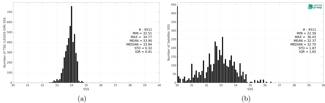
Figure 2: Histograms of SSS from TSG (LEGOS-DM) (a) and Aquarius SSS L2 OR v5 (NASA-GSFC) (b) considering all match-up pairs per bins of 0.1 over the Sea of Japan Pi-MEP region and for the full satellite product period.
