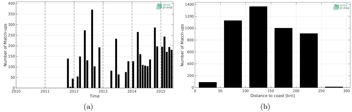
Figure 1: Number of match-ups between TSG-LEGOS-DM and Aquarius-L2-OR-V5 SSS as a function of time (a) and as function of the distance to coast (b) over the Sea of Japan Pi-MEP region and for the full satellite product period.
