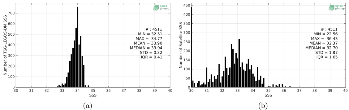
Figure 2: Histograms of SSS from TSG-LEGOS-DM (a) and Aquarius-L2-OR-V5 (b) considering all match-up pairs per bins of 0.1 over the Sea of Japan Pi-MEP region and for the full satellite product period.
