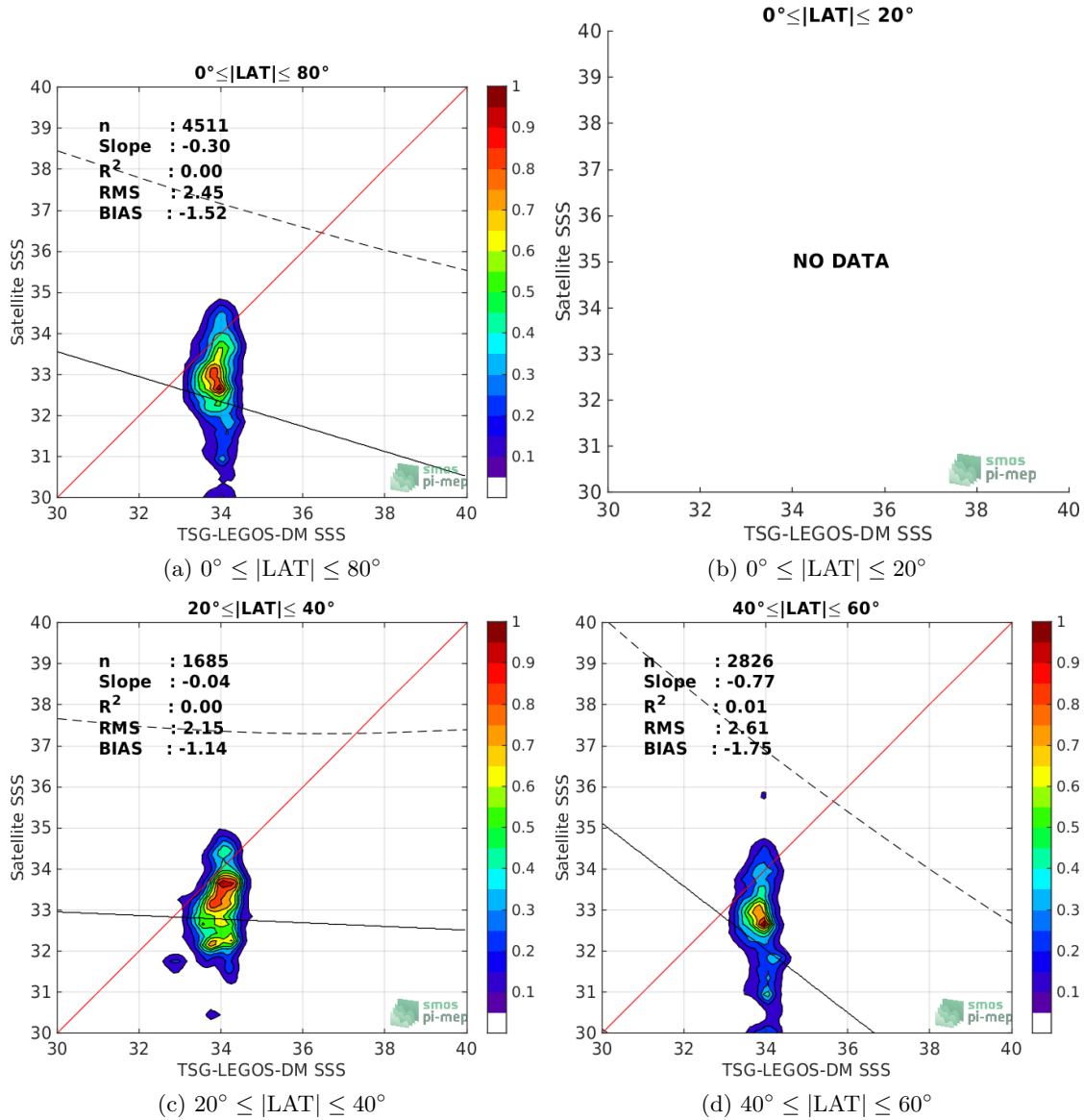
Figure 9: Contour maps of the concentration of Aquarius-L2-OR-V5 SSS (y-axis) versus TSG-LEGOS-DM SSS (x-axis) at match-up pairs for different latitude bands. For each plot, the red line shows x=y . The black thin and dashed lines indicate a linear fit through the data cloud and the \pm 95\% confidence levels, respectively. The number match-up pairs n , the slope and R^2 coefficient of the linear fit, the root mean square (RMS) and the mean bias between satellite and in situ data are indicated for each latitude band in each plots.
