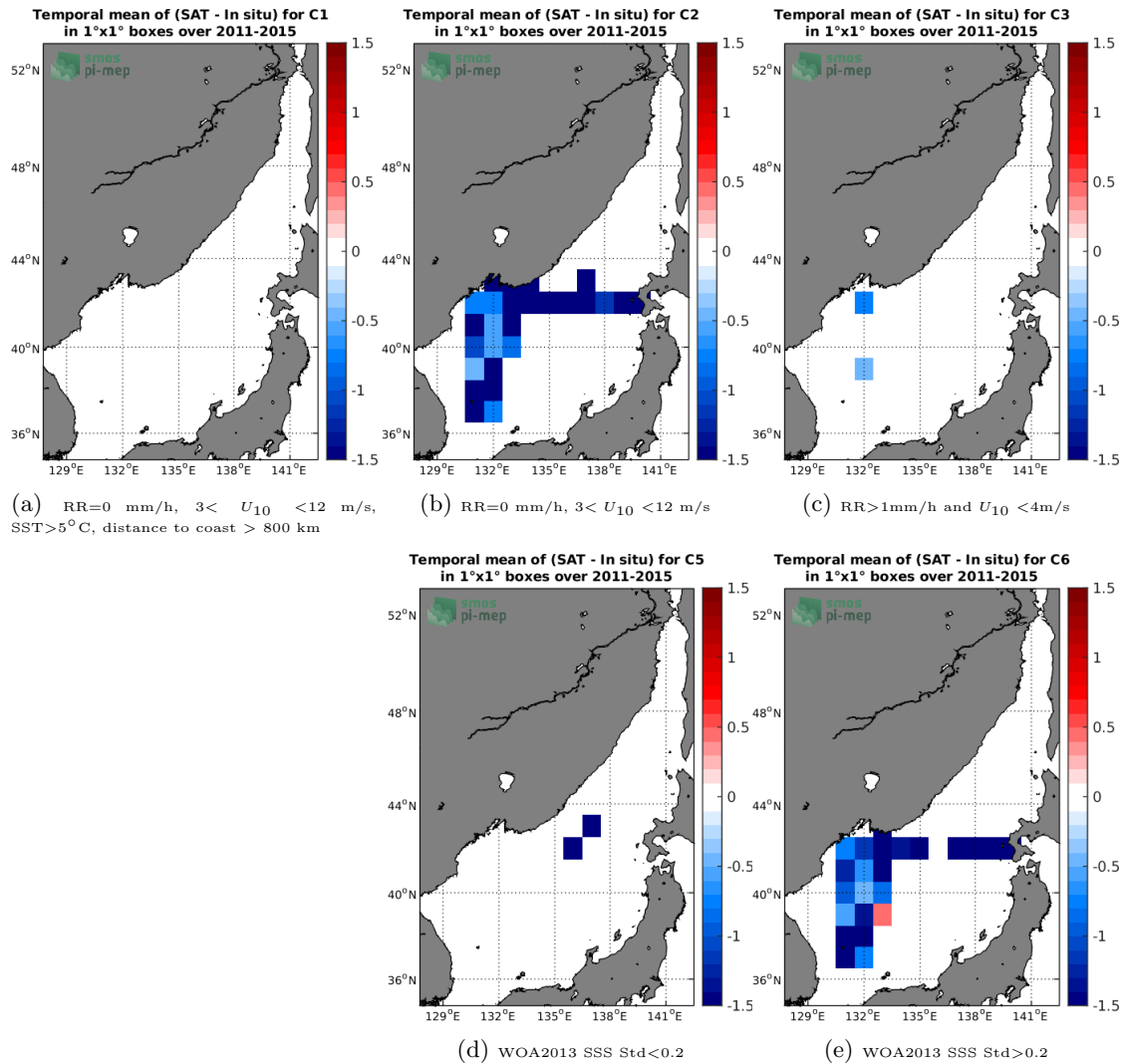
Figure 12: Temporal mean gridded over spatial boxes of size 1^\circ \times 1^\circ of \Delta SSS (Aquarius-L2-OR-V5 - TSG-LEGOS-DM) for 5 different subdatasets corresponding to: RR=0 mm/h, 3 < U_{10} < 12 m/s, SST > 5^\circ\text{C} , distance to coast > 800 km (a), RR=0 mm/h, 3 < U_{10} < 12 m/s (b), RR > 1 mm/h and U_{10} < 4 m/s (c), WOA2013 SSS Std < 0.2 (d), WOA2013 SSS Std > 0.2 (e).
