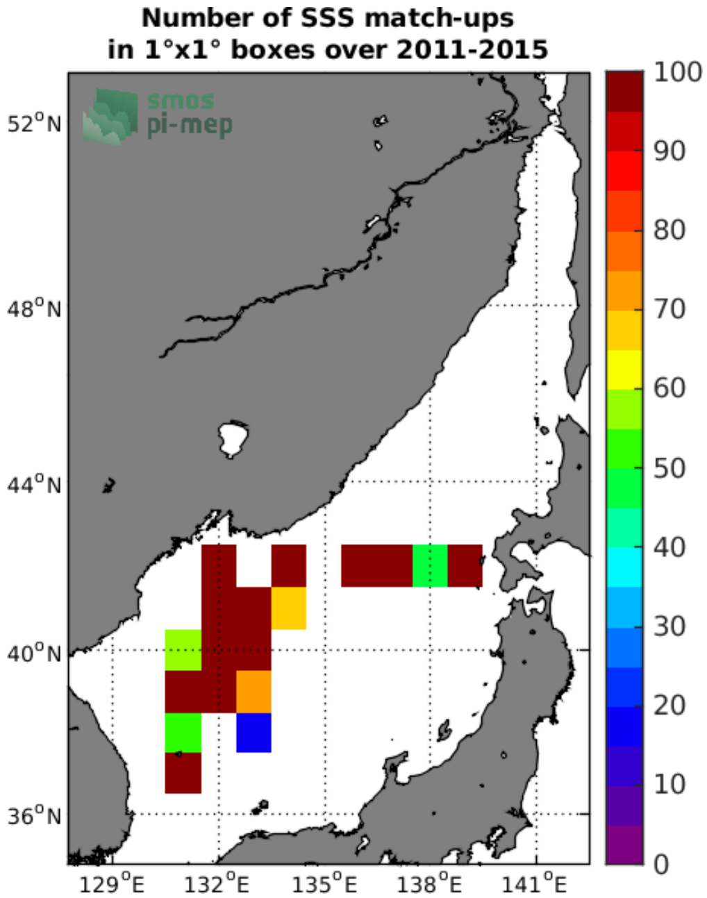
Figure 4: Number of SSS match-ups between TSG-LEGOS-DM SSS and the Aquarius-L2-OR-V5 SSS product for the Sea of Japan Pi-MEP region over 1°x1° boxes and for the full satellite product period.
