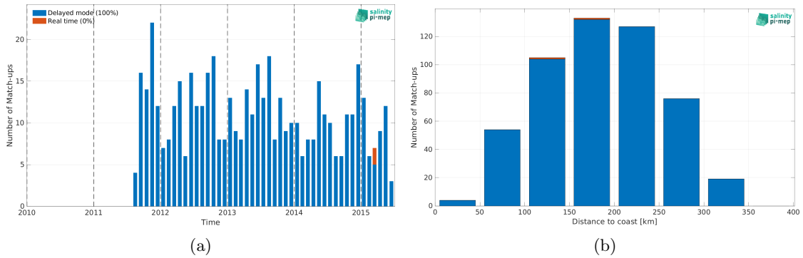
Figure 2: Number of match-ups between Argo and Aquarius SSS L2 OR v5 (NASA-GSFC) SSS as a function of time (a) and as function of the distance to coast (b) over the Sea of Japan Pi-MEP region and for the full satellite product period.
