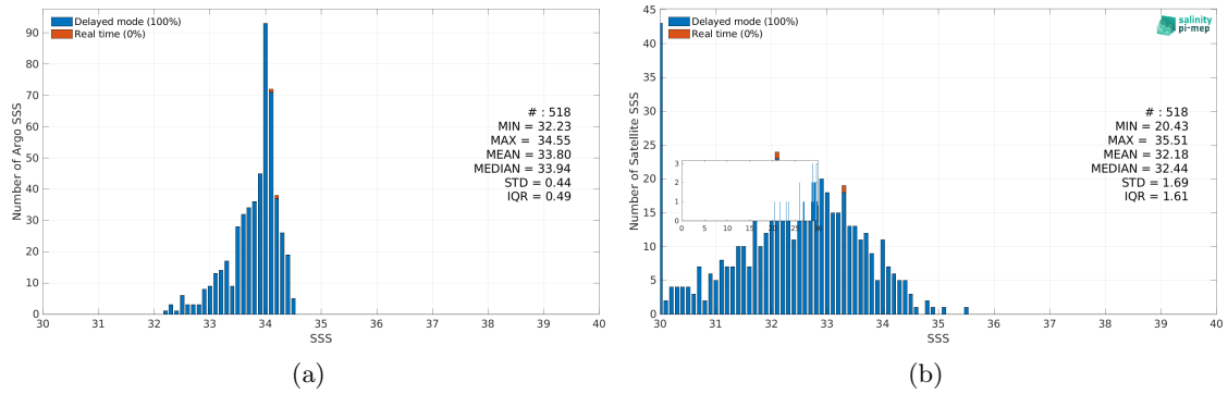
Figure 3: Histograms of SSS from Argo (a) and Aquarius SSS L2 OR v5 (NASA-GSFC) (b) considering all match-up pairs per bins of 0.1 over the Sea of Japan Pi-MEP region and for the full satellite product period.
