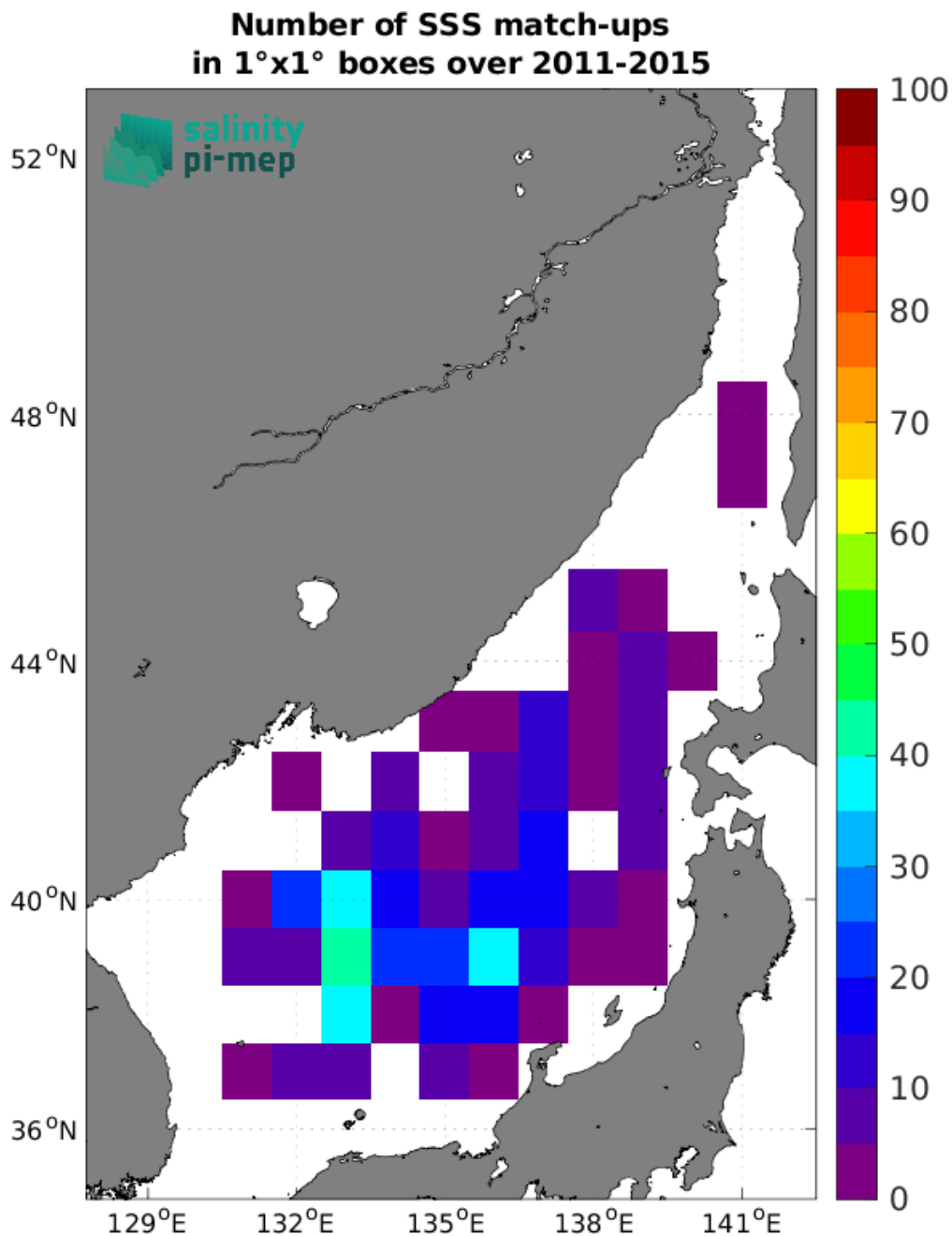
Figure 5: Number of SSS match-ups between Argo SSS and the Aquarius SSS L2 OR v5 (NASA-GSFC) SSS product for the Sea of Japan Pi-MEP region over 1^\circ \times 1^\circ boxes and for the full satellite product period.
