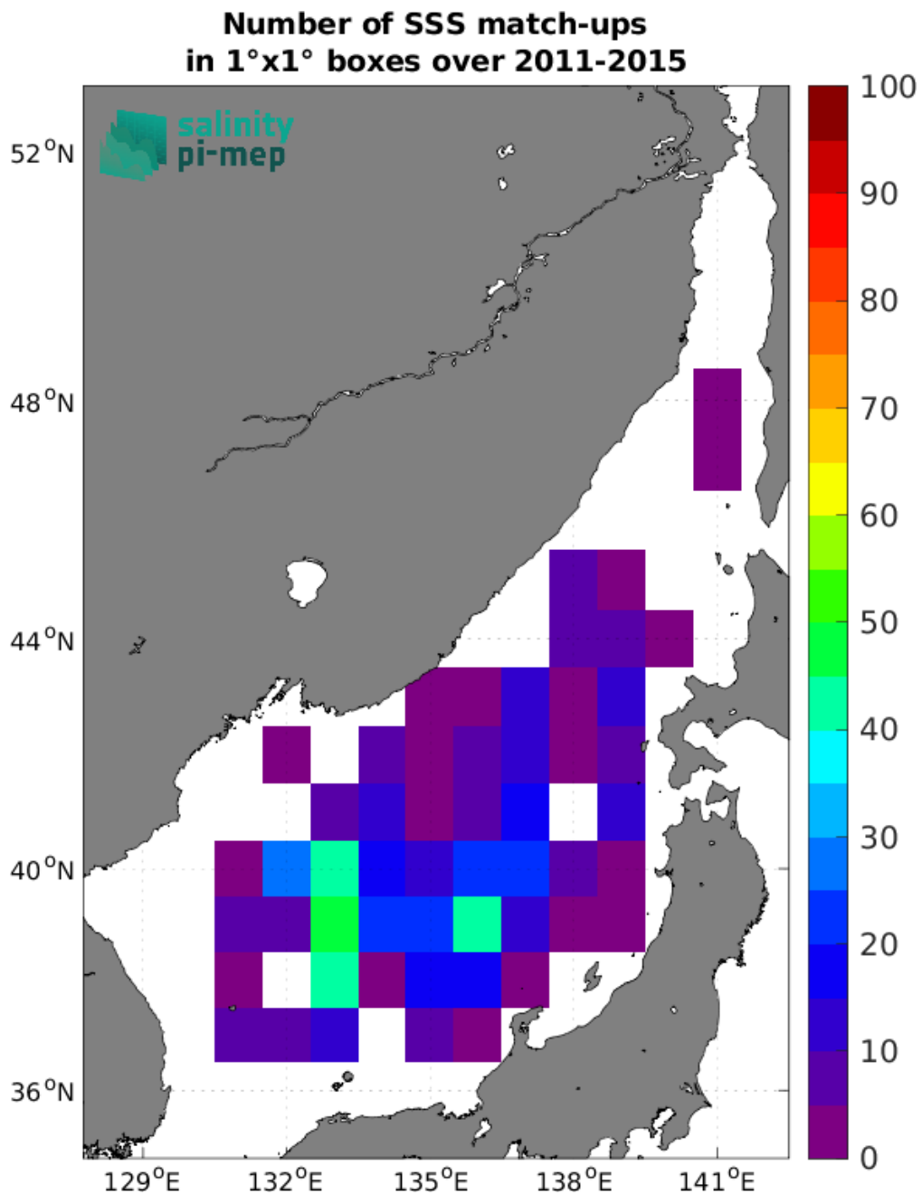
Figure 4: Number of SSS match-ups between Argo SSS and the Aquarius SSS L2 OR v5 (NASA-GSFC) SSS product for the Sea of Japan Pi-MEP region over 1^\circ \times 1^\circ boxes and for the full satellite product period.
