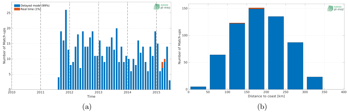
Figure 1: Number of match-ups between Argo and Aquarius SSS L2 OR v5 (NASA-GSFC) SSS as a function of time (a) and as function of the distance to coast (b) over the Sea of Japan Pi-MEP region and for the full satellite product period.
