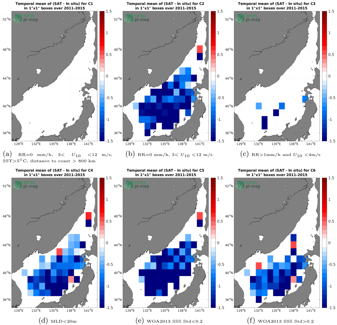
Figure 12: Temporal mean gridded over spatial boxes of size 1^\circ \times 1^\circ of \Delta SSS (Aquarius SSS L2 OR v5 (NASA-GSFC) - Argo) for 6 different subdatasets corresponding to: RR=0 mm/h, 3 < U_{10} < 12 m/s, SST > 5^\circ C , distance to coast > 800 km (a), RR=0 mm/h, 3 < U_{10} < 12 m/s (b), RR > 1 mm/h and U_{10} < 4 m/s (c), MLD < 20 m (d), WOA2013 SSS Std < 0.2 (e), WOA2013 SSS Std > 0.2 (f).
