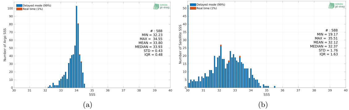
Figure 2: Histograms of SSS from Argo (a) and Aquarius SSS L2 OR v5 (NASA-GSFC) (b) considering all match-up pairs per bins of 0.1 over the Sea of Japan Pi-MEP region and for the full satellite product period.
