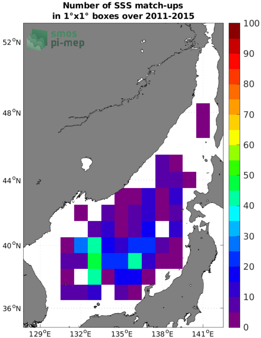
Figure 4: Number of SSS match-ups between Argo SSS and the Aquarius SSS L2 OR v5 (NASA-GSFC) SSS product for the Sea of Japan Pi-MEP region over 1°×1° boxes and for the full satellite product period.
