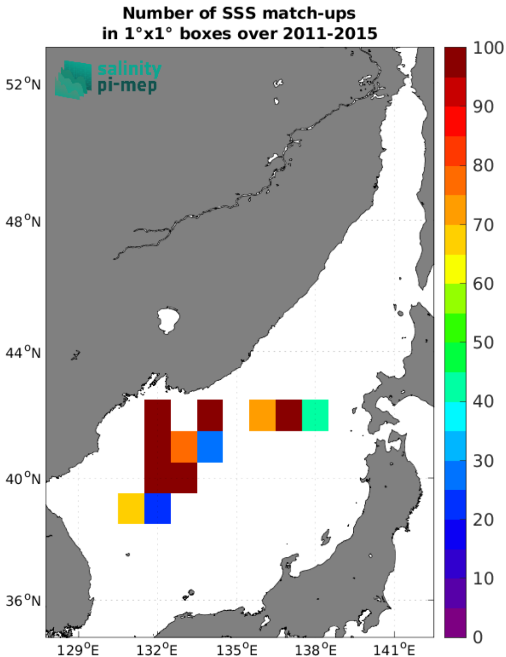
Figure 5: Number of SSS match-ups between TSG (LEGOS-DM) SSS and the Aquarius SSS L2 CAP v5 (JPL) SSS product for the Sea of Japan Pi-MEP region over 1°x1° boxes and for the full satellite product period.
