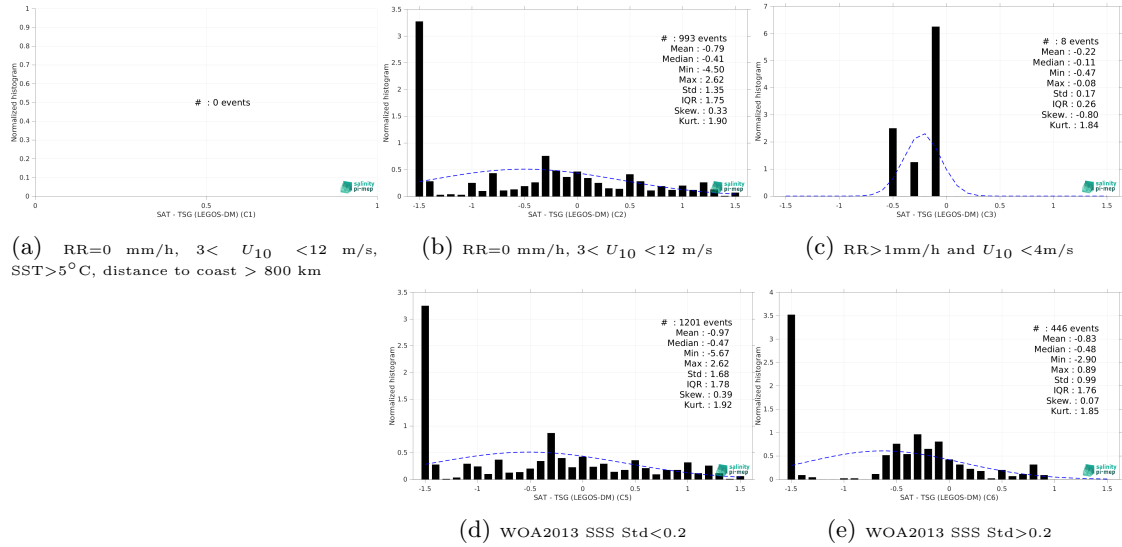
Figure 15: Normalized histogram of \Delta\text{SSS} (Aquarius SSS L2 CAP v5 (JPL) - TSG (LEGOS-DM)) for 5 different subdatasets corresponding to: \text{RR}=0 mm/h, 3 < U_{10} < 12 m/s, \text{SST} > 5^\circ\text{C} , distance to coast > 800 km (a), \text{RR}=0 mm/h, 3 < U_{10} < 12 m/s (b), \text{RR} > 1 mm/h and U_{10} < 4 m/s (c), WOA2013 SSS Std < 0.2 (d), WOA2013 SSS Std > 0.2 (e).
