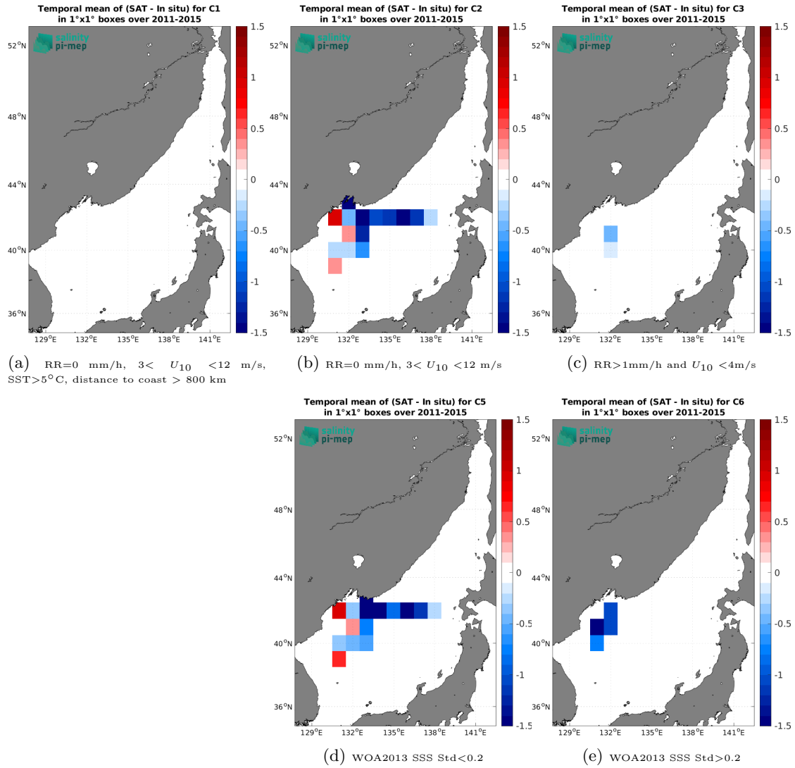
Figure 14: Temporal mean gridded over spatial boxes of size 1^\circ \times 1^\circ of \Delta SSS (Aquarius SSS L2 CAP v5 (JPL) - TSG (LEGOS-DM)) for 5 different subdatasets corresponding to: RR=0 mm/h, 3 < U_{10} < 12 m/s, SST > 5^\circ C , distance to coast > 800 km (a), RR=0 mm/h, 3 < U_{10} < 12 m/s (b), RR > 1 mm/h and U_{10} < 4 m/s (c), WOA2013 SSS Std < 0.2 (d), WOA2013 SSS Std > 0.2 (e).
