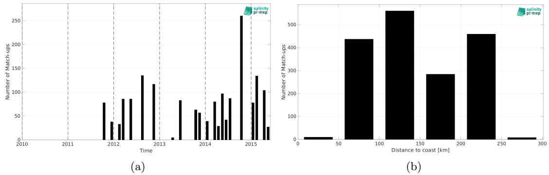
Figure 2: Number of match-ups between TSG (LEGOS-DM) and Aquarius SSS L2 CAP v5 (JPL) SSS as a function of time (a) and as function of the distance to coast (b) over the Sea of Japan Pi-MEP region and for the full satellite product period.
