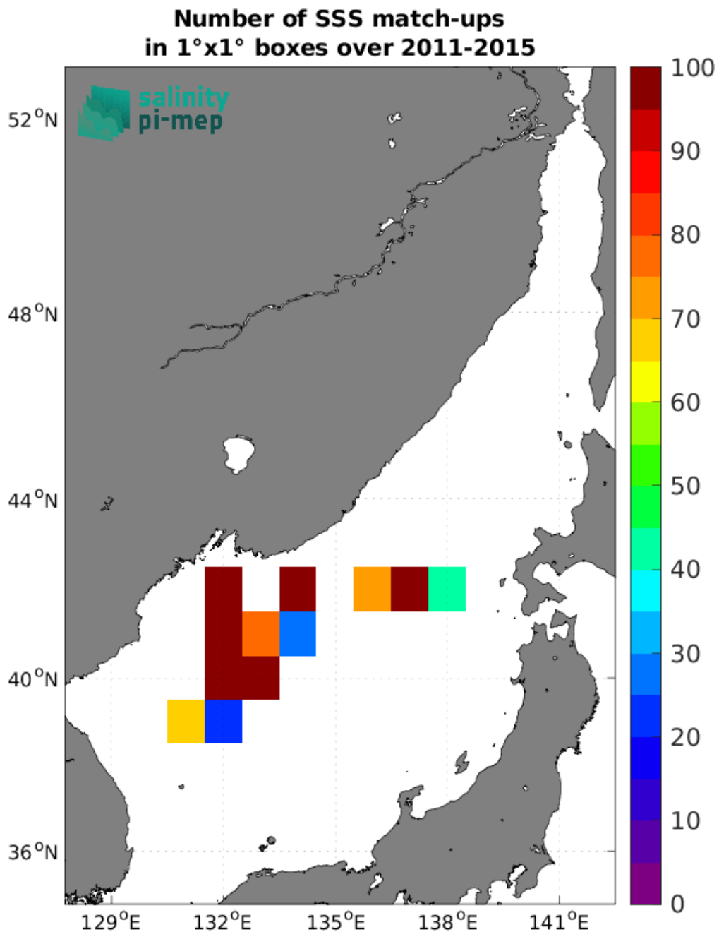
Figure 5: Number of SSS match-ups between TSG (LEGOS-DM) SSS and the Aquarius SSS L2 CAP v5 (JPL) SSS product for the Sea of Japan Pi-MEP region over 1°×1° boxes and for the full satellite product period.
