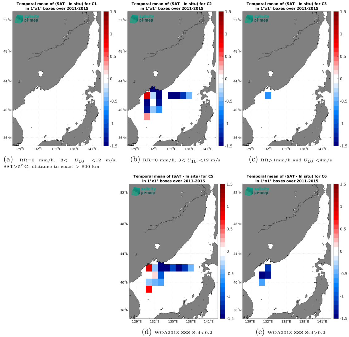
Figure 12: Temporal mean gridded over spatial boxes of size 1^\circ \times 1^\circ of \Delta\text{SSS} (Aquarius SSS L2 CAP v5 (JPL) - TSG (LEGOS-DM)) for 5 different subdatasets corresponding to: RR=0 mm/h, 3 < U_{10} < 12 m/s, SST > 5^\circ\text{C} , distance to coast > 800 km (a), RR=0 mm/h, 3 < U_{10} < 12 m/s (b), RR > 1 mm/h and U_{10} < 4 m/s (c), WOA2013 SSS Std < 0.2 (d), WOA2013 SSS Std > 0.2 (e).
