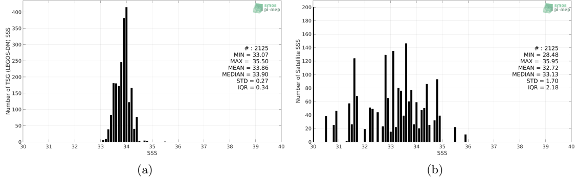
Figure 2: Histograms of SSS from TSG (LEGOS-DM) (a) and Aquarius SSS L2 CAP v5 (JPL) (b) considering all match-up pairs per bins of 0.1 over the Sea of Japan Pi-MEP region and for the full satellite product period.
