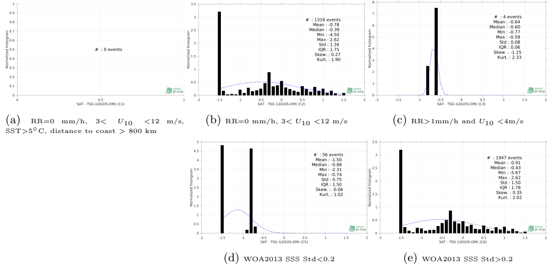
Figure 13: Normalized histogram of \Delta SSS (Aquarius SSS L2 CAP v5 (JPL) - TSG (LEGOS-DM)) for 5 different subdatasets corresponding to: RR=0 mm/h, 3 < U_{10} < 12 m/s, SST > 5^\circ\text{C} , distance to coast > 800 km (a), RR=0 mm/h, 3 < U_{10} < 12 m/s (b), RR > 1 mm/h and U_{10} < 4 m/s (c), WOA2013 SSS Std < 0.2 (d), WOA2013 SSS Std > 0.2 (e).
