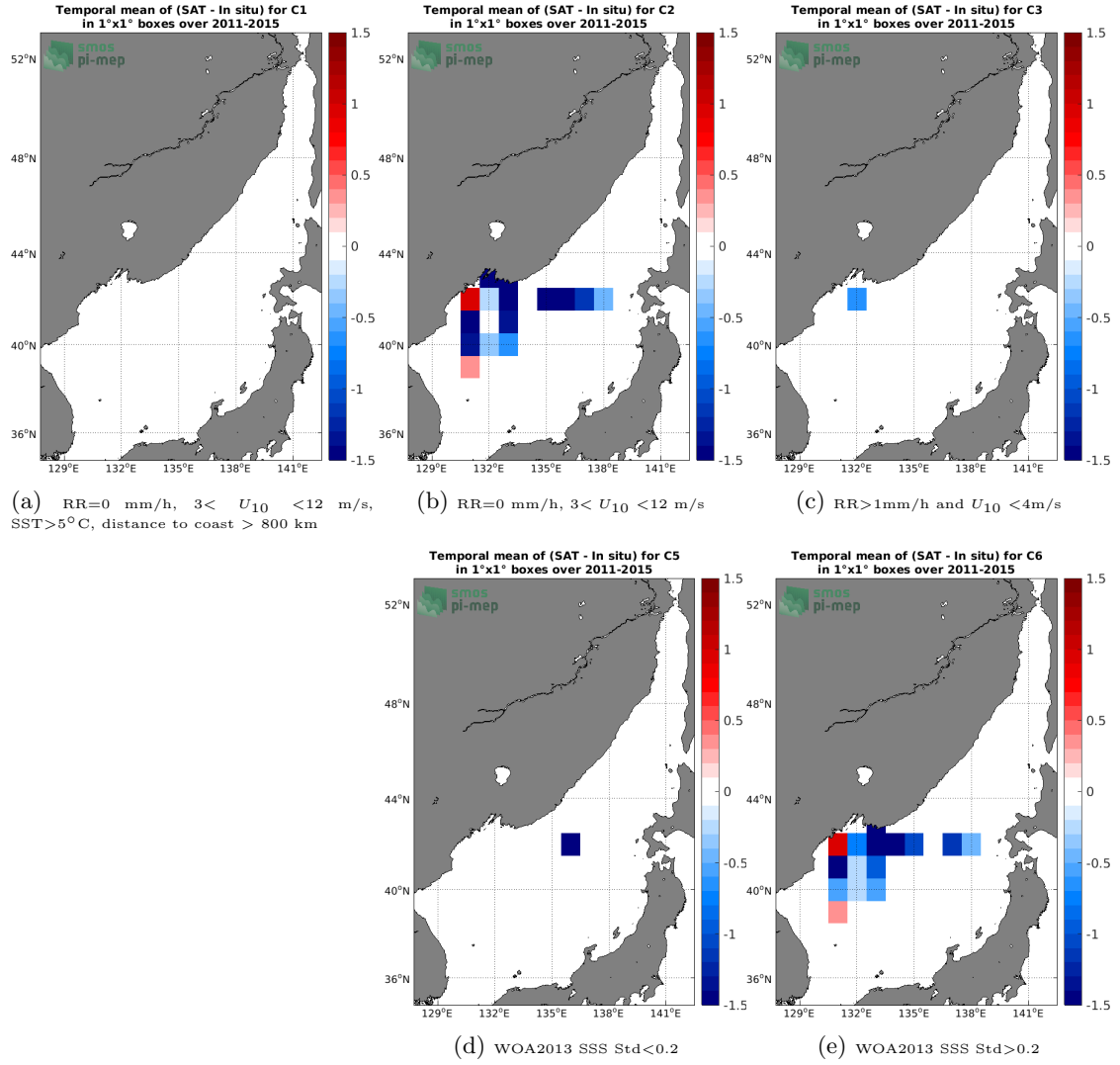
Figure 12: Temporal mean gridded over spatial boxes of size 1°x1° of \Delta SSS (Aquarius SSS L2 CAP v5 (JPL) - TSG (LEGOS-DM)) for 5 different subdatasets corresponding to: RR=0 mm/h, 3 < U_{10} < 12 m/s, SST>5°C, distance to coast > 800 km (a), RR=0 mm/h, 3 < U_{10} < 12 m/s (b), RR>1mm/h and U_{10} < 4 m/s (c), WOA2013 SSS Std<0.2 (d), WOA2013 SSS Std>0.2 (e).
