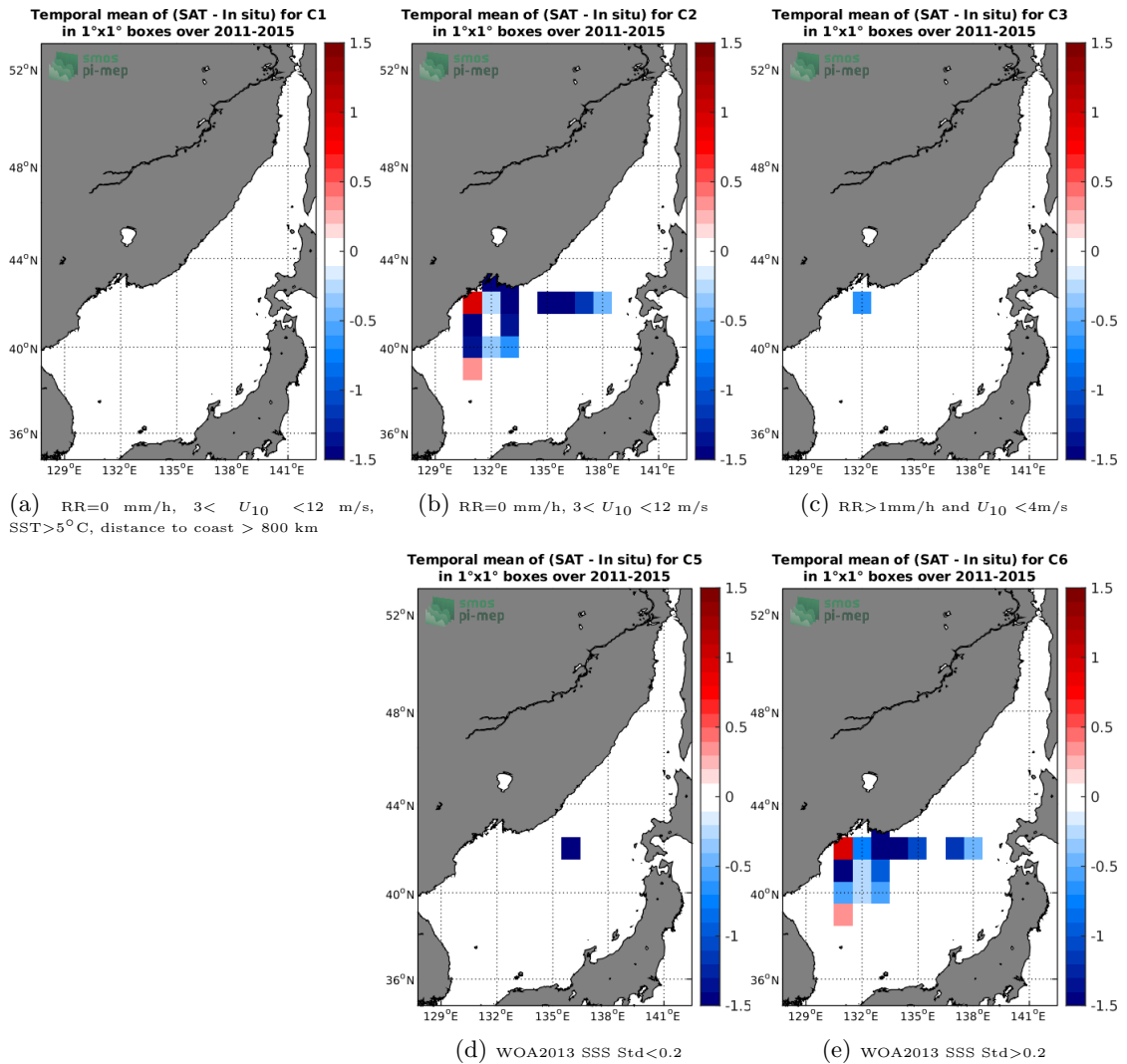
Figure 12: Temporal mean gridded over spatial boxes of size 1^\circ \times 1^\circ of \Delta SSS (Aquarius-L2-JPL-V5 - TSG-LEGOS-DM) for 5 different subdatasets corresponding to:RR=0 mm/h, 3 < U_{10} < 12 m/s, SST>5°C, distance to coast > 800 km (a), RR=0 mm/h, 3 < U_{10} < 12 m/s (b), RR>1mm/h and U_{10} < 4 m/s (c), WOA2013 SSS Std<0.2 (d), WOA2013 SSS Std>0.2 (e).
