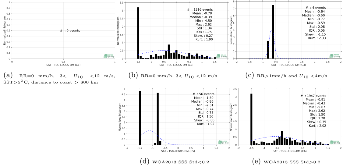
Figure 13: Normalized histogram of \Delta\text{SSS} (Aquarius-L2-JPL-V5 - TSG-LEGOS-DM) for 5 different subdatasets corresponding to: RR=0 mm/h, 3 < U_{10} < 12 m/s, SST > 5^{\circ}\text{C} , distance to coast > 800 km (a), RR=0 mm/h, 3 < U_{10} < 12 m/s (b), RR > 1\text{mm/h} and U_{10} < 4\text{m/s} (c), WOA2013 SSS Std < 0.2 (d), WOA2013 SSS Std > 0.2 (e).
