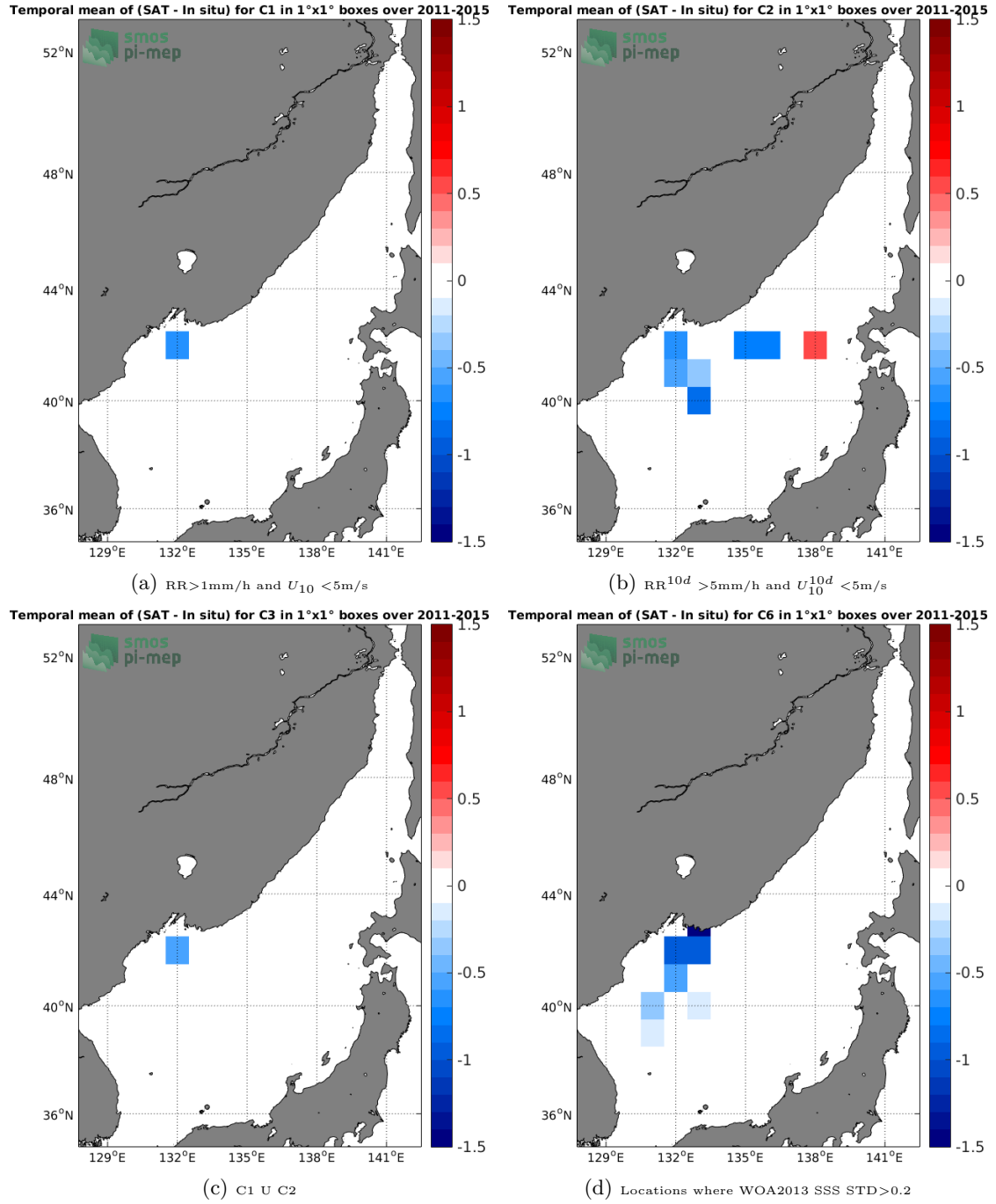
Figure 12: Temporal mean gridded over spatial boxes of size 1°x1° of \Delta\text{SSS} (Aquarius-L2-JPL-V5 - TSG-LEGOS-DM) for 4 different subdatasets corresponding to: RR > 1\text{mm/h} and U_{10} < 5\text{m/s} (a), RR^{10d} > 5\text{mm/h} and U_{10}^{10d} < 5\text{m/s} (b), C1 U C2 (c), Locations where WOA2013 SSS STD > 0.2 (d).
