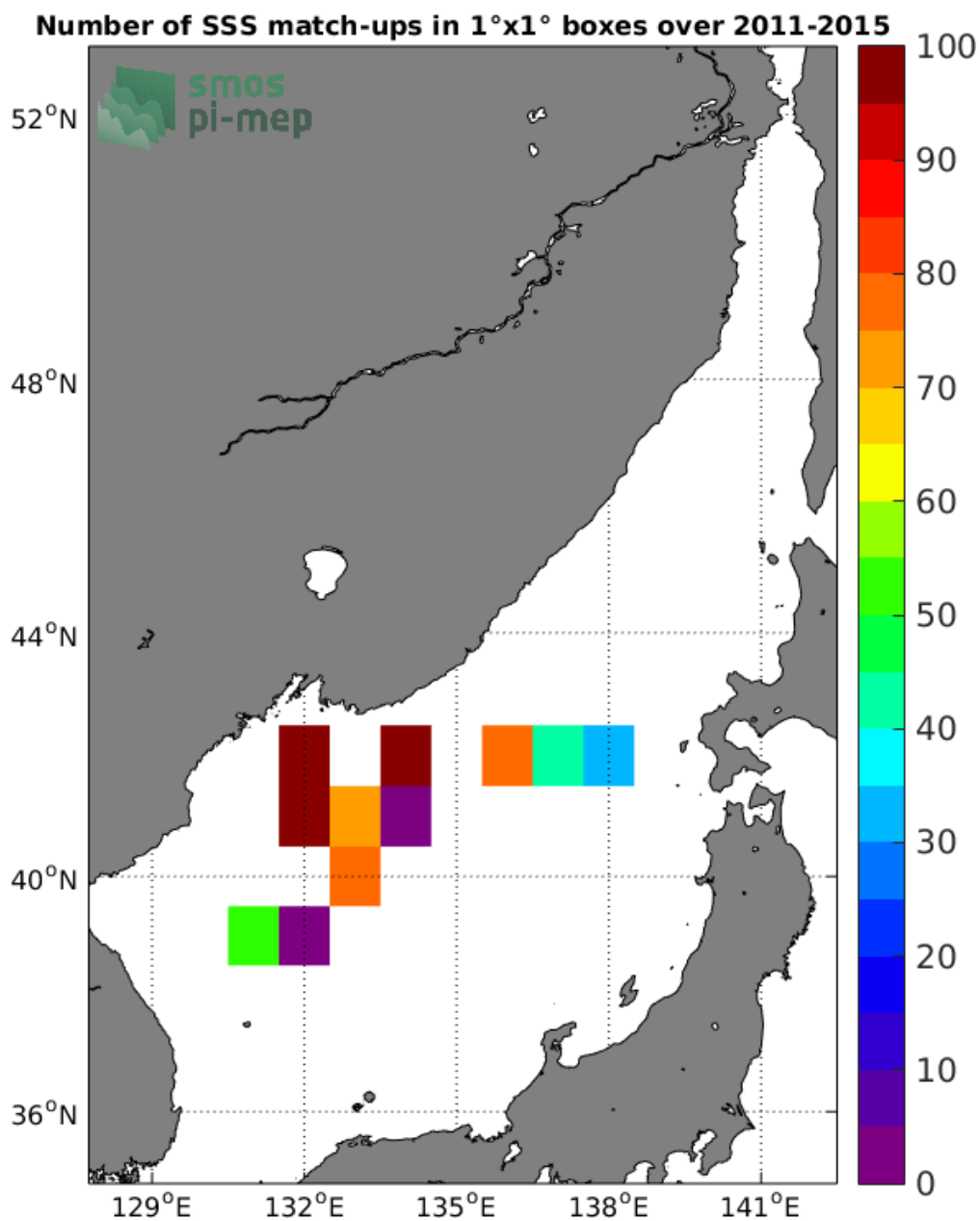
Figure 4: Number of SSS match-ups between TSG-LEGOS-DM SSS and the Aquarius-L2-JPL-V5 SSS product for the Sea of Japan Pi-MEP region over 1°x1° boxes and for the full satellite product period.
