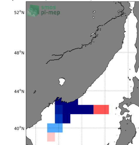
Temporal mean of (Sat-TSG-LEGOS-DM) in 1°x1° boxes over 2011-2015
