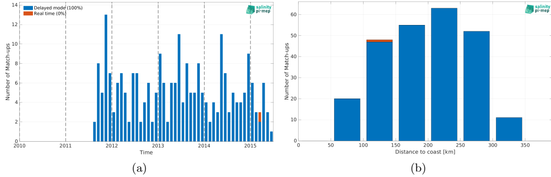
Figure 2: Number of match-ups between Argo and Aquarius SSS L2 CAP v5 (JPL) SSS as a function of time (a) and as function of the distance to coast (b) over the Sea of Japan Pi-MEP region and for the full satellite product period.
