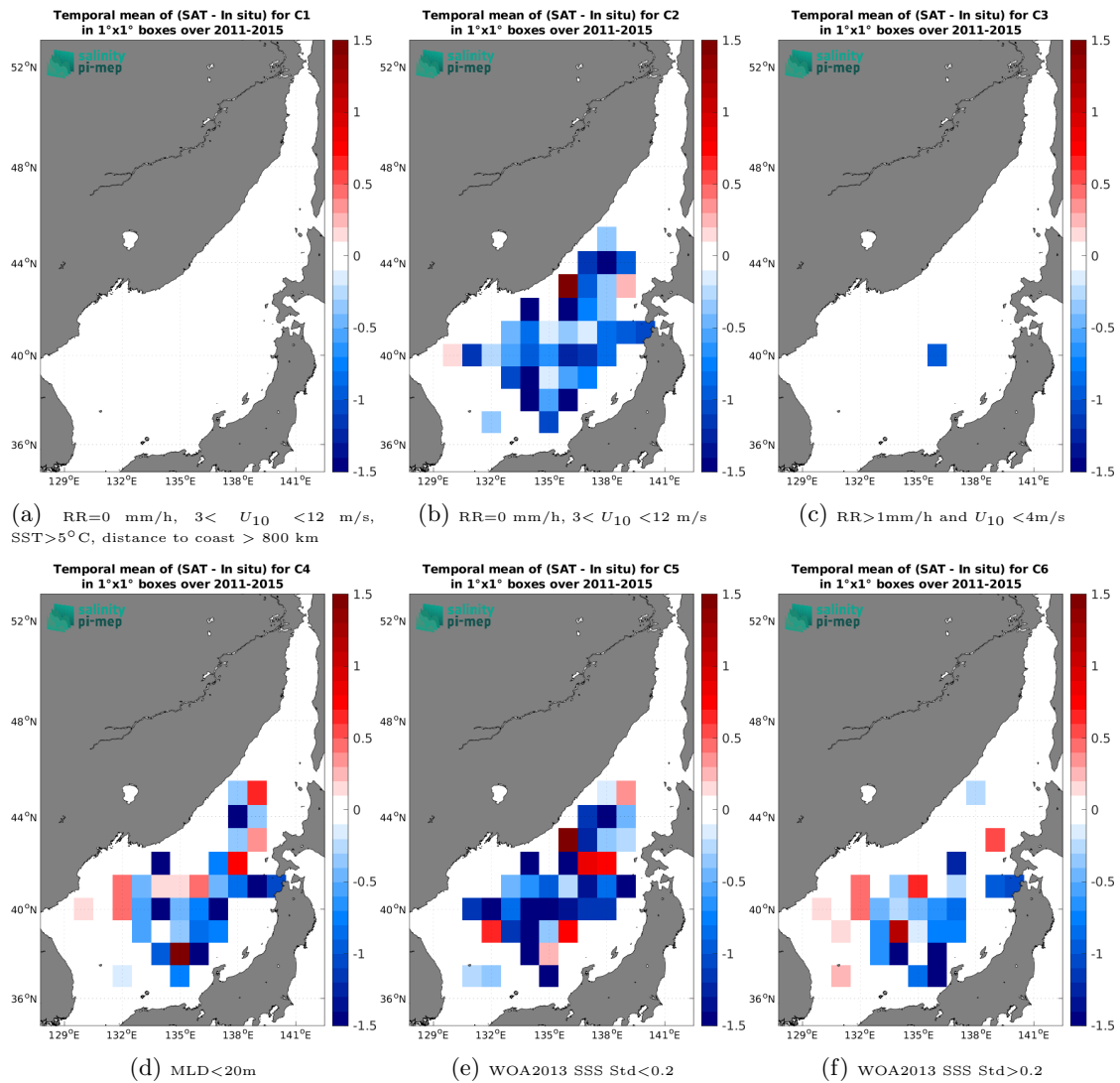
Figure 14: Temporal mean gridded over spatial boxes of size 1^\circ \times 1^\circ of \Delta SSS (Aquarius SSS L2 CAP v5 (JPL) - Argo) for 6 different subdatasets corresponding to: RR=0 mm/h, 3 < U_{10} < 12 m/s, SST > 5°C, distance to coast > 800 km (a), RR=0 mm/h, 3 < U_{10} < 12 m/s (b), RR > 1mm/h and U_{10} < 4 m/s (c), MLD < 20m (d), WOA2013 SSS Std < 0.2 (e), WOA2013 SSS Std > 0.2 (f).
