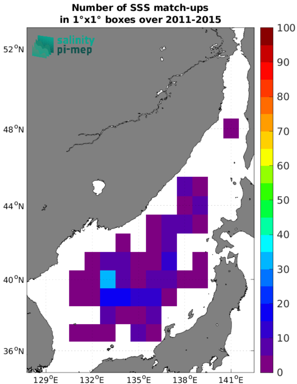
Figure 5: Number of SSS match-ups between Argo SSS and the Aquarius SSS L2 CAP v5 (JPL) SSS product for the Sea of Japan Pi-MEP region over 1°x1° boxes and for the full satellite product period.
