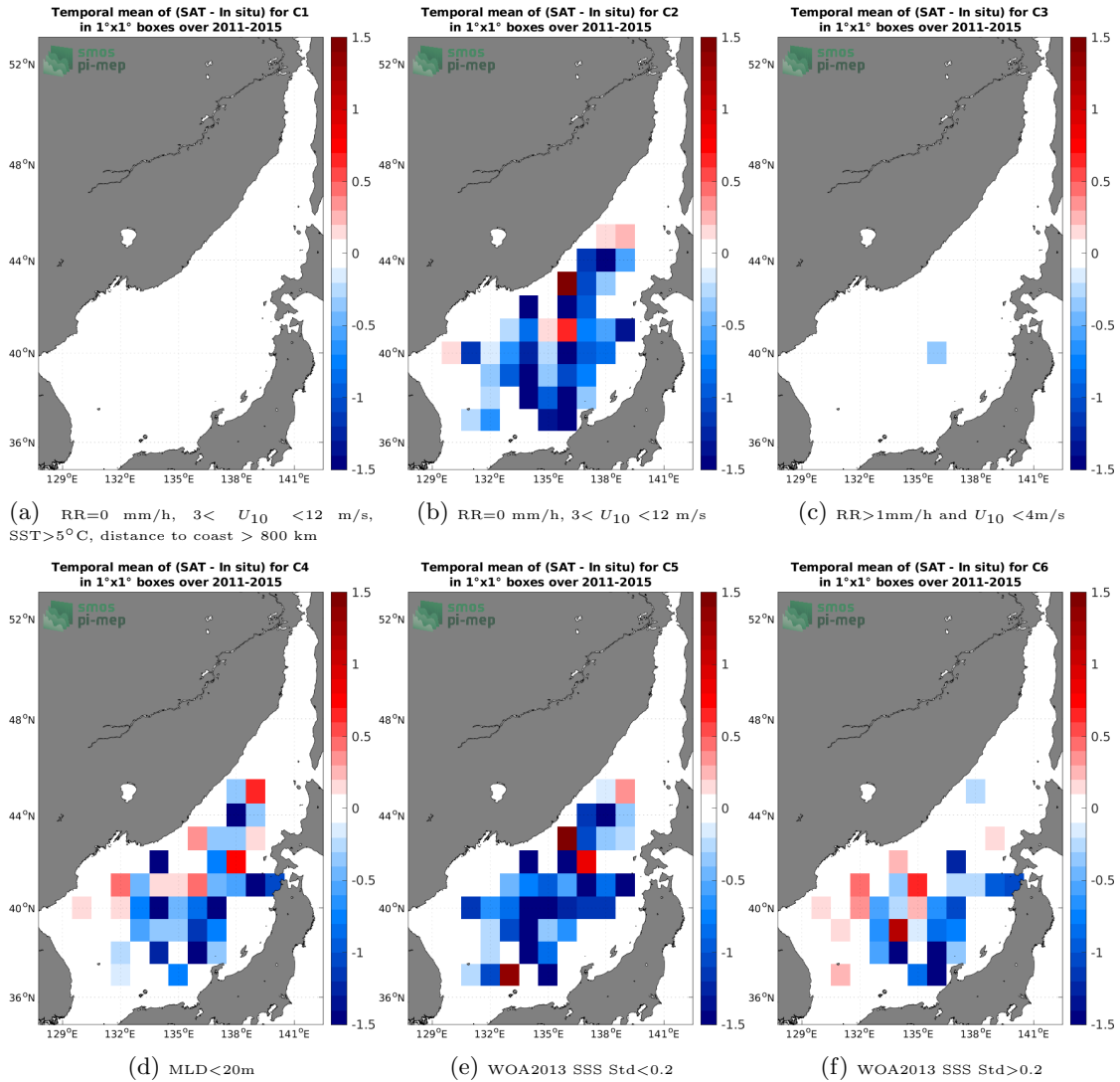
Figure 12: Temporal mean gridded over spatial boxes of size 1^\circ \times 1^\circ of \Delta\text{SSS} (Aquarius SSS L2 CAP v5 (JPL) - Argo) for 6 different subdatasets corresponding to: RR=0 mm/h, 3 < U_{10} < 12 m/s, SST > 5^\circ\text{C} , distance to coast > 800 km (a), RR=0 mm/h, 3 < U_{10} < 12 m/s (b), RR > 1 mm/h and U_{10} < 4 m/s (c), MLD < 20 m (d), WOA2013 SSS Std < 0.2 (e), WOA2013 SSS Std > 0.2 (f).
