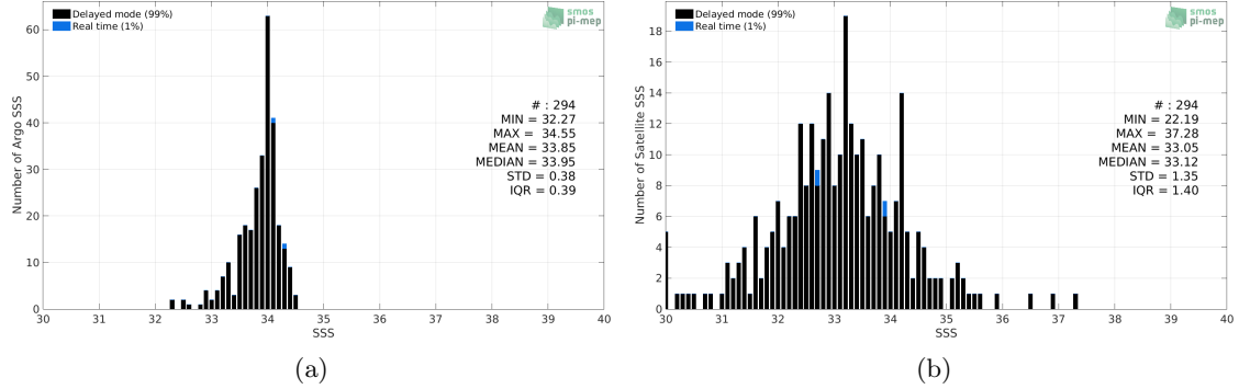
Figure 2: Histograms of SSS from Argo (a) and Aquarius SSS L2 CAP v5 (JPL) (b) considering all match-up pairs per bins of 0.1 over the Sea of Japan Pi-MEP region and for the full satellite product period.
