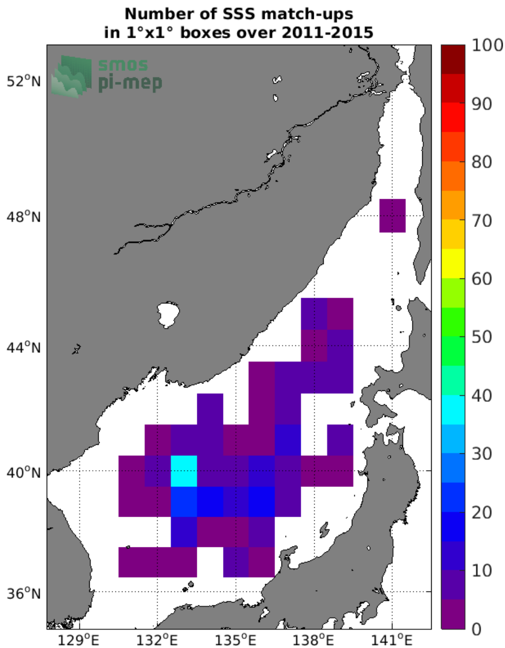
Figure 4: Number of SSS match-ups between Argo SSS and the Aquarius SSS L2 CAP v5 (JPL) SSS product for the Sea of Japan Pi-MEP region over 1°x1° boxes and for the full satellite product period.
