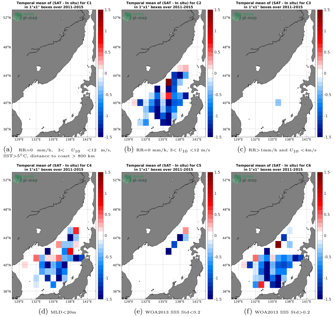
Figure 12: Temporal mean gridded over spatial boxes of size 1^\circ \times 1^\circ of \Delta SSS (Aquarius SSS L2 CAP v5 (JPL) - Argo) for 6 different subdatasets corresponding to: RR=0 mm/h, 3 < U_{10} < 12 m/s, SST > 5^\circ\text{C} , distance to coast > 800 km (a), RR=0 mm/h, 3 < U_{10} < 12 m/s (b), RR > 1 mm/h and U_{10} < 4 m/s (c), MLD < 20\text{m} (d), WOA2013 SSS Std < 0.2 (e), WOA2013 SSS Std > 0.2 (f).
