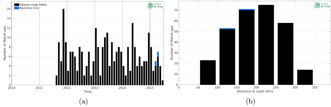
Figure 1: Number of match-ups between Argo and Aquarius SSS L2 CAP v5 (JPL) SSS as a function of time (a) and as function of the distance to coast (b) over the Sea of Japan Pi-MEP region and for the full satellite product period.
