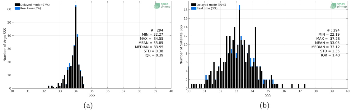
Figure 2: Histograms of SSS from Argo (a) and Aquarius-L2-JPL-V5 (b) considering all match-up pairs per bins of 0.1 over the Sea of Japan Pi-MEP region and for the full satellite product period.
