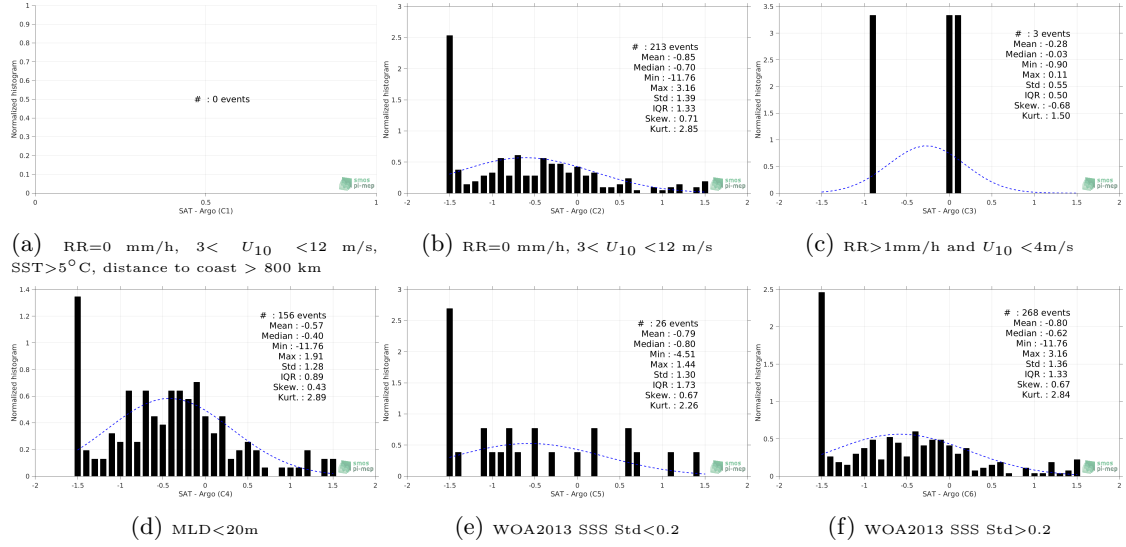
Figure 13: Normalized histogram of \Delta\text{SSS} (Aquarius-L2-JPL-V5 - Argo) for 6 different sub-datasets corresponding to: RR=0 mm/h, 3 < U_{10} < 12 m/s, SST > 5^\circ\text{C} , distance to coast > 800 km (a), RR=0 mm/h, 3 < U_{10} < 12 m/s (b), RR > 1\text{mm/h} and U_{10} < 4\text{m/s} (c), MLD < 20\text{m} (d), WOA2013 SSS Std < 0.2 (e), WOA2013 SSS Std > 0.2 (f).
