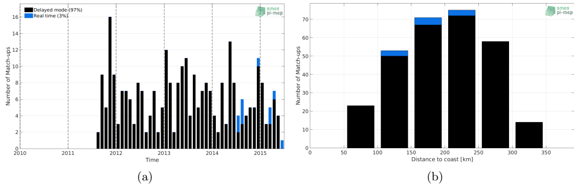
Figure 1: Number of match-ups between Argo and Aquarius-L2-JPL-V5 SSS as a function of time (a) and as function of the distance to coast (b) over the Sea of Japan Pi-MEP region and for the full satellite product period.
