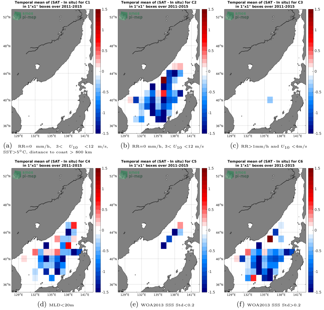
Figure 12: Temporal mean gridded over spatial boxes of size 1^\circ \times 1^\circ of \Delta\text{SSS} (Aquarius-L2-JPL-V5 - Argo) for 6 different subdatasets corresponding to: RR=0 mm/h, 3 < U_{10} < 12 m/s, SST > 5^\circ\text{C} , distance to coast > 800 km (a), RR=0 mm/h, 3 < U_{10} < 12 m/s (b), RR > 1 mm/h and U_{10} < 4 m/s (c), MLD < 20\text{m} (d), WOA2013 SSS Std < 0.2 (e), WOA2013 SSS Std > 0.2 (f).
