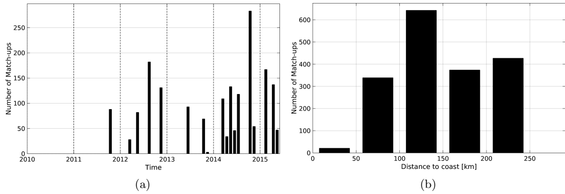
Figure 1: Number of match-ups between TSG-LEGOS-DM and AQUARIUS-L2-JPL-V4 SSS as a function of time (a) and as function of the distance to coast (b) over the Sea of Japan Pi-MEP region and for the full satellite product period.
