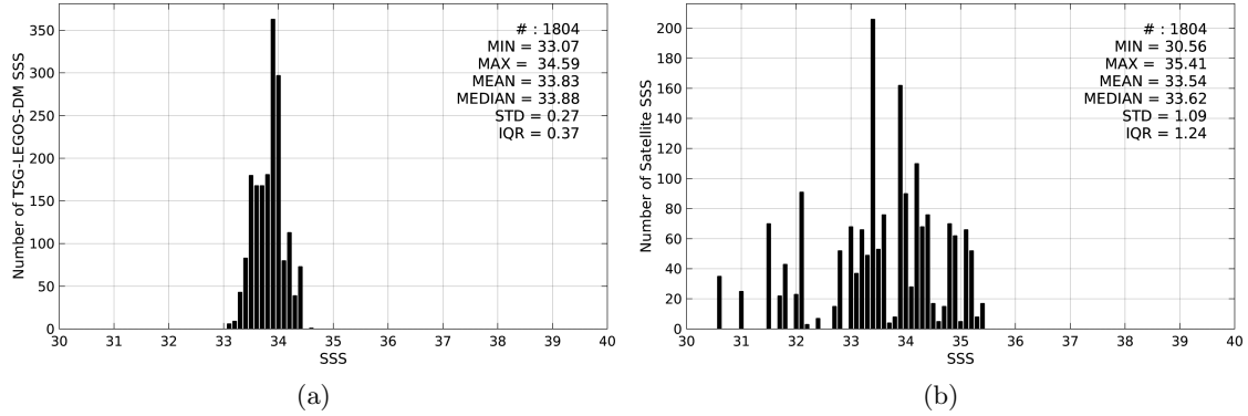
Figure 2: Histograms of SSS from TSG-LEGOS-DM (a) and AQUARIUS-L2-JPL-V4 (b) considering all match-up pairs per bins of 0.1 over the Sea of Japan Pi-MEP region and for the full satellite product period.
