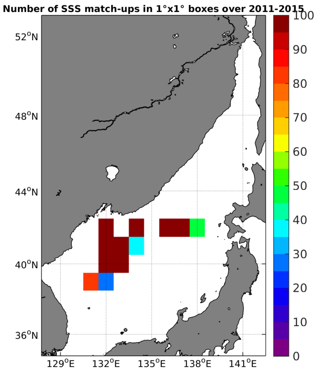
Figure 4: Number of SSS match-ups between TSG-LEGOS-DM SSS and the AQUARIUS-L2-JPL-V4 SSS product for the Sea of Japan Pi-MEP region over 1°x1° boxes and for the full satellite product period.
