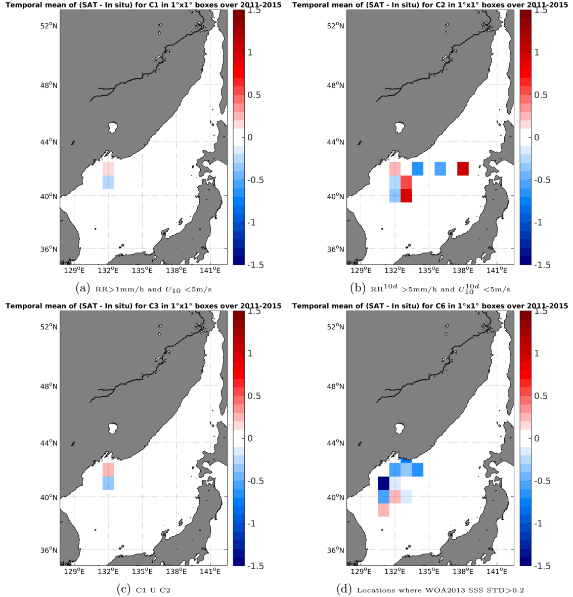
Figure 12: Temporal mean gridded over spatial boxes of size 1^\circ \times 1^\circ of \Delta SSS (AQUARIUS-L2-JPL-V4 - TSG-LEGOS-DM) for 4 different subdatasets corresponding to: RR > 1mm/h and U_{10} < 5 m/s (a), RR 10d > 5mm/h and U_{10}^{10d} < 5 m/s (b), C1 U C2 (c), Locations where WOA2013 SSS STD > 0.2 (d).
