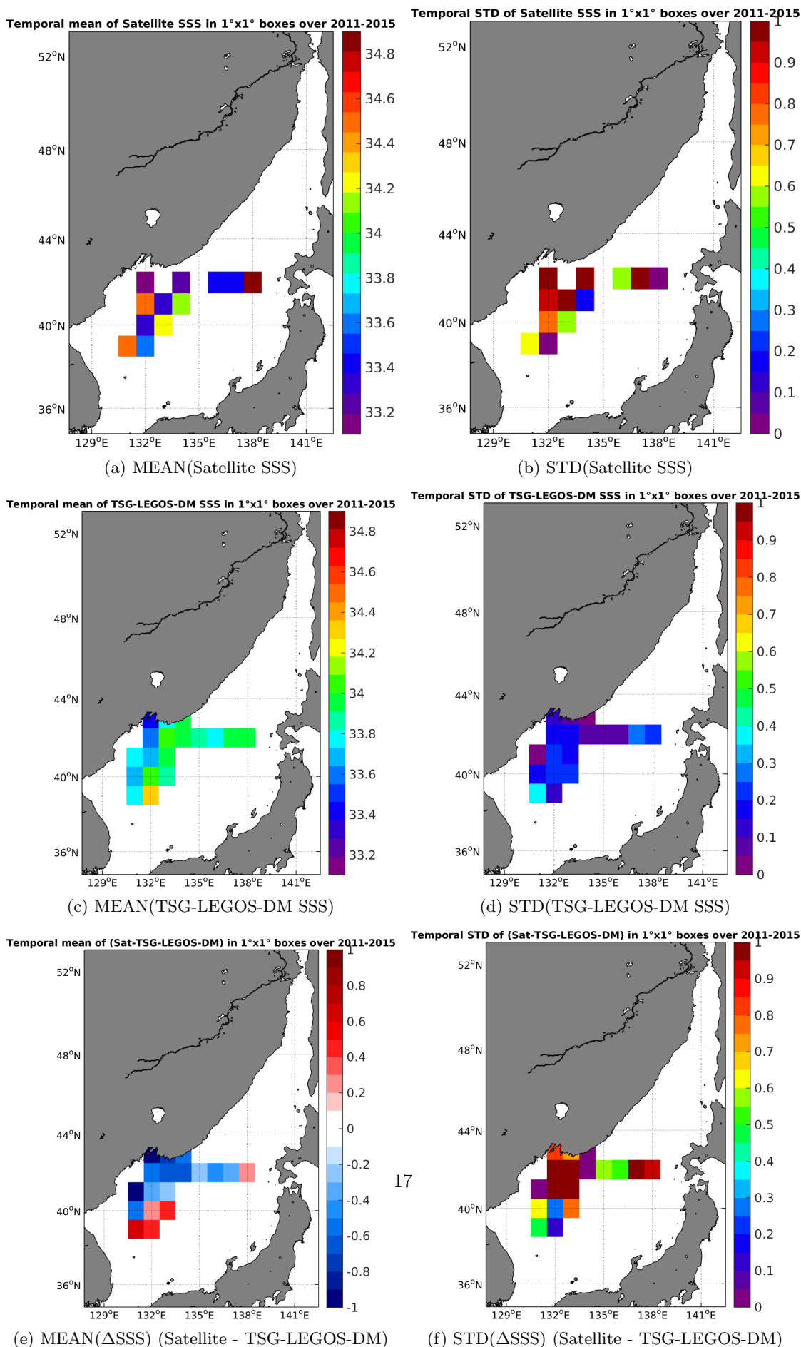
Figure 6: Temporal mean (left) and STD (right) of SSS from AQUARIUS-L2-JPL-V4 (top), TSG-LEGOS-DM (middle), and of \Delta SSS (Satellite - TSG-LEGOS-DM). Only match-up pairs are used to generate these maps.
