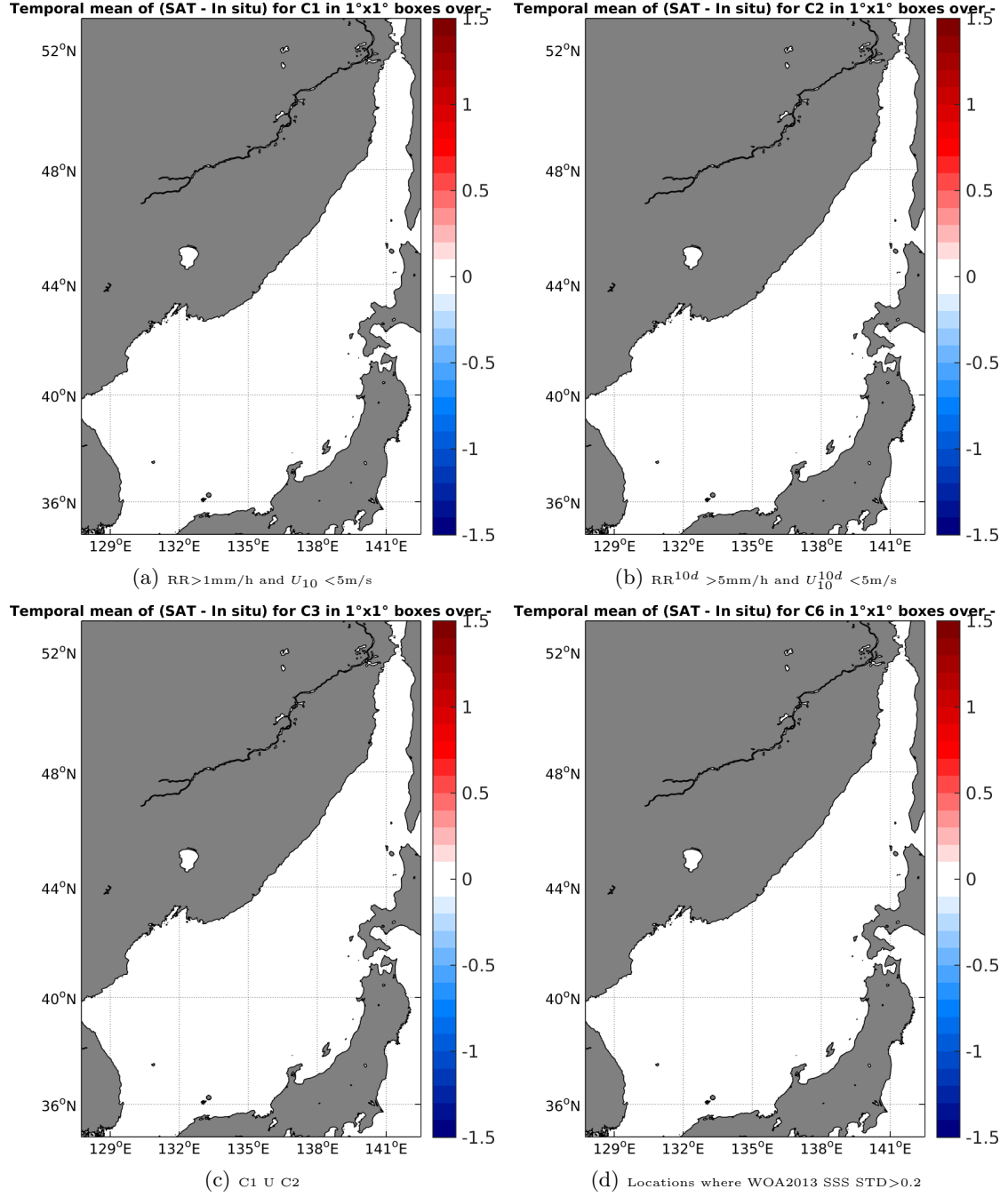
Figure 12: Temporal mean gridded over spatial boxes of size 1^\circ \times 1^\circ of \Delta\text{SSS} (AQUARIUS-L2-JPL-V4 - TSG-GOSUD-Sailing-ship) for 4 different subdatasets corresponding to: RR > 1\text{mm/h} and U_{10} < 5\text{m/s} (a), RR^{10d} > 5\text{mm/h} and U_{10}^{10d} < 5\text{m/s} (b), C1 U C2 (c), Locations where WOA2013 SSS STD > 0.2 (d).
