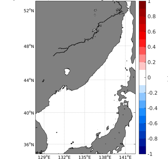
(e) MEAN(ΔSSS) (Satellite - TSG-GOSUD-Sailing-ship)
