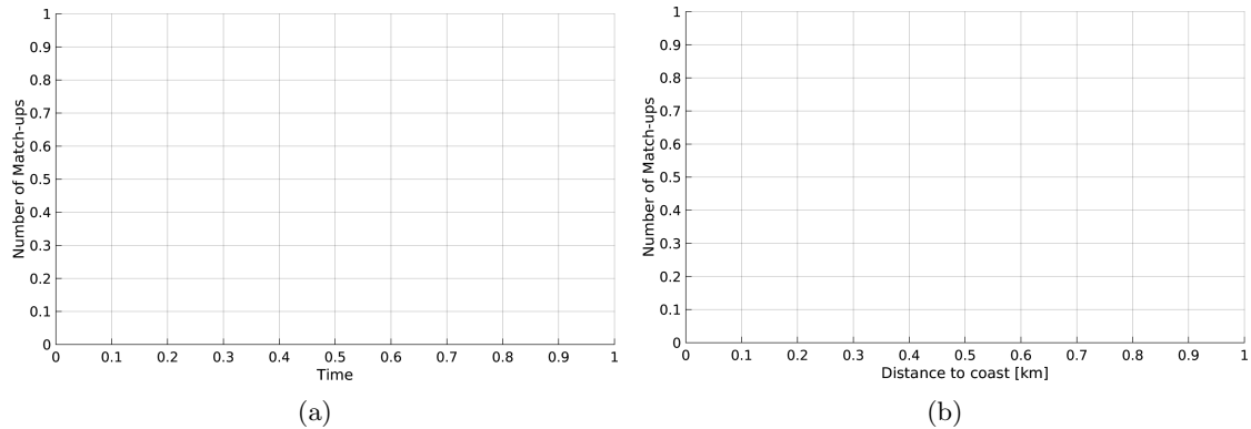
Figure 1: Number of match-ups between Sea mammals and AQUARIUS-L2-JPL-V4 SSS as a function of time (a) and as function of the distance to coast (b) over the Sea of Japan Pi-MEP region and for the full satellite product period.
