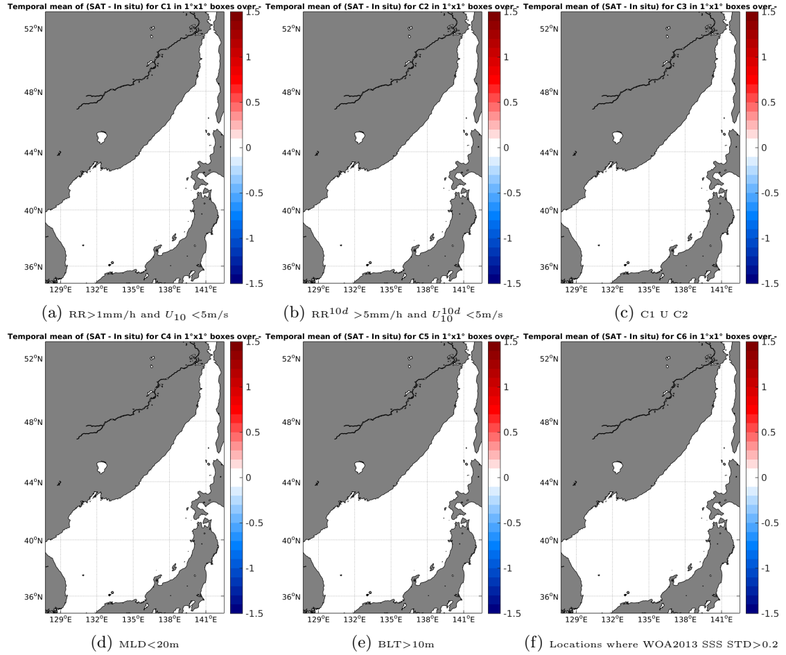
Figure 12: Temporal mean gridded over spatial boxes of size 1^\circ \times 1^\circ of \Delta SSS (AQUARIUS-L2-JPL-V4 - Sea mammals) for 6 different subdatasets corresponding to: RR > 1mm/h and U_{10} < 5\text{m/s} (a), RR^{10d} > 5\text{mm/h} and U_{10}^{10d} < 5\text{m/s} (b), C1 U C2 (c), MLD < 20m (d), BLT > 10m (e), Locations where WOA2013 SSS STD > 0.2 (f).
