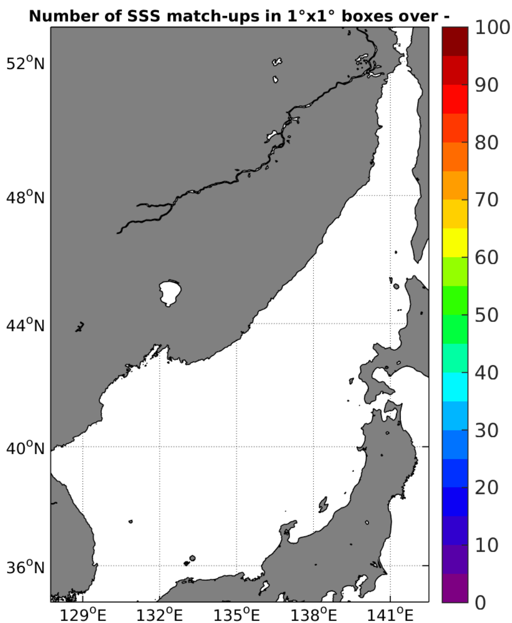
Figure 4: Number of SSS match-ups between Sea mammals SSS and the AQUARIUS-L2-JPL-V4 SSS product for the Sea of Japan Pi-MEP region over 1°x1° boxes and for the full satellite product period.
