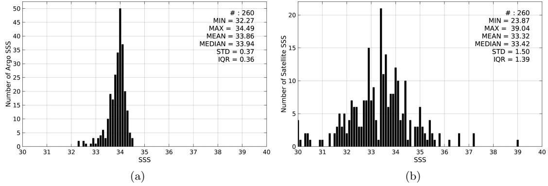
Figure 2: Histograms of SSS from Argo (a) and AQUARIUS-L2-JPL-V4 (b) considering all match-up pairs per bins of 0.1 over the Sea of Japan Pi-MEP region and for the full satellite product period.
