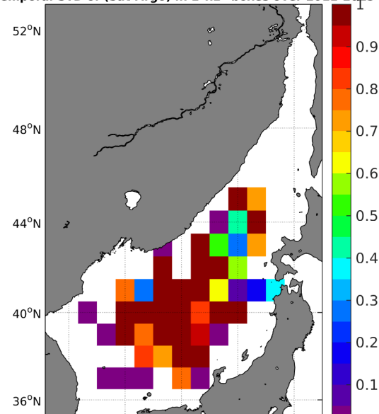
Temporal STD of (Sat-Argo) in 1^\circ \times 1^\circ boxes over 2011-2015
