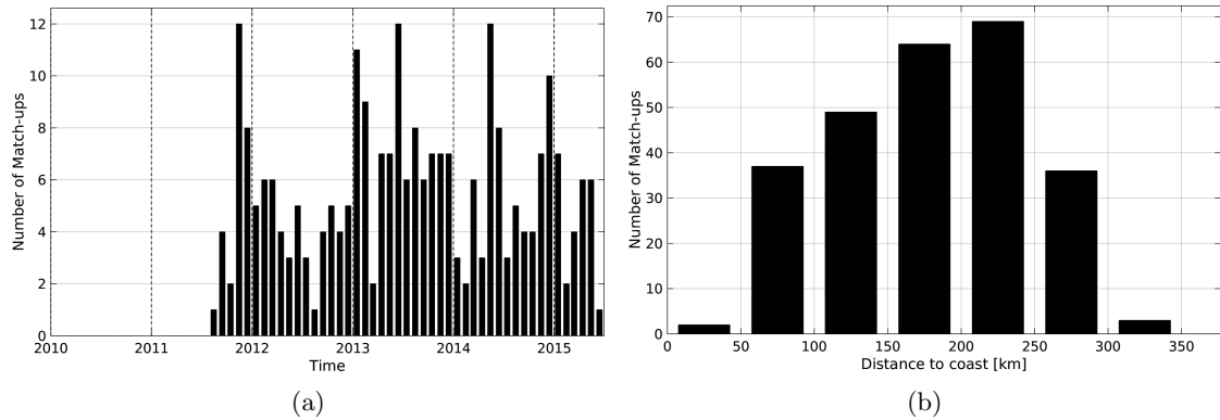
Figure 1: Number of match-ups between Argo and AQUARIUS-L2-JPL-V4 SSS as a function of time (a) and as function of the distance to coast (b) over the Sea of Japan Pi-MEP region and for the full satellite product period.
