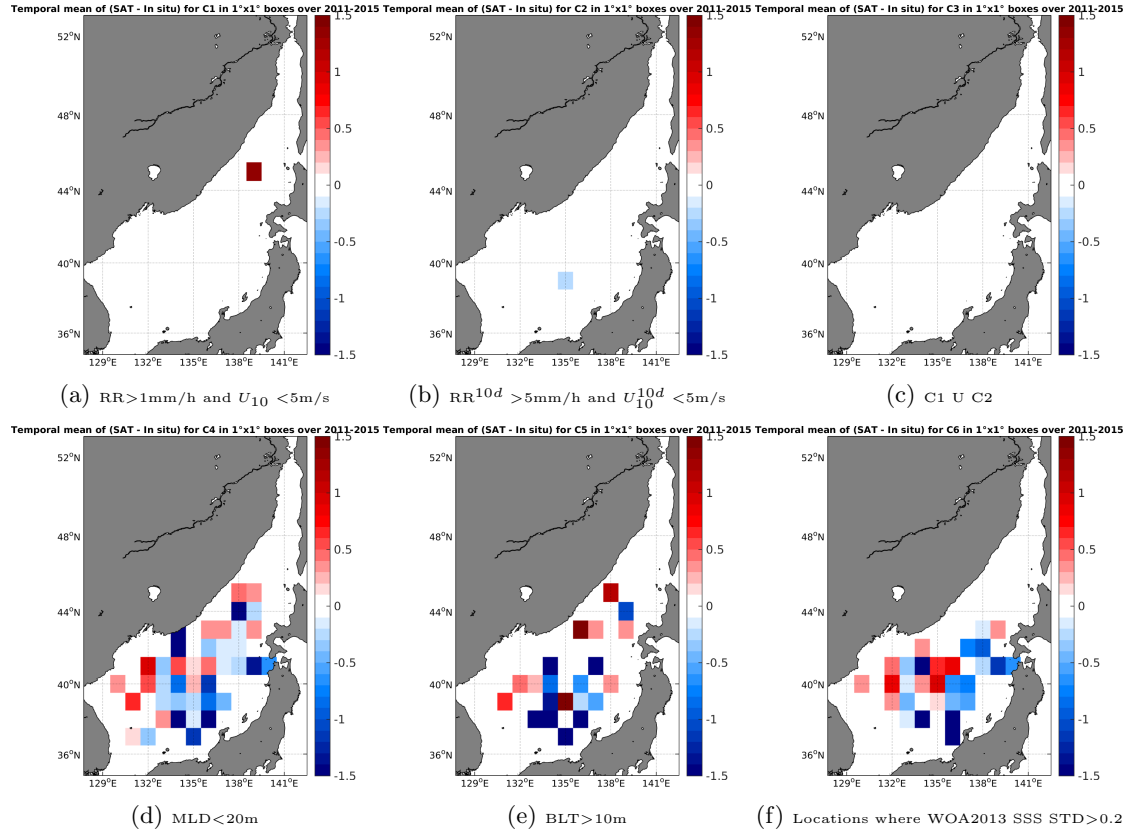
Figure 12: Temporal mean gridded over spatial boxes of size 1^\circ \times 1^\circ of \Delta\text{SSS} (AQUARIUS-L2-JPL-V4 - Argo) for 6 different subdatasets corresponding to: \text{RR} > 1\text{mm/h} and U_{10} < 5\text{m/s} (a), \text{RR}^{10d} > 5\text{mm/h} and U_{10}^{10d} < 5\text{m/s} (b), C1 U C2 (c), \text{MLD} < 20\text{m} (d), \text{BLT} > 10\text{m} (e), Locations where WOA2013 SSS STD > 0.2 (f).
