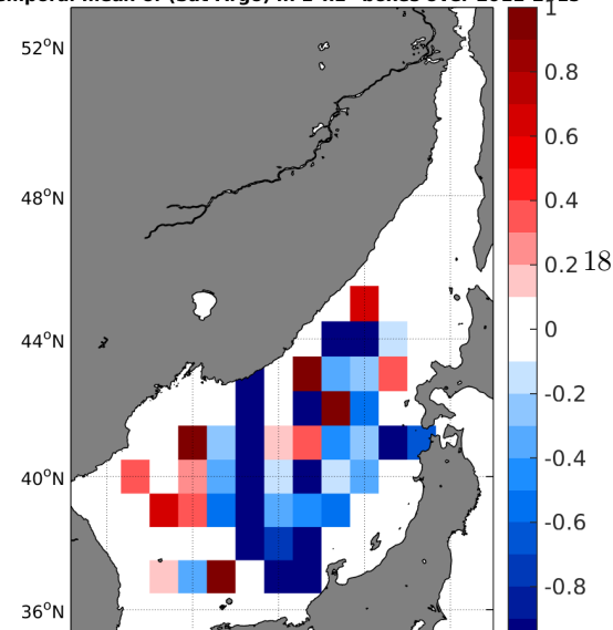
Temporal mean of (Sat-Argo) in 1^\circ \times 1^\circ boxes over 2011-2015
