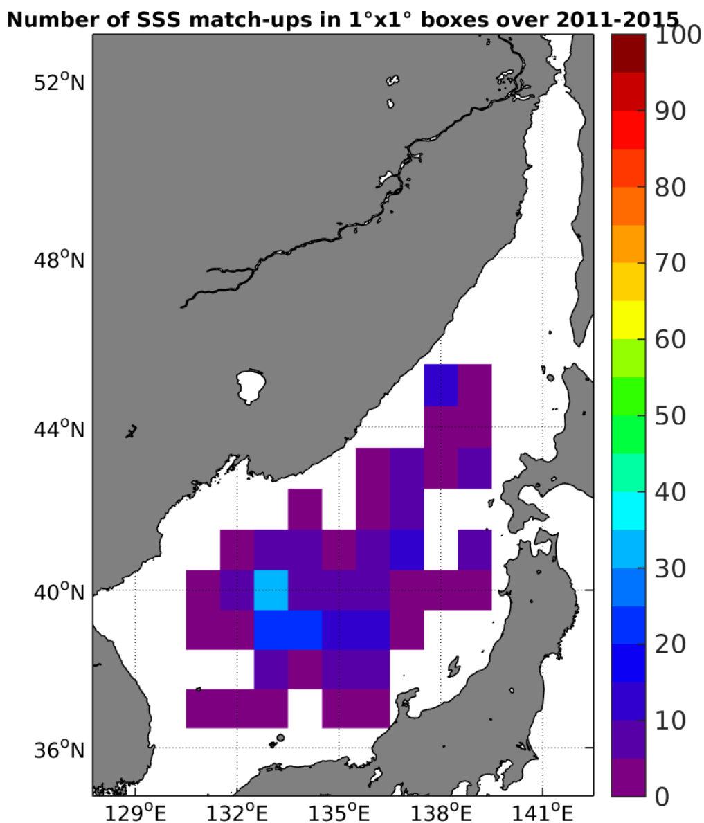
Figure 4: Number of SSS match-ups between Argo SSS and the AQUARIUS-L2-JPL-V4 SSS product for the Sea of Japan Pi-MEP region over 1°x1° boxes and for the full satellite product period.
