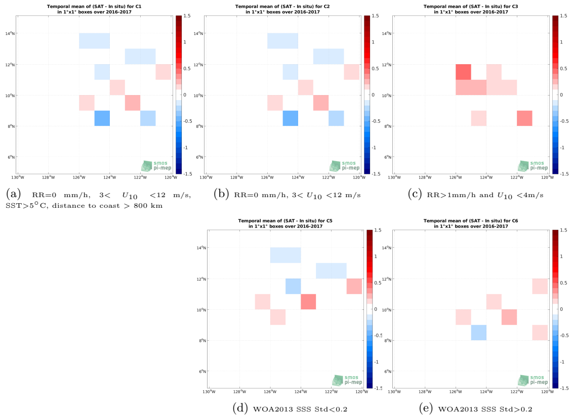
Figure 12: Temporal mean gridded over spatial boxes of size 1^\circ \times 1^\circ of \Delta SSS (SMOS and SMAP SSS L4 OI v1 - 7 Days (LOPS) - Waveglider (SPURS 2)) for 5 different subdatasets corresponding to:RR=0 mm/h, 3 < U_{10} < 12 m/s, SST >5^\circ C, distance to coast > 800 km (a), RR=0 mm/h, 3 < U_{10} < 12 m/s (b), RR >1 mm/h and U_{10} < 4 m/s (c), WOA2013 SSS Std <0.2 (d), WOA2013 SSS Std >0.2 (e).
