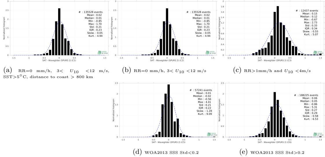
Figure 13: Normalized histogram of \Delta SSS (SMOS and SMAP SSS L4 OI v1 - 7 Days (LOPS) - Waveglider (SPURS 2)) for 5 different subdatasets corresponding to: RR=0 mm/h, 3 < U_{10} < 12 m/s, SST > 5°C, distance to coast > 800 km (a), RR=0 mm/h, 3 < U_{10} < 12 m/s (b), RR > 1mm/h and U_{10} < 4 m/s (c), WOA2013 SSS Std < 0.2 (d), WOA2013 SSS Std > 0.2 (e).
