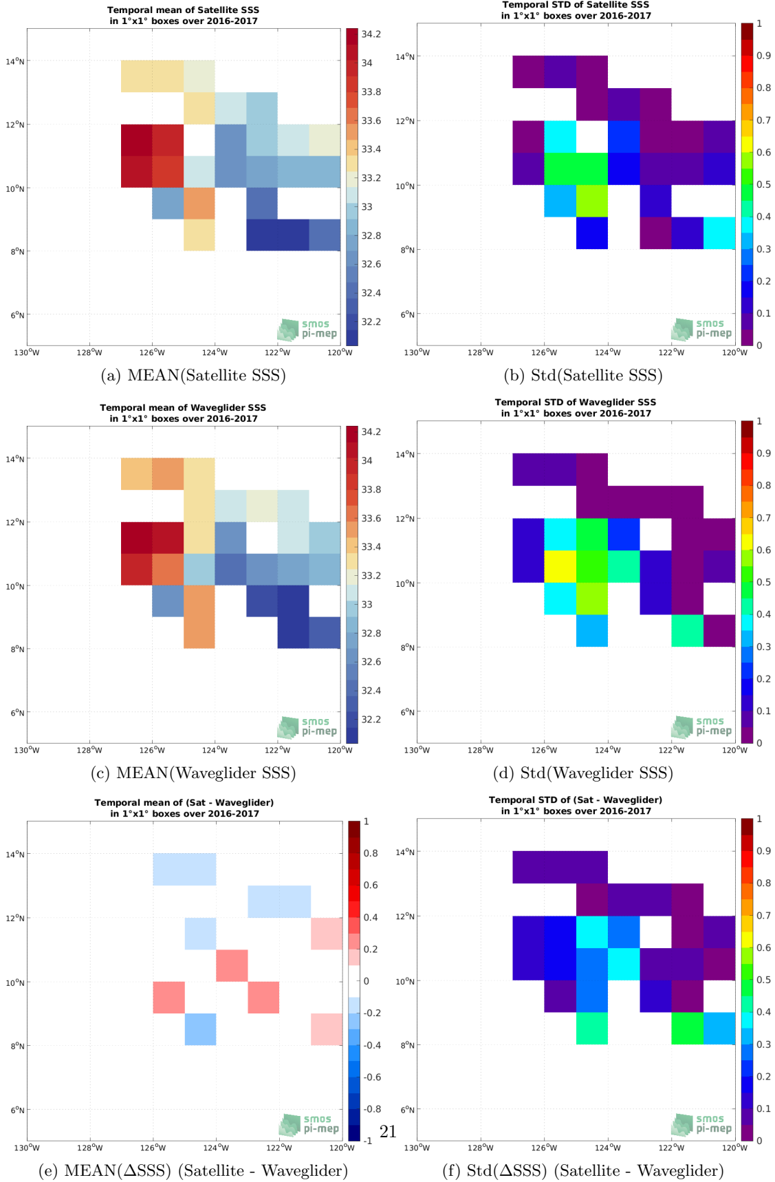
Figure 5: Temporal mean (left) and Std (right) of SSS from SMOS and SMAP SSS L4 OI v1 - 7 Days (LOPS) (top), Waveglider (middle), and of \Delta SSS (Satellite - Waveglider). Only match-up pairs are used to generate these maps.
