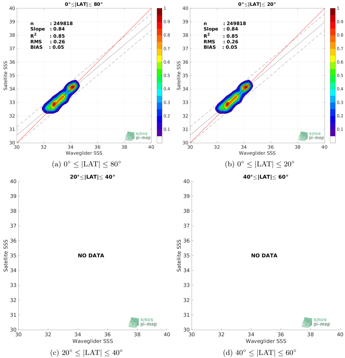
Figure 8: Contour maps of the concentration of SMOS and SMAP SSS L4 OI v1 - 7 Days (LOPS) SSS (y-axis) versus Waveglider SSS (x-axis) at match-up pairs for different latitude bands. For each plot, the red line shows x=y . The black thin and dashed lines indicate a linear fit through the data cloud and the \pm 95\% confidence levels, respectively. The number match-up pairs n , the slope and R^2 coefficient of the linear fit, the root mean square (RMS) and the mean bias between satellite and in situ data are indicated for each latitude band in each plots.
