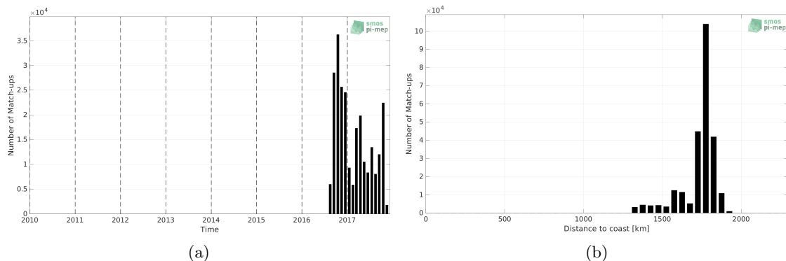
Figure 1: Number of match-ups between Waveglider and SMOS and SMAP SSS L4 OI v1 - 7 Days (LOPS) SSS as a function of time (a) and as function of the distance to coast (b) over the SPURS 2 Pi-MEP region and for the full satellite product period.
