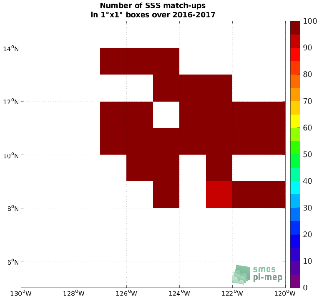
Figure 3: Number of SSS match-ups between Waveglider SSS and the SMOS and SMAP SSS L4 OI v1 - 7 Days (LOPS) SSS product for the SPURS 2 Pi-MEP region over 1°x1° boxes and for the full satellite product period.
