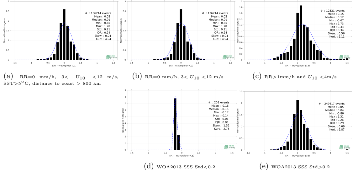
Figure 12: Normalized histogram of \Delta SSS (SMOS and SMAP SSS L4 OI v1 - 7 Days (LOPS) - Waveglider) for 5 different subdatasets corresponding to: RR=0 mm/h, 3 < U_{10} < 12 m/s, SST>5°C, distance to coast > 800 km (a), RR=0 mm/h, 3 < U_{10} < 12 m/s (b), RR>1mm/h and U_{10} < 4 m/s (c), WOA2013 SSS Std<0.2 (d), WOA2013 SSS Std>0.2 (e).
