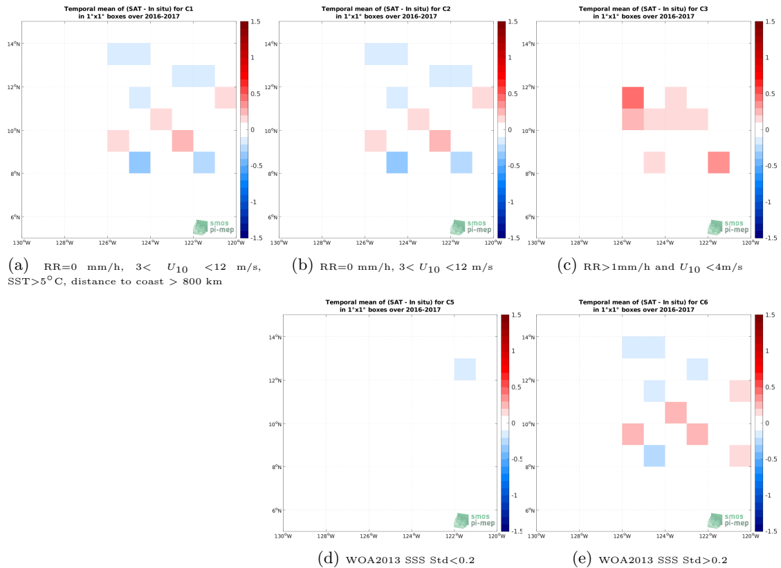
Figure 11: Temporal mean gridded over spatial boxes of size 1^\circ \times 1^\circ of \Delta\text{SSS} (SMOS and SMAP SSS L4 OI v1 - 7 Days (LOPS) - Waveglider) for 5 different subdatasets corresponding to:RR=0 mm/h, 3 < U_{10} < 12 m/s, SST >5^\circ\text{C} , distance to coast > 800 km (a), RR=0 mm/h, 3 < U_{10} < 12 m/s (b), RR >1 mm/h and U_{10} < 4 m/s (c), WOA2013 SSS Std <0.2 (d), WOA2013 SSS Std >0.2 (e).
