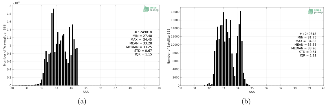
Figure 2: Histograms of SSS from Waveglider (a) and SMOS and SMAP SSS L4 OI v1 - 7 Days (LOPS) (b) considering all match-up pairs per bins of 0.1 over the SPURS 2 Pi-MEP region and for the full satellite product period.
