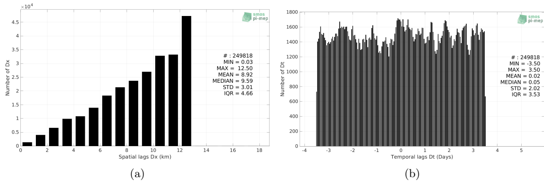
Figure 4: Histograms of the spatial (a) and temporal (b) lags between the location/time of the Waveglider measurement and the date of the corresponding SMOS and SMAP SSS L4 OI v1 - 7 Days (LOPS) SSS pixel.
