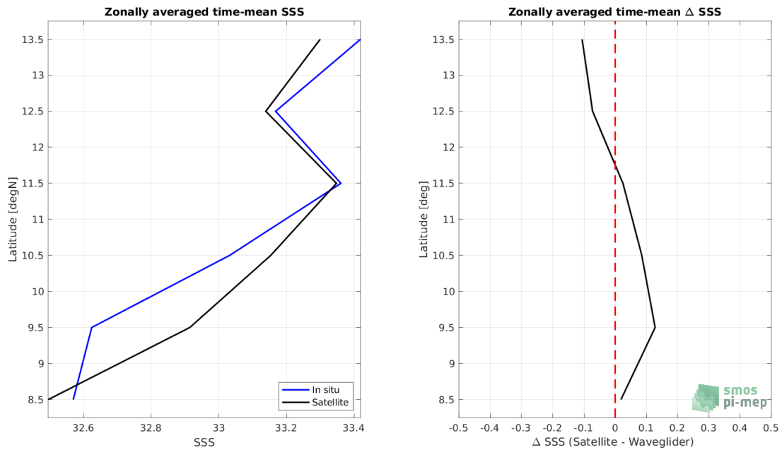
Figure 7: Left panel: Zonal mean SSS from SMOS and SMAP SSS L4 OI v1 - 7 Days (LOPS) satellite product (black) and from Waveglider (blue). Right panel: Zonal mean of \Delta SSS (Satellite - Waveglider) for all the collected Pi-MEP match-up pairs estimated over the full satellite product period.
