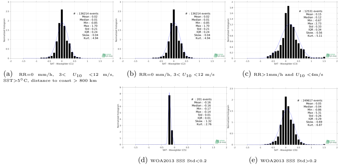
Figure 13: Normalized histogram of \Delta SSS (SMOS and SMAP SSS L4 OI v1 - 7 Days (LOPS) - Waveglider) for 5 different subdatasets corresponding to: RR=0 mm/h, 3 < U_{10} < 12 m/s, SST>5°C, distance to coast > 800 km (a), RR=0 mm/h, 3 < U_{10} < 12 m/s (b), RR>1mm/h and U_{10} < 4 m/s (c), WOA2013 SSS Std<0.2 (d), WOA2013 SSS Std>0.2 (e).
