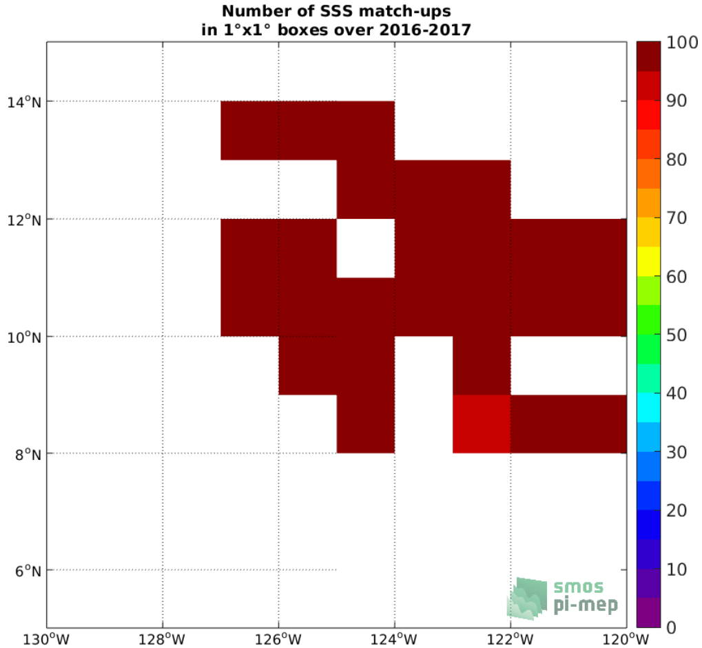
Figure 4: Number of SSS match-ups between Waveglider SSS and the SMOS and SMAP SSS L4 OI v1 - 7 Days (LOPS) SSS product for the SPURS 2 Pi-MEP region over 1^\circ \times 1^\circ boxes and for the full satellite product period.
