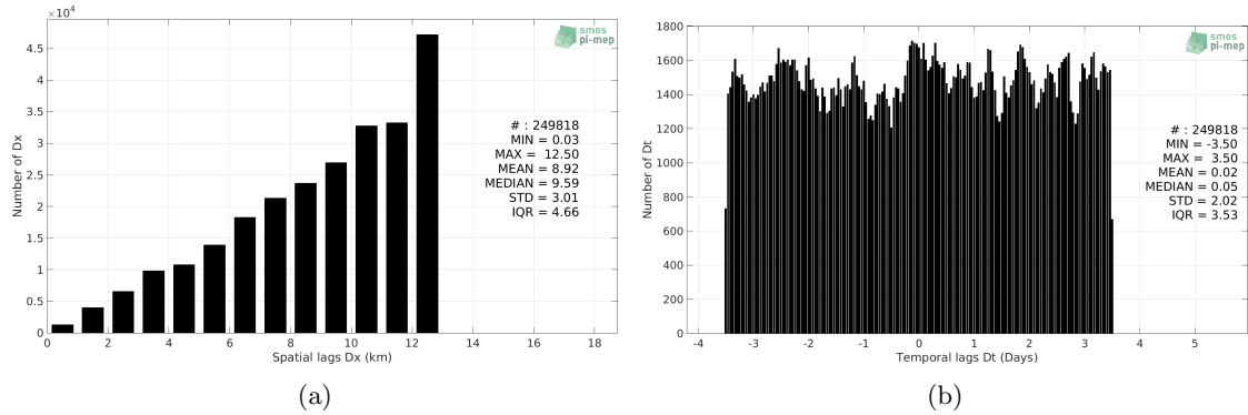
Figure 5: Histograms of the spatial (a) and temporal (b) lags between the location/time of the Waveglider measurement and the date of the corresponding SMOS and SMAP SSS L4 OI v1 - 7 Days (LOPS) SSS pixel.
