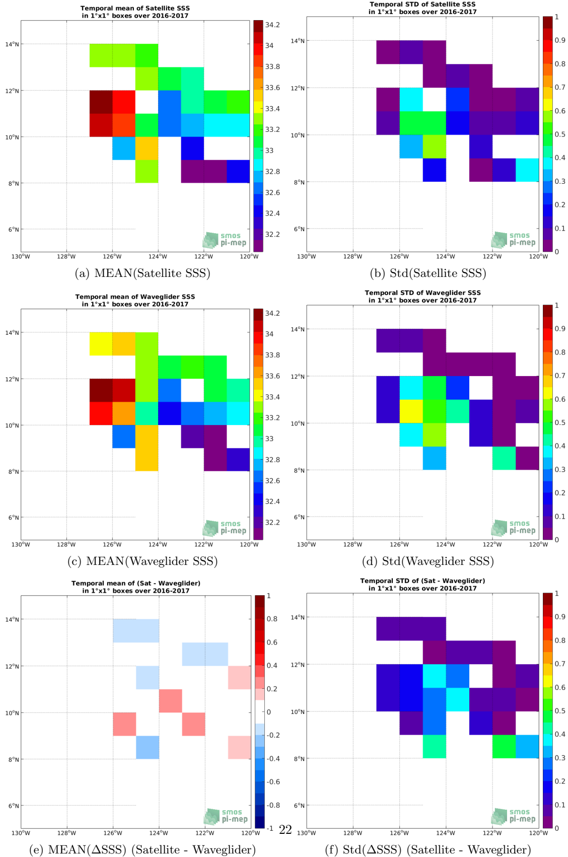
Figure 6: Temporal mean (left) and Std (right) of SSS from SMOS and SMAP SSS L4 OI v1 - 7 Days (LOPS) (top), Waveglider (middle), and of \Delta SSS (Satellite - Waveglider). Only match-up pairs are used to generate these maps.
