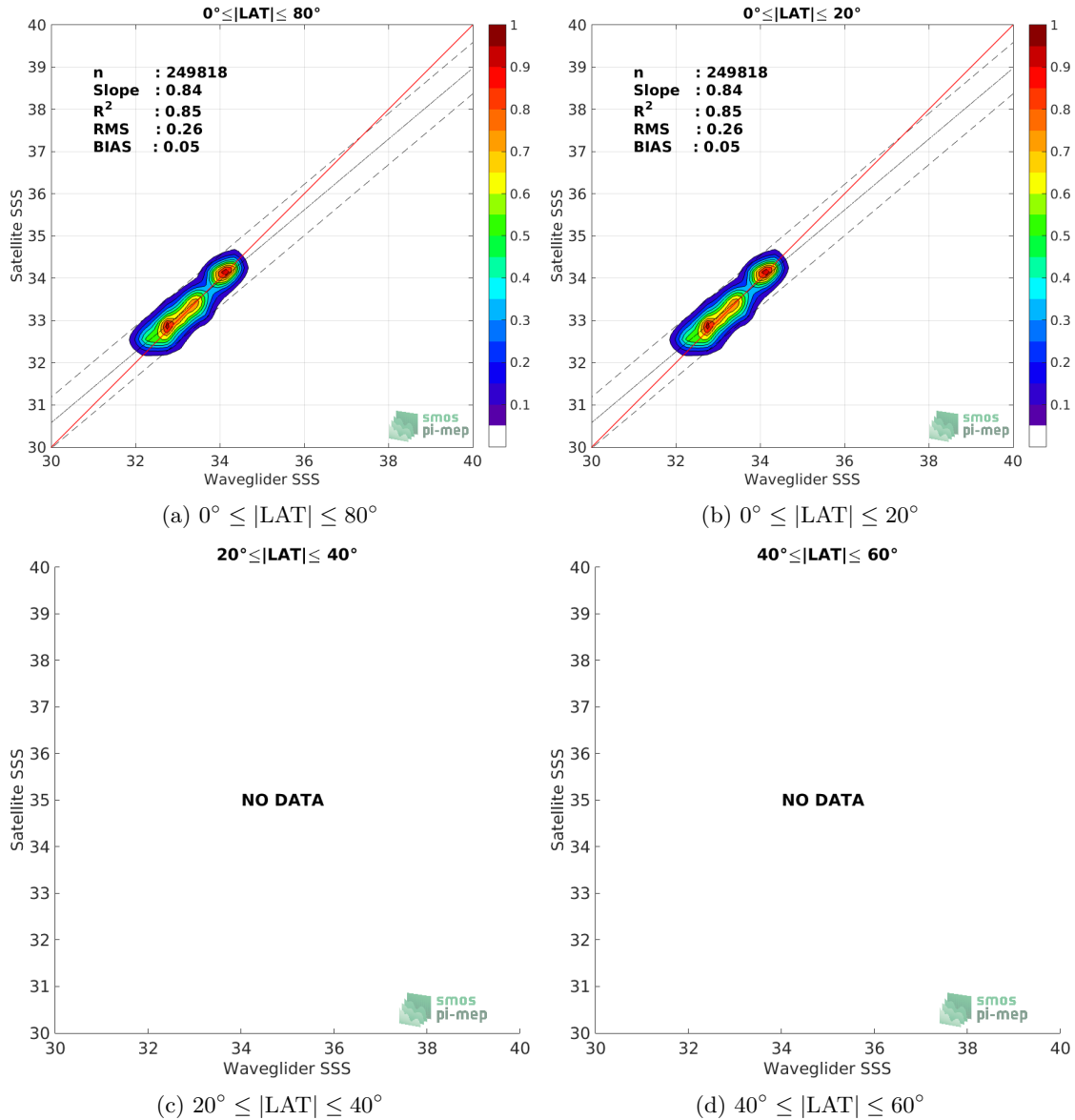
Figure 9: Contour maps of the concentration of SMOS and SMAP SSS L4 OI v1 - 7 Days (LOPS) SSS (y-axis) versus Waveglider SSS (x-axis) at match-up pairs for different latitude bands. For each plot, the red line shows x=y . The black thin and dashed lines indicate a linear fit through the data cloud and the \pm 95\% confidence levels, respectively. The number match-up pairs n , the slope and R^2 coefficient of the linear fit, the root mean square (RMS) and the mean bias between satellite and in situ data are indicated for each latitude band in each plots.
