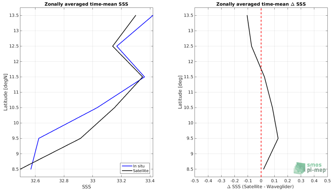
Figure 8: Left panel: Zonal mean SSS from SMOS and SMAP SSS L4 OI v1 - 7 Days (LOPS) satellite product (black) and from Waveglider (blue). Right panel: Zonal mean of \Delta SSS (Satellite - Waveglider) for all the collected Pi-MEP match-up pairs estimated over the full satellite product period.
