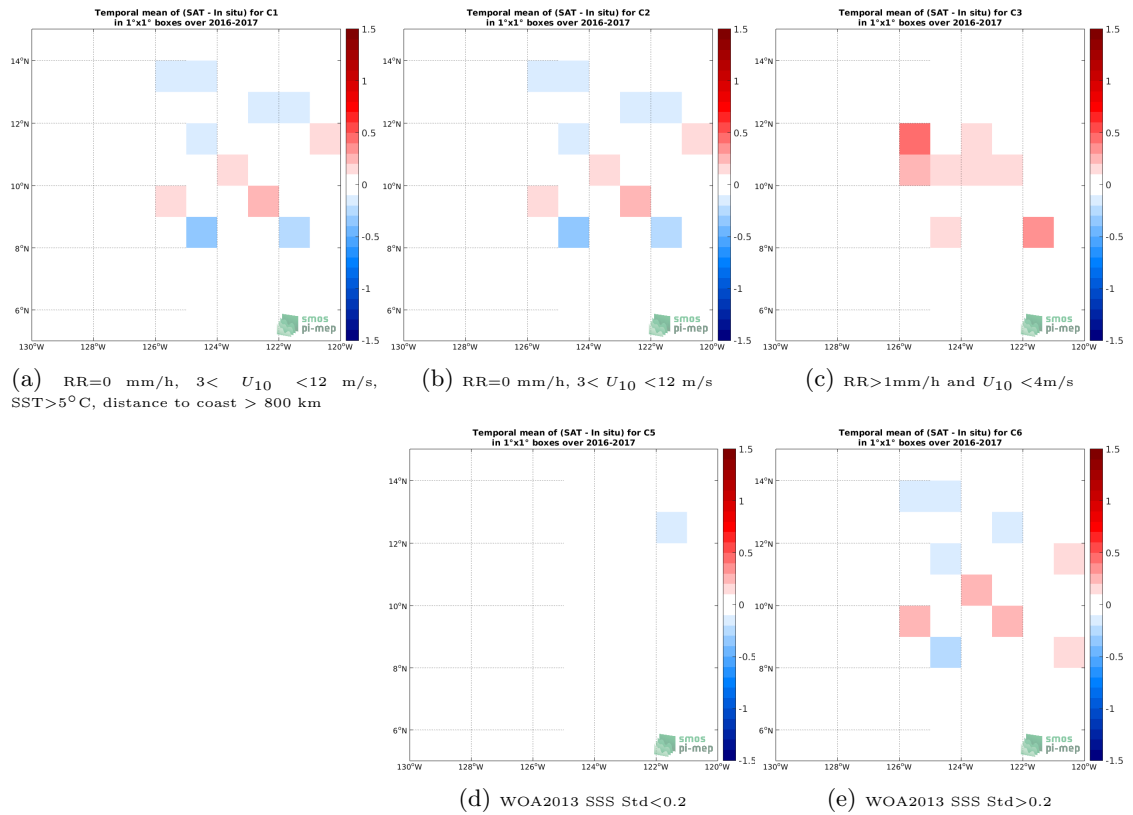
Figure 12: Temporal mean gridded over spatial boxes of size 1^\circ \times 1^\circ of \Delta SSS (SMOS and SMAP SSS L4 OI v1 - 7 Days (LOPS) - Waveglider) for 5 different subdatasets corresponding to:RR=0 mm/h, 3 < U_{10} < 12 m/s, SST >5^\circ\text{C} , distance to coast > 800 km (a), RR=0 mm/h, 3 < U_{10} < 12 m/s (b), RR >1 mm/h and U_{10} < 4 m/s (c), WOA2013 SSS Std <0.2 (d), WOA2013 SSS Std >0.2 (e).
