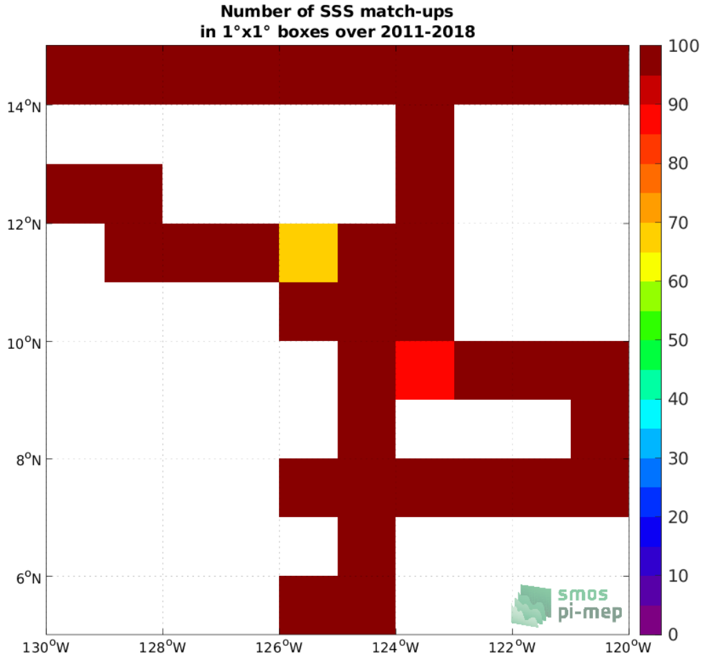
Figure 4: Number of SSS match-ups between TSG (SAMOS) SSS and the SMOS and SMAP SSS L4 OI v1 - 7 Days (LOPS) SSS product for the SPURS 2 Pi-MEP region over 1^\circ \times 1^\circ boxes and for the full satellite product period.
