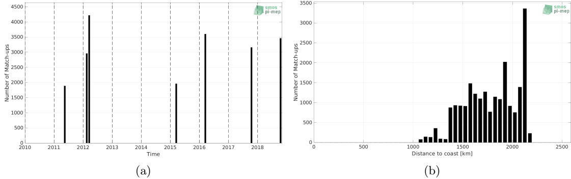
Figure 1: Number of match-ups between TSG (SAMOS) and SMOS and SMAP SSS L4 OI v1 - 7 Days (LOPS) SSS as a function of time (a) and as function of the distance to coast (b) over the SPURS 2 Pi-MEP region and for the full satellite product period.
