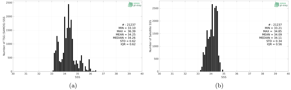
Figure 2: Histograms of SSS from TSG (SAMOS) (a) and SMOS and SMAP SSS L4 OI v1 - 7 Days (LOPS) (b) considering all match-up pairs per bins of 0.1 over the SPURS 2 Pi-MEP region and for the full satellite product period.
