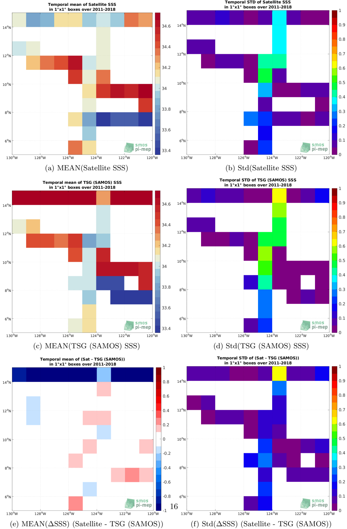
Figure 6: Temporal mean (left) and Std (right) of SSS from SMOS and SMAP SSS L4 OI v1 - 7 Days (LOPS) (top), TSG (SAMOS) (middle), and of \Delta SSS (Satellite - TSG (SAMOS)). Only match-up pairs are used to generate these maps.
