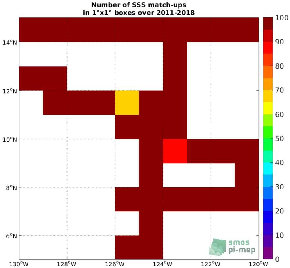
Figure 4: Number of SSS match-ups between TSG (SAMOS) SSS and the SMOS and SMAP SSS L4 OI v1 - 7 Days (LOPS) SSS product for the SPURS 2 Pi-MEP region over 1°x1° boxes and for the full satellite product period.
