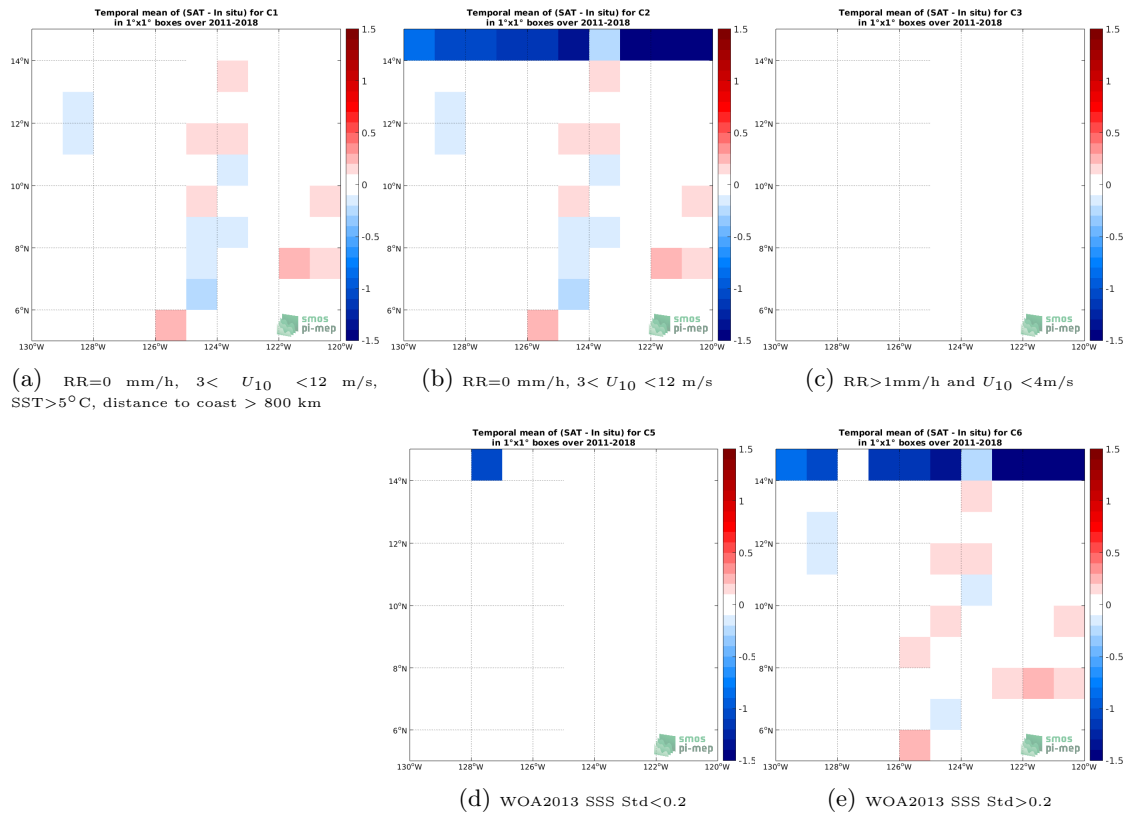
Figure 12: Temporal mean gridded over spatial boxes of size 1^\circ \times 1^\circ of \Delta\text{SSS} (SMOS and SMAP SSS L4 OI v1 - 7 Days (LOPS) - TSG (SAMOS)) for 5 different subdatasets corresponding to: RR=0 mm/h, 3 < U_{10} < 12 m/s, SST >5^\circ\text{C} , distance to coast > 800 km (a), RR=0 mm/h, 3 < U_{10} < 12 m/s (b), RR >1 mm/h and U_{10} < 4 m/s (c), WOA2013 SSS Std <0.2 (d), WOA2013 SSS Std >0.2 (e).
