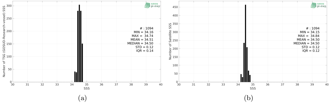
Figure 2: Histograms of SSS from TSG (GOSUD-Research-vessel) (a) and SMOS and SMAP SSS L4 OI v1 - 7 Days (LOPS) (b) considering all match-up pairs per bins of 0.1 over the SPURS 2 Pi-MEP region and for the full satellite product period.
