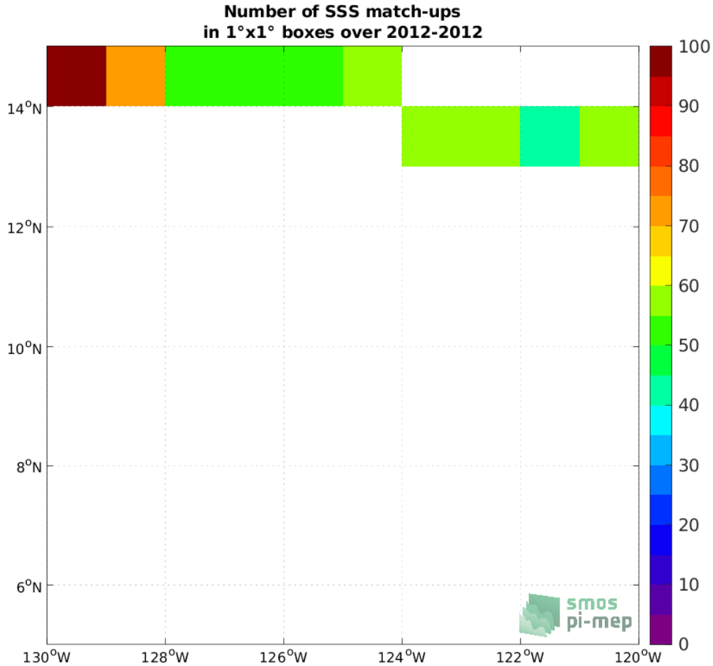
Figure 4: Number of SSS match-ups between TSG (GOSUD-Research-vessel) SSS and the SMOS and SMAP SSS L4 OI v1 - 7 Days (LOPS) SSS product for the SPURS 2 Pi-MEP region over 1^\circ \times 1^\circ boxes and for the full satellite product period.
