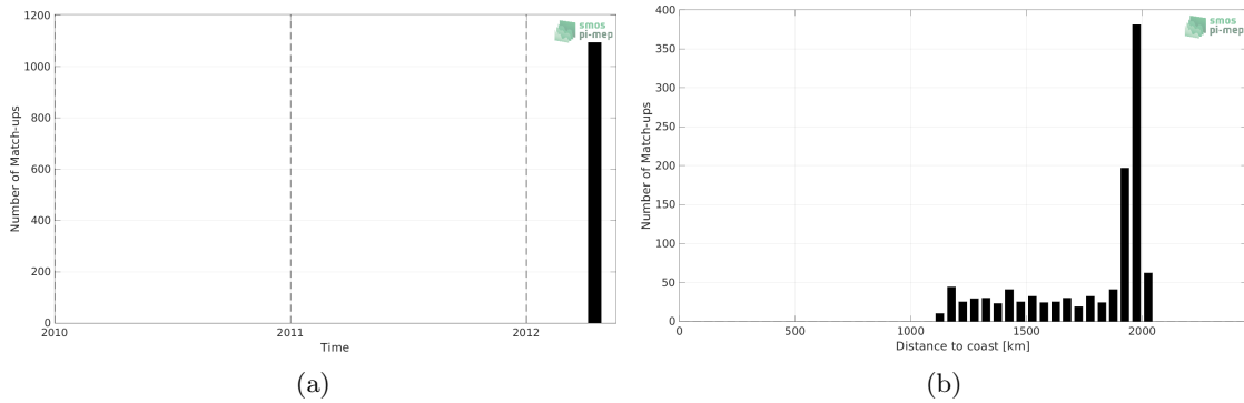
Figure 1: Number of match-ups between TSG (GOSUD-Research-vessel) and SMOS and SMAP SSS L4 OI v1 - 7 Days (LOPS) SSS as a function of time (a) and as function of the distance to coast (b) over the SPURS 2 Pi-MEP region and for the full satellite product period.
