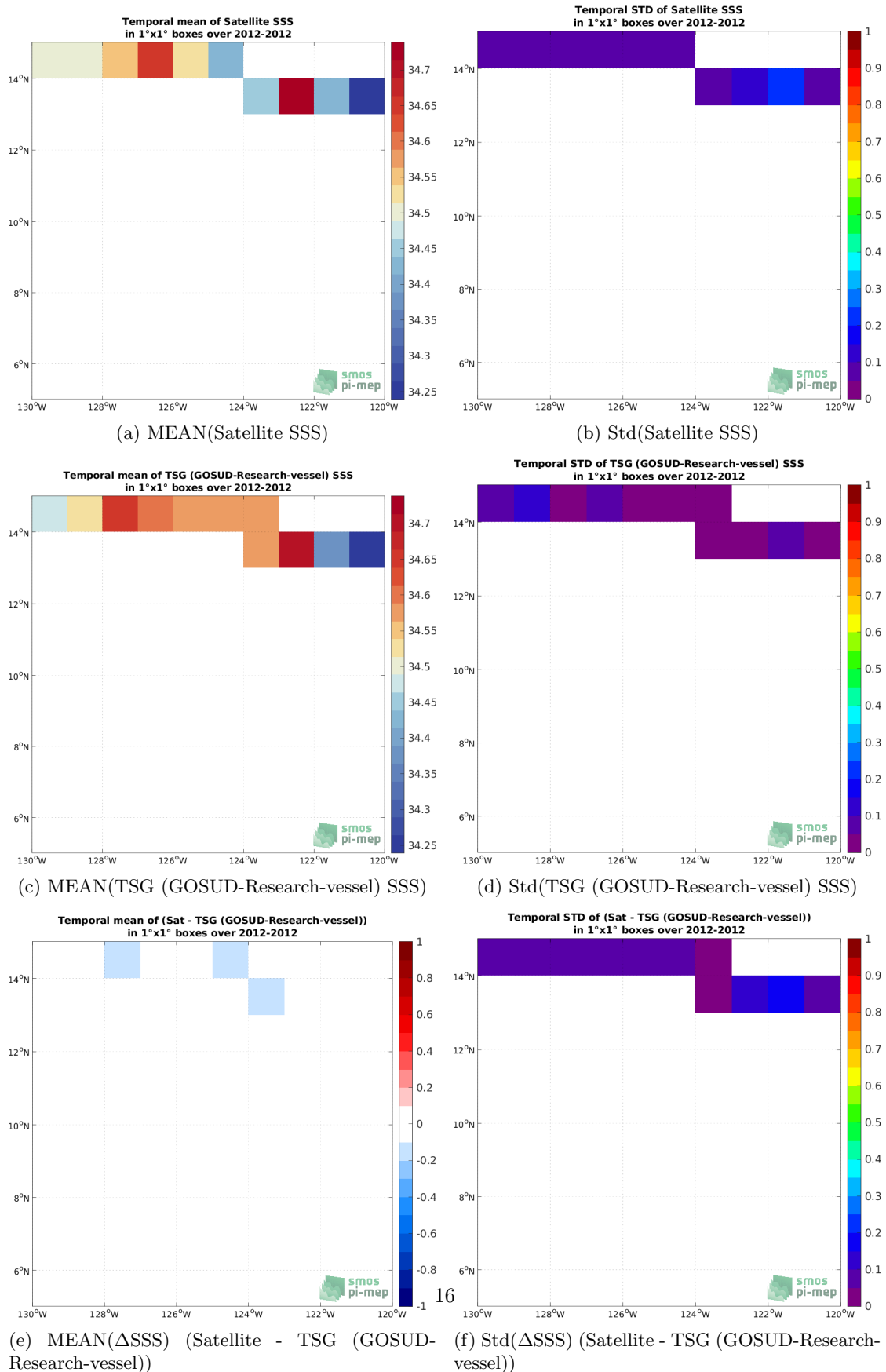
Figure 6: Temporal mean (left) and Std (right) of SSS from SMOS and SMAP SSS L4 OI v1 - 7 Days (LOPS) (top), TSG (GOSUD-Research-vessel) (middle), and of \Delta SSS (Satellite - TSG (GOSUD-Research-vessel)). Only match-up pairs are used to generate these maps.
