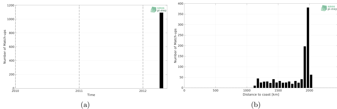
Figure 1: Number of match-ups between TSG (GOSUD-Research-vessel) and SMOS and SMAP SSS L4 OI v1 - 7 Days (LOPS) SSS as a function of time (a) and as function of the distance to coast (b) over the SPURS 2 Pi-MEP region and for the full satellite product period.
