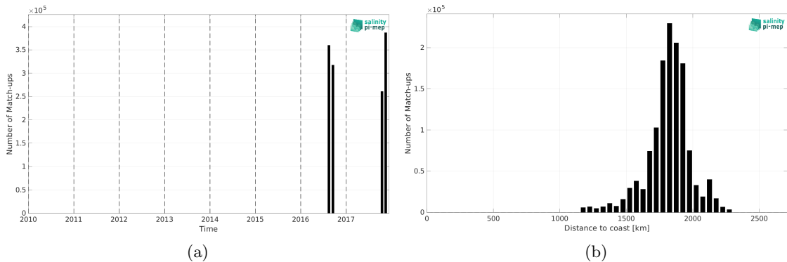
Figure 1: Number of match-ups between Salinity Snake (SPURS 2) and SMOS and SMAP SSS L4 OI v1 - 7 Days (LOPS) SSS as a function of time (a) and as function of the distance to coast (b) over the SPURS 2 Pi-MEP region and for the full satellite product period.
