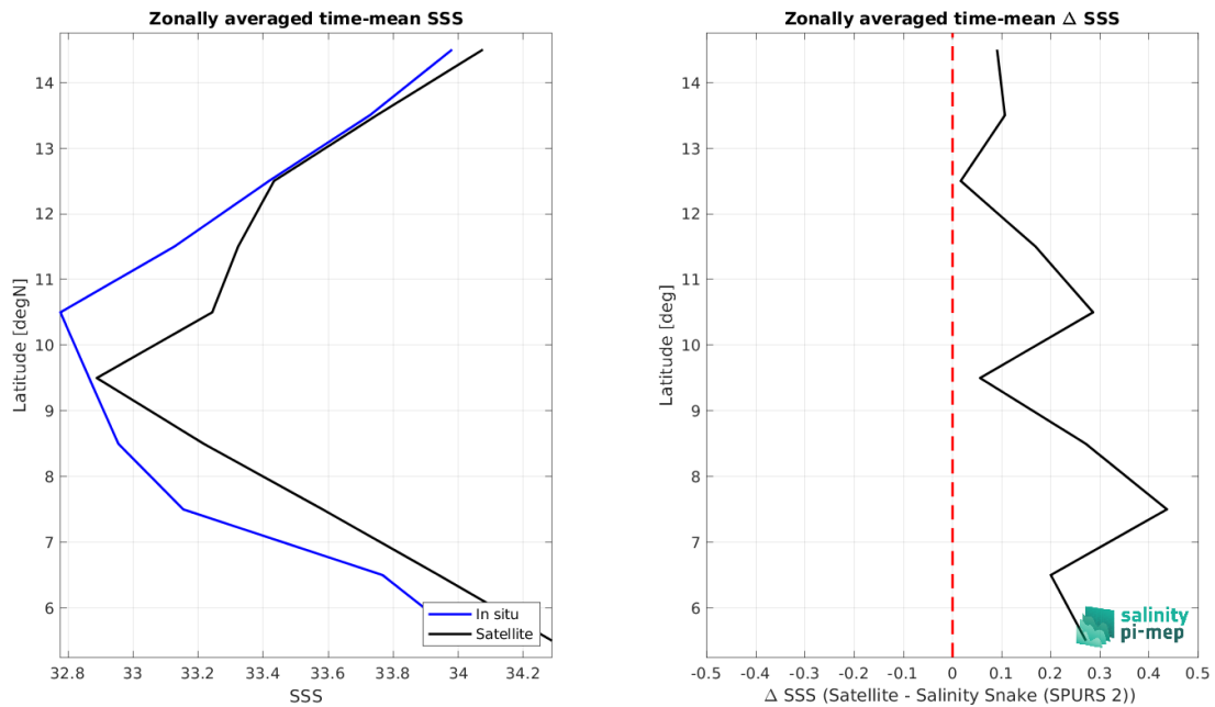
Figure 8: Left panel: Zonal mean SSS from SMOS and SMAP SSS L4 OI v1 - 7 Days (LOPS) satellite product (black) and from Salinity Snake (SPURS 2) (blue). Right panel: Zonal mean of \Delta SSS (Satellite - Salinity Snake (SPURS 2)) for all the collected Pi-MEP match-up pairs estimated over the full satellite product period.
