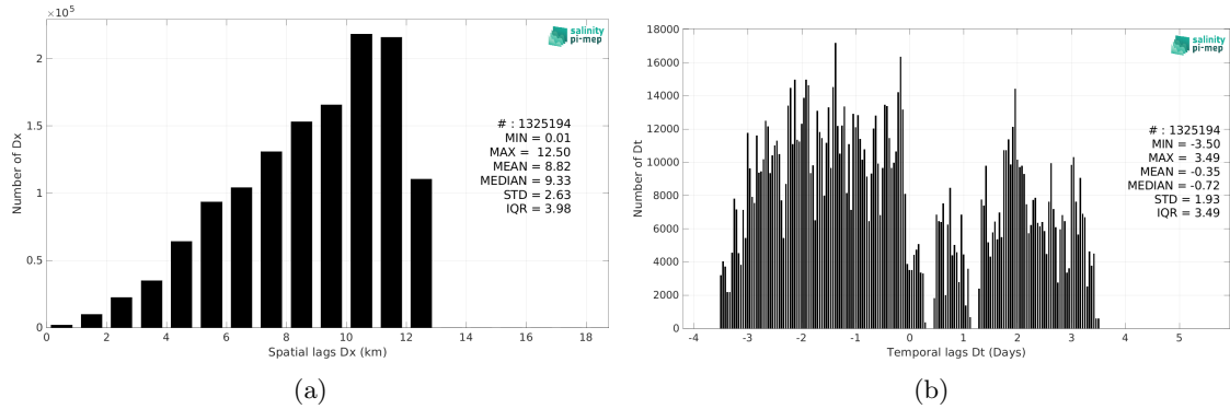
Figure 5: Histograms of the spatial (a) and temporal (b) lags between the location/time of the Salinity Snake (SPURS 2) measurement and the date of the corresponding SMOS and SMAP SSS L4 OI v1 - 7 Days (LOPS) SSS pixel.
