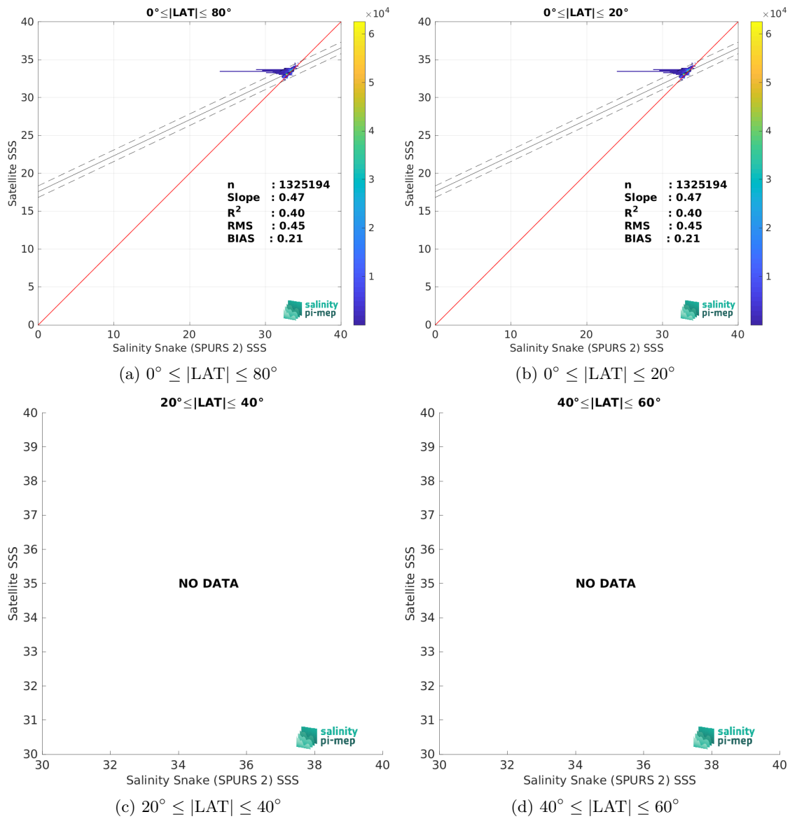
Figure 9: Contour maps of the concentration of SMOS and SMAP SSS L4 OI v1 - 7 Days (LOPS) SSS (y-axis) versus Salinity Snake (SPURS 2) SSS (x-axis) at match-up pairs for different latitude bands. For each plot, the red line shows x=y . The black thin and dashed lines indicate a linear fit through the data cloud and the \pm 95\% confidence levels, respectively. The number match-up pairs n , the slope and R^2 coefficient of the linear fit, the root mean square (RMS) and the mean bias between satellite and in situ data are indicated for each latitude band in each plots.
