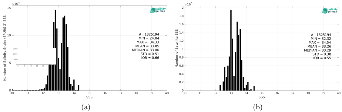
Figure 2: Histograms of SSS from Salinity Snake (SPURS 2) (a) and SMOS and SMAP SSS L4 OI v1 - 7 Days (LOPS) (b) considering all match-up pairs per bins of 0.1 over the SPURS 2 Pi-MEP region and for the full satellite product period.
