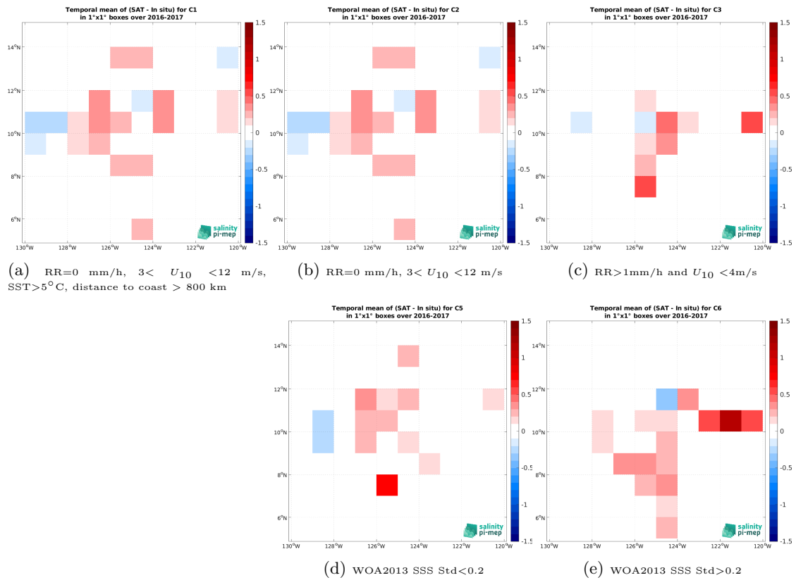
Figure 12: Temporal mean gridded over spatial boxes of size 1^\circ \times 1^\circ of \Delta\text{SSS} (SMOS and SMAP SSS L4 OI v1 - 7 Days (LOPS) - Salinity Snake (SPURS 2)) for 5 different subdatasets corresponding to:RR=0 mm/h, 3 < U_{10} < 12 m/s, SST>5°C, distance to coast > 800 km (a), RR=0 mm/h, 3 < U_{10} < 12 m/s (b), RR>1mm/h and U_{10} < 4 m/s (c), WOA2013 SSS Std<0.2 (d), WOA2013 SSS Std>0.2 (e).
