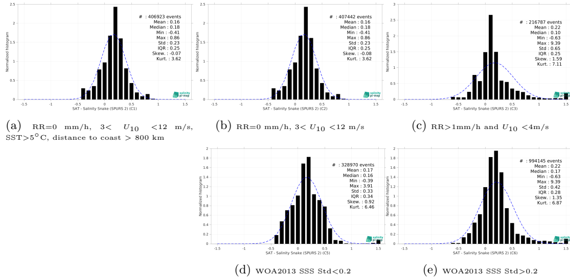
Figure 13: Normalized histogram of \Delta SSS (SMOS and SMAP SSS L4 OI v1 - 7 Days (LOPS) - Salinity Snake (SPURS 2)) for 5 different subdatasets corresponding to: RR=0 mm/h, 3 < U_{10} < 12 m/s, SST > 5°C, distance to coast > 800 km (a), RR=0 mm/h, 3 < U_{10} < 12 m/s (b), RR > 1mm/h and U_{10} < 4 m/s (c), WOA2013 SSS Std < 0.2 (d), WOA2013 SSS Std > 0.2 (e).
