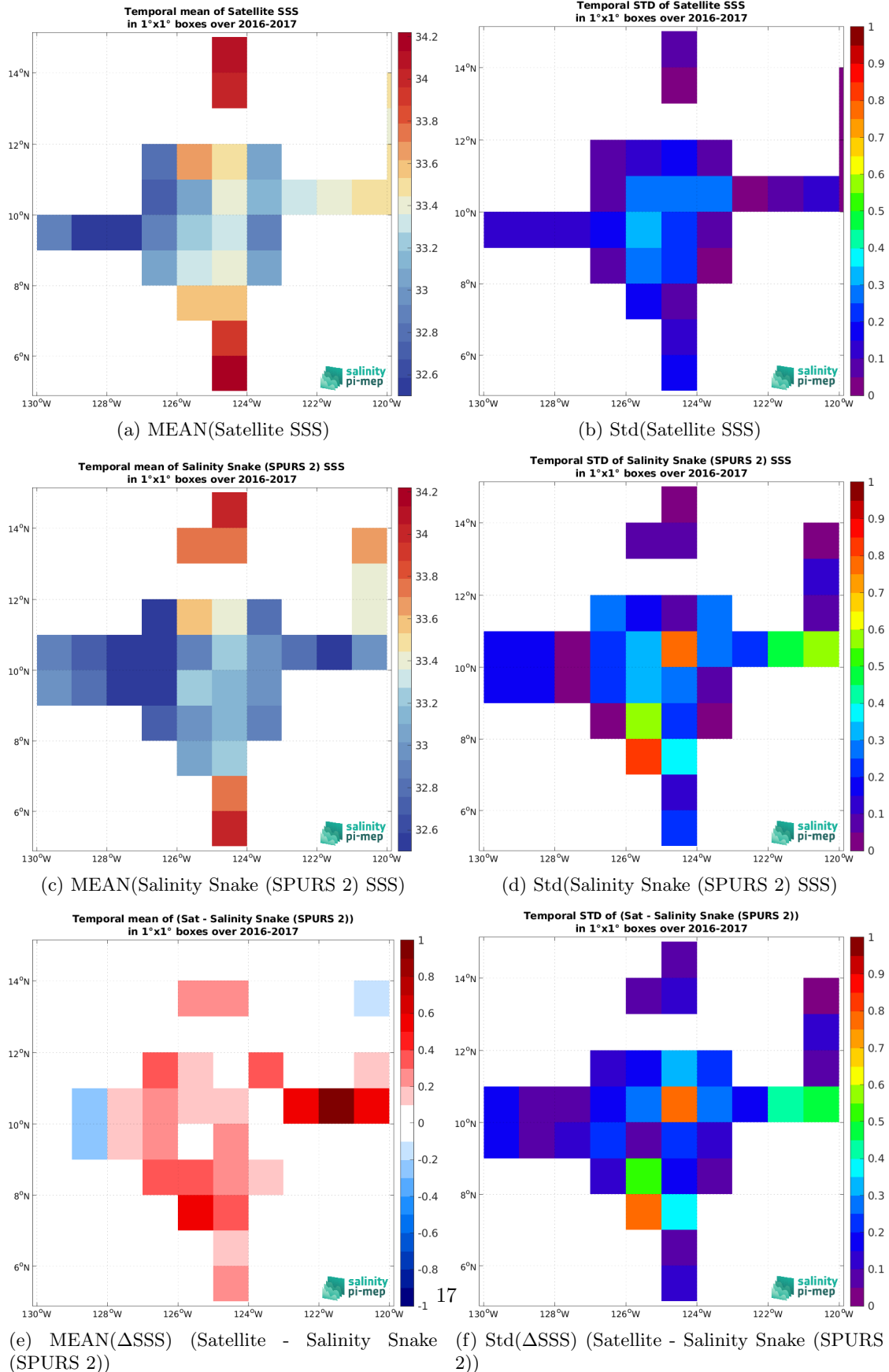
Figure 6: Temporal mean (left) and Std (right) of SSS from SMOS and SMAP SSS L4 OI v1 - 7 Days (LOPS) (top), Salinity Snake (SPURS 2) (middle), and of \Delta SSS (Satellite - Salinity Snake (SPURS 2)). Only match-up pairs are used to generate these maps.
