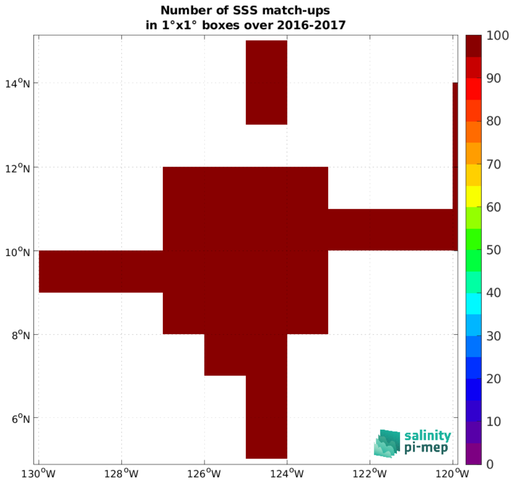
Figure 4: Number of SSS match-ups between Salinity Snake (SPURS 2) SSS and the SMOS and SMAP SSS L4 OI v1 - 7 Days (LOPS) SSS product for the SPURS 2 Pi-MEP region over 1°x1° boxes and for the full satellite product period.
