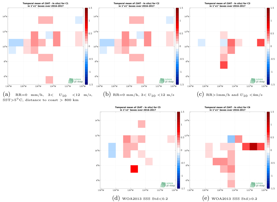
Figure 12: Temporal mean gridded over spatial boxes of size 1^\circ \times 1^\circ of \Delta SSS (SMOS and SMAP SSS L4 OI v1 - 7 Days (LOPS) - Salinity Snake (SPURS 2)) for 5 different subdatasets corresponding to:RR=0 mm/h, 3 < U_{10} < 12 m/s, SST >5^\circ C, distance to coast > 800 km (a), RR=0 mm/h, 3 < U_{10} < 12 m/s (b), RR >1 mm/h and U_{10} < 4 m/s (c), WOA2013 SSS Std <0.2 (d), WOA2013 SSS Std >0.2 (e).
