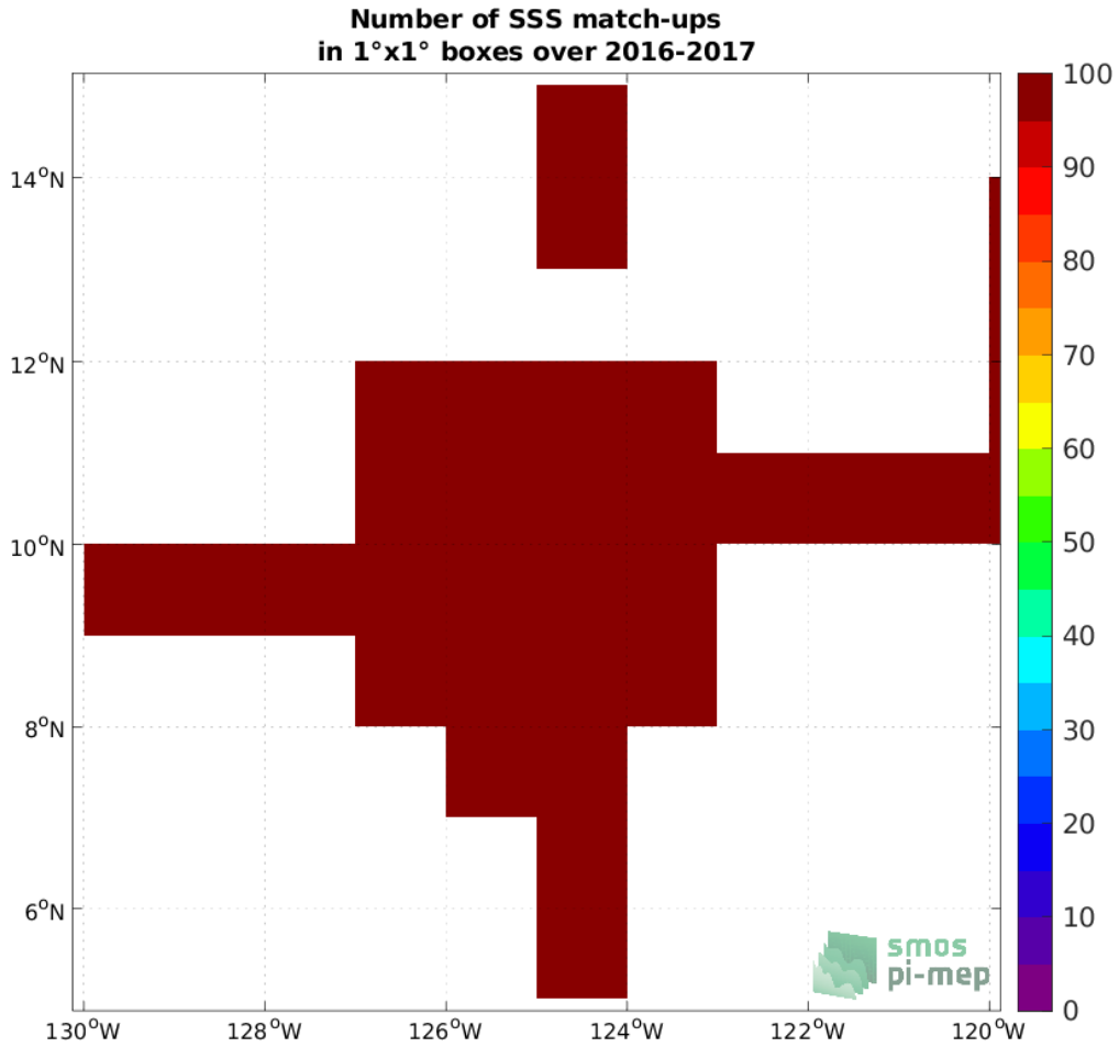
Figure 4: Number of SSS match-ups between Salinity Snake (SPURS 2) SSS and the SMOS and SMAP SSS L4 OI v1 - 7 Days (LOPS) SSS product for the SPURS 2 Pi-MEP region over 1^\circ \times 1^\circ boxes and for the full satellite product period.
