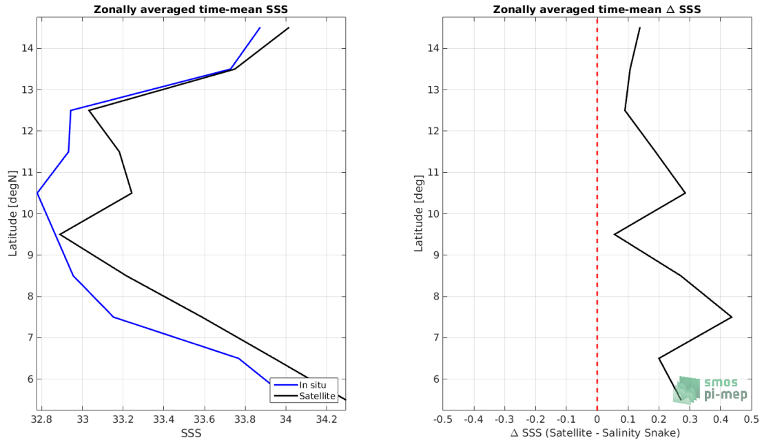
Figure 8: Left panel: Zonal mean SSS from SMOS and SMAP SSS L4 OI v1 - 7 Days (LOPS) satellite product (black) and from Salinity Snake (blue). Right panel: Zonal mean of \Delta SSS (Satellite - Salinity Snake) for all the collected Pi-MEP match-up pairs estimated over the full satellite product period.
