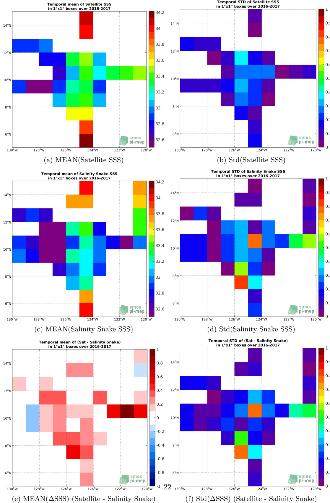
Figure 6: Temporal mean (left) and Std (right) of SSS from SMOS and SMAP SSS L4 OI v1 - 7 Days (LOPS) (top), Salinity Snake (middle), and of \Delta SSS (Satellite - Salinity Snake). Only match-up pairs are used to generate these maps.
