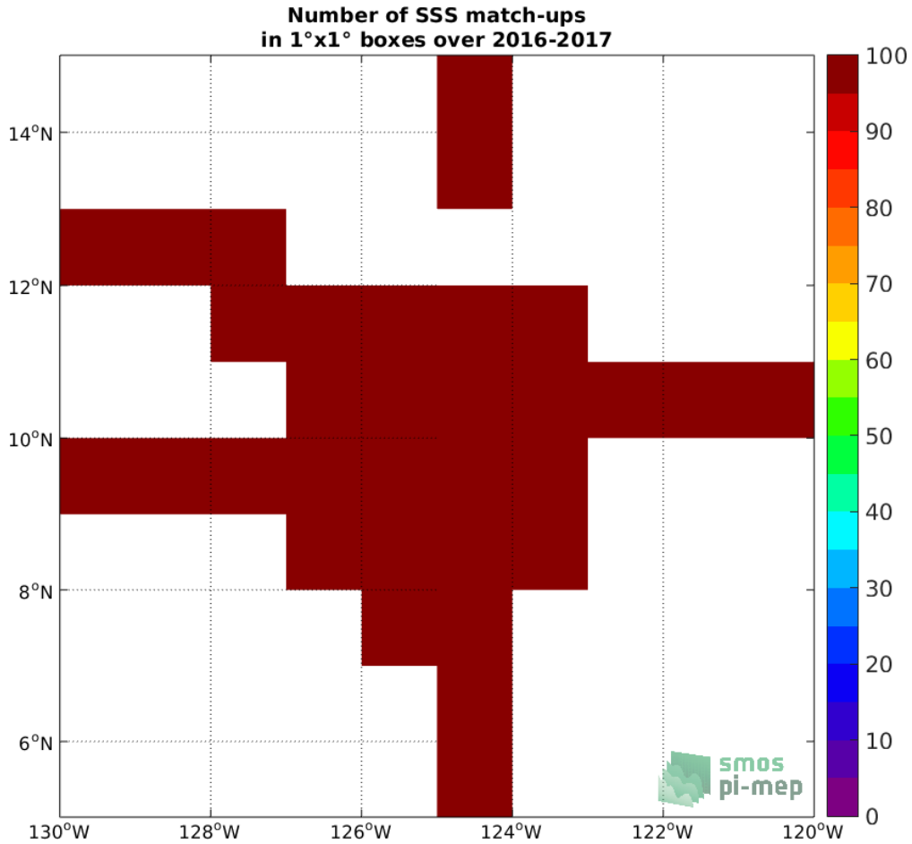
Figure 4: Number of SSS match-ups between Salinity Snake SSS and the SMOS and SMAP SSS L4 OI v1 - 7 Days (LOPS) SSS product for the SPURS 2 Pi-MEP region over 1^\circ \times 1^\circ boxes and for the full satellite product period.
