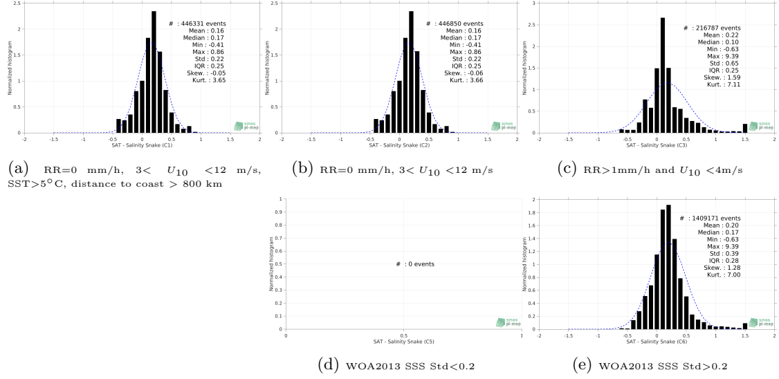
Figure 13: Normalized histogram of \Delta SSS (SMOS and SMAP SSS L4 OI v1 - 7 Days (LOPS) - Salinity Snake) for 5 different subdatasets corresponding to: RR=0 mm/h, 3 < U_{10} < 12 m/s, SST>5°C, distance to coast > 800 km (a), RR=0 mm/h, 3 < U_{10} < 12 m/s (b), RR>1mm/h and U_{10} < 4 m/s (c), WOA2013 SSS Std<0.2 (d), WOA2013 SSS Std>0.2 (e).
