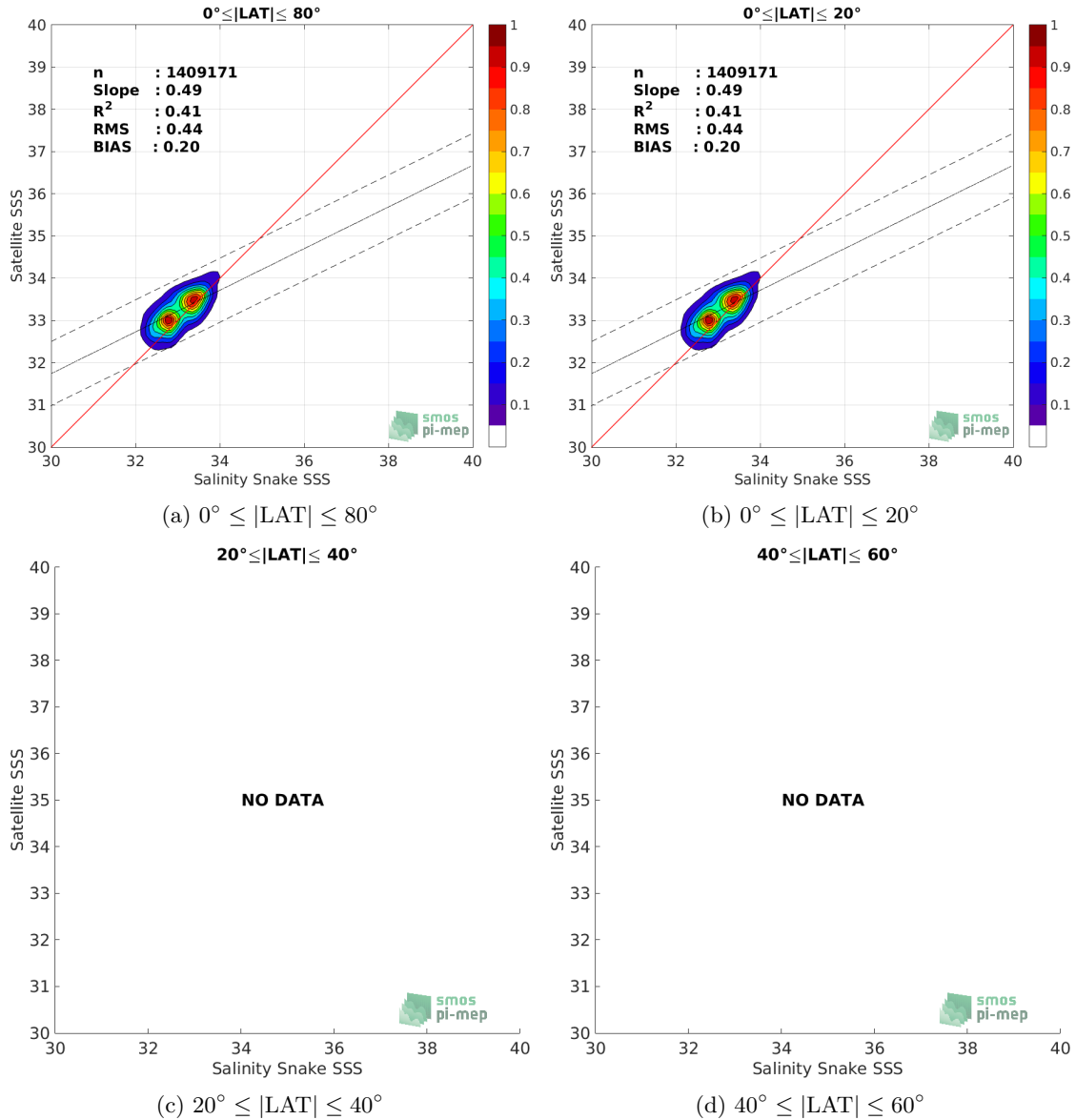
Figure 9: Contour maps of the concentration of SMOS and SMAP SSS L4 OI v1 - 7 Days (LOPS) SSS (y-axis) versus Salinity Snake SSS (x-axis) at match-up pairs for different latitude bands. For each plot, the red line shows x=y . The black thin and dashed lines indicate a linear fit through the data cloud and the \pm 95\% confidence levels, respectively. The number match-up pairs n , the slope and R^2 coefficient of the linear fit, the root mean square (RMS) and the mean bias between satellite and in situ data are indicated for each latitude band in each plots.
