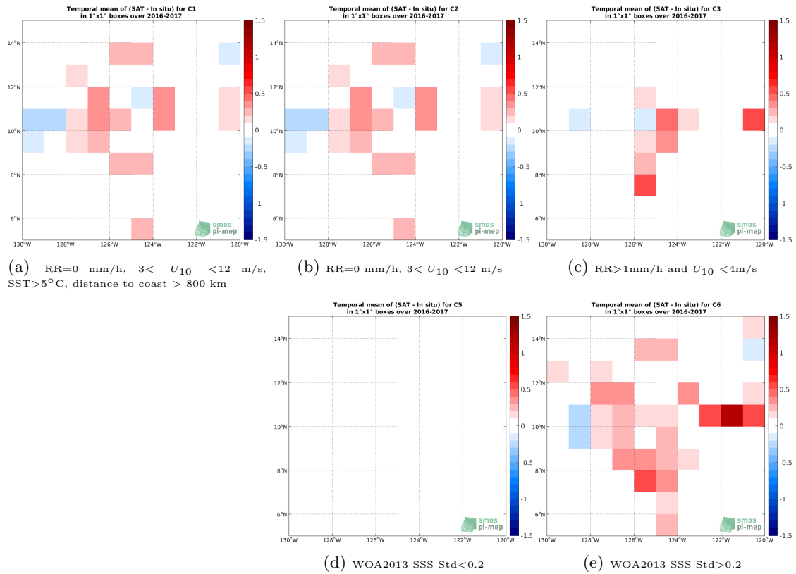
Figure 12: Temporal mean gridded over spatial boxes of size 1^\circ \times 1^\circ of \Delta SSS (SMOS and SMAP SSS L4 OI v1 - 7 Days (LOPS) - Salinity Snake) for 5 different subdatasets corresponding to: RR=0 mm/h, 3 < U_{10} < 12 m/s, SST >5^\circ\text{C} , distance to coast > 800 km (a), RR=0 mm/h, 3 < U_{10} < 12 m/s (b), RR >1 mm/h and U_{10} < 4 m/s (c), WOA2013 SSS Std <0.2 (d), WOA2013 SSS Std >0.2 (e).
