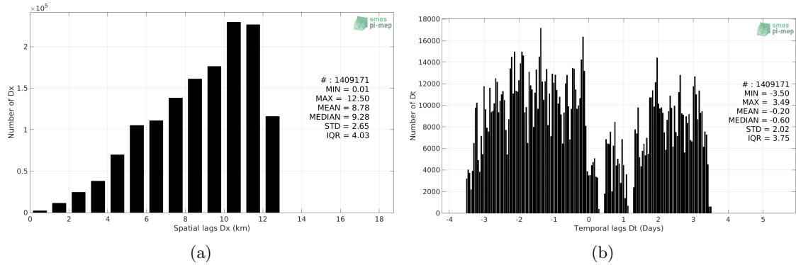
Figure 5: Histograms of the spatial (a) and temporal (b) lags between the location/time of the Salinity Snake measurement and the date of the corresponding SMOS and SMAP SSS L4 OI v1 - 7 Days (LOPS) SSS pixel.
