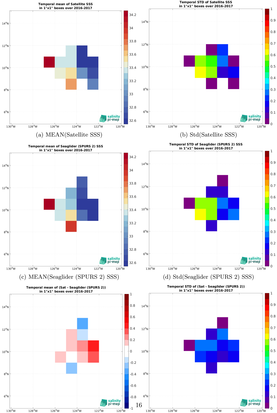
Figure 6: Temporal mean (left) and Std (right) of SSS from SMOS and SMAP SSS L4 OI v1 - 7 Days (LOPS) (top), Seaglider (SPURS 2) (middle), and of \Delta SSS (Satellite - Seaglider (SPURS 2)). Only match-up pairs are used to generate these maps.
