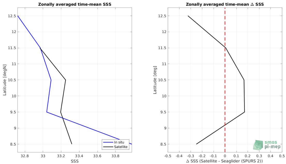
Figure 8: Left panel: Zonal mean SSS from SMOS and SMAP SSS L4 OI v1 - 7 Days (LOPS) satellite product (black) and from Seaglider (SPURS 2) (blue). Right panel: Zonal mean of \Delta SSS (Satellite - Seaglider (SPURS 2)) for all the collected Pi-MEP match-up pairs estimated over the full satellite product period.
