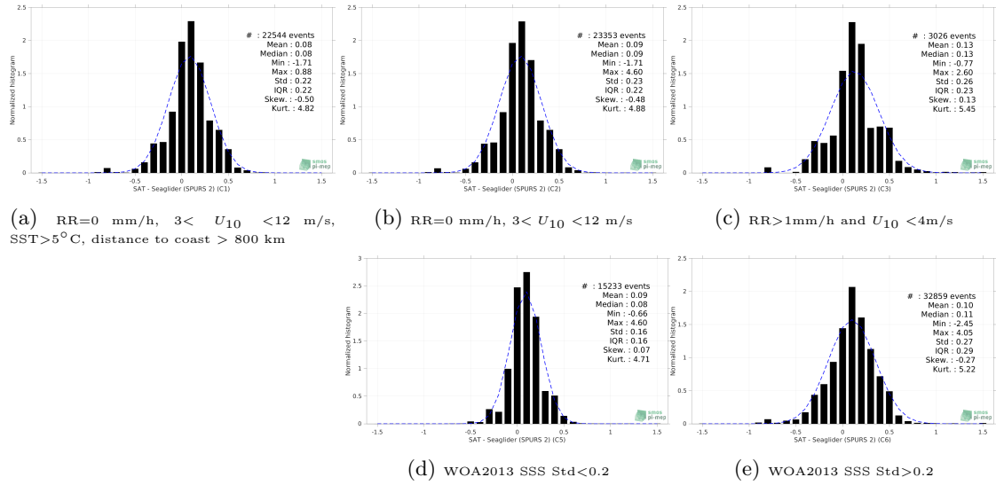
Figure 13: Normalized histogram of \Delta SSS (SMOS and SMAP SSS L4 OI v1 - 7 Days (LOPS) - Seaglider (SPURS 2)) for 5 different subdatasets corresponding to: RR=0 mm/h, 3 < U_{10} < 12 m/s, SST>5°C, distance to coast > 800 km (a), RR=0 mm/h, 3 < U_{10} < 12 m/s (b), RR>1mm/h and U_{10} < 4 m/s (c), WOA2013 SSS Std<0.2 (d), WOA2013 SSS Std>0.2 (e).
