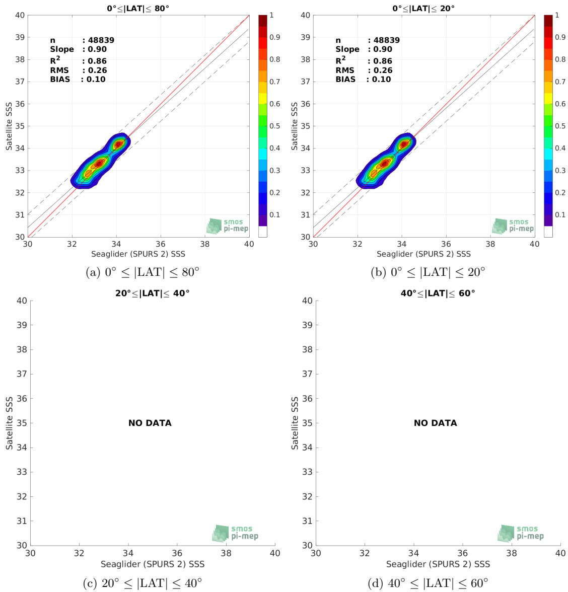
Figure 9: Contour maps of the concentration of SMOS and SMAP SSS L4 OI v1 - 7 Days (LOPS) SSS (y-axis) versus Seaglider (SPURS 2) SSS (x-axis) at match-up pairs for different latitude bands. For each plot, the red line shows x=y . The black thin and dashed lines indicate a linear fit through the data cloud and the \pm 95\% confidence levels, respectively. The number match-up pairs n , the slope and R^2 coefficient of the linear fit, the root mean square (RMS) and the mean bias between satellite and in situ data are indicated for each latitude band in each plots.
