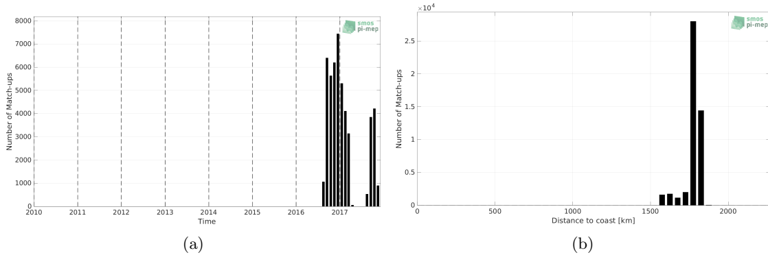
Figure 1: Number of match-ups between Seaglider (SPURS 2) and SMOS and SMAP SSS L4 OI v1 - 7 Days (LOPS) SSS as a function of time (a) and as function of the distance to coast (b) over the SPURS 2 Pi-MEP region and for the full satellite product period.
