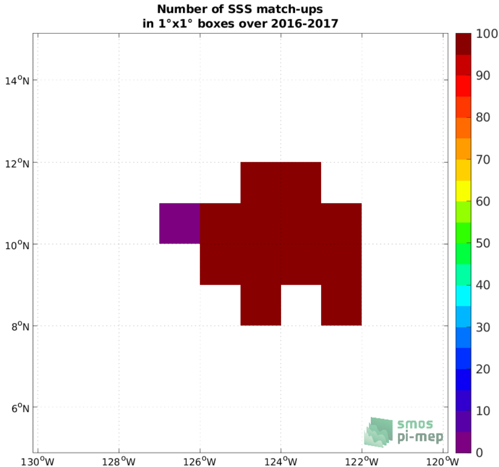
Figure 4: Number of SSS match-ups between Seaglider (SPURS 2) SSS and the SMOS and SMAP SSS L4 OI v1 - 7 Days (LOPS) SSS product for the SPURS 2 Pi-MEP region over 1^\circ \times 1^\circ boxes and for the full satellite product period.
