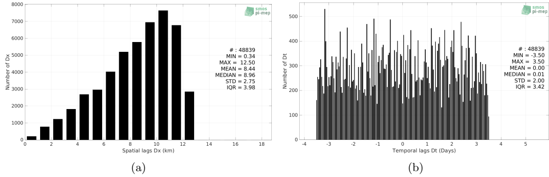
Figure 5: Histograms of the spatial (a) and temporal (b) lags between the location/time of the Seaglider (SPURS 2) measurement and the date of the corresponding SMOS and SMAP SSS L4 OI v1 - 7 Days (LOPS) SSS pixel.
