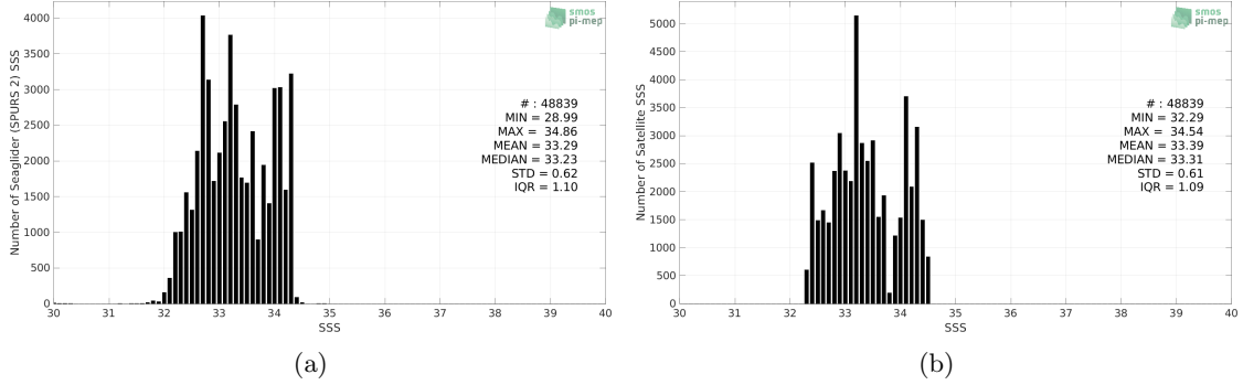
Figure 2: Histograms of SSS from Seaglider (SPURS 2) (a) and SMOS and SMAP SSS L4 OI v1 - 7 Days (LOPS) (b) considering all match-up pairs per bins of 0.1 over the SPURS 2 Pi-MEP region and for the full satellite product period.
