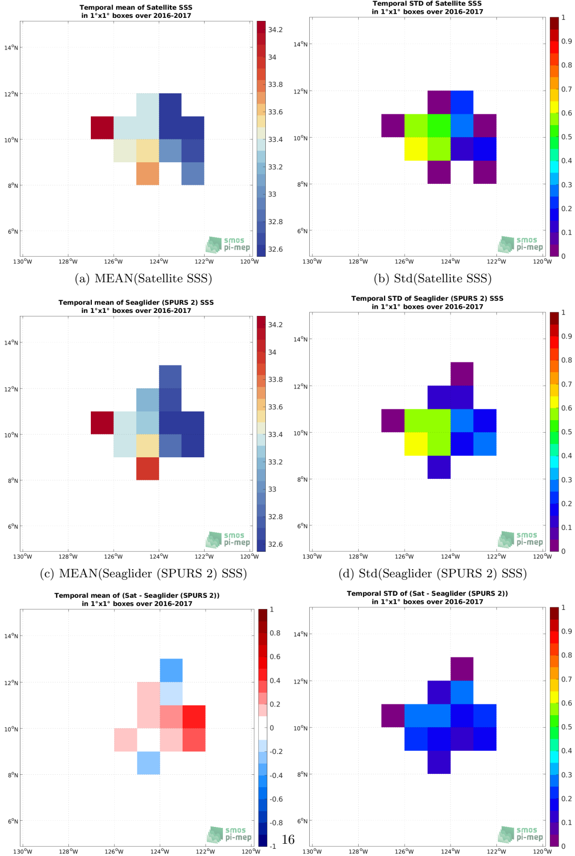
(e) MEAN( \Delta SSS) (Satellite - Seaglider (SPURS 2)) (f) Std( \Delta SSS) (Satellite - Seaglider (SPURS 2)) Figure 6: Temporal mean (left) and Std (right) of SSS from SMOS and SMAP SSS L4 OI v1 - 7 Days (LOPS) (top), Seaglider (SPURS 2) (middle), and of \Delta SSS (Satellite - Seaglider (SPURS 2)). Only match-up pairs are used to generate these maps.
