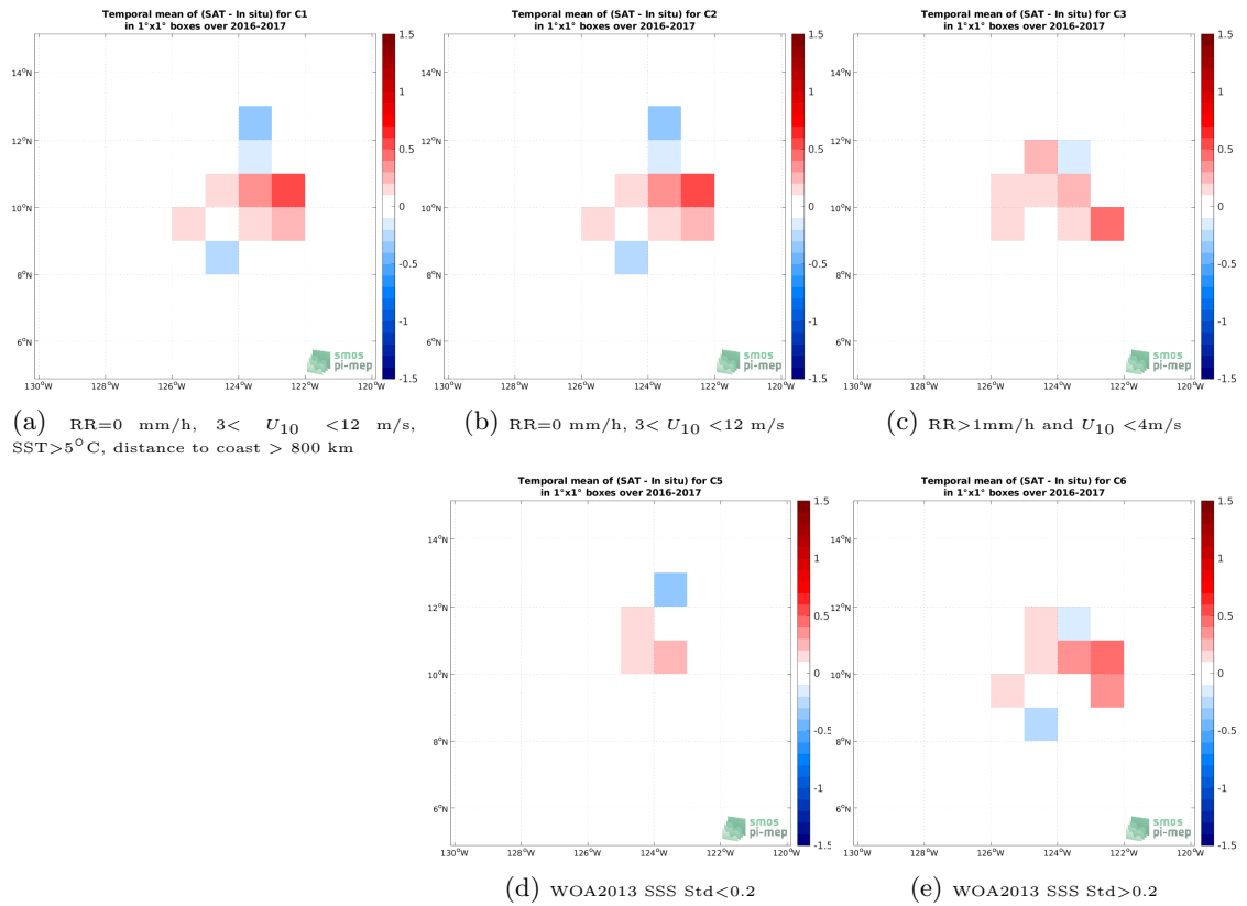
Figure 12: Temporal mean gridded over spatial boxes of size 1^\circ \times 1^\circ of \Delta SSS (SMOS and SMAP SSS L4 OI v1 - 7 Days (LOPS) - Seaglider (SPURS 2)) for 5 different subdatasets corresponding to:RR=0 mm/h, 3 < U_{10} < 12 m/s, SST >5^\circ C, distance to coast > 800 km (a), RR=0 mm/h, 3 < U_{10} < 12 m/s (b), RR >1 mm/h and U_{10} < 4 m/s (c), WOA2013 SSS Std <0.2 (d), WOA2013 SSS Std >0.2 (e).
