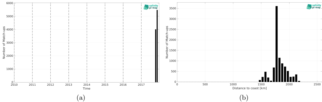
Figure 1: Number of match-ups between Saildrone and SMOS and SMAP SSS L4 OI v1 - 7 Days (LOPS) SSS as a function of time (a) and as function of the distance to coast (b) over the SPURS 2 Pi-MEP region and for the full satellite product period.
