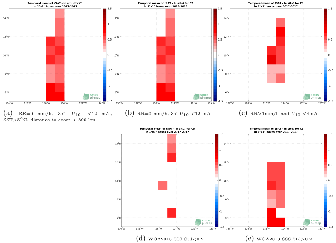
Figure 12: Temporal mean gridded over spatial boxes of size 1^\circ \times 1^\circ of \Delta SSS (SMOS and SMAP SSS L4 OI v1 - 7 Days (LOPS) - Sairdrone) for 5 different subdatasets corresponding to:RR=0 mm/h, 3 < U_{10} < 12 m/s, SST >5^\circ\text{C} , distance to coast > 800 km (a), RR=0 mm/h, 3 < U_{10} < 12 m/s (b), RR >1 mm/h and U_{10} < 4 m/s (c), WOA2013 SSS Std <0.2 (d), WOA2013 SSS Std >0.2 (e).
