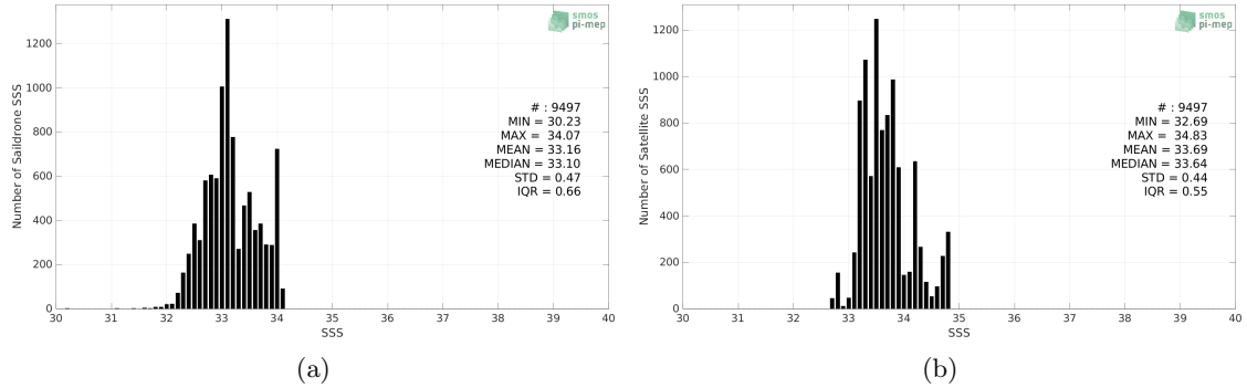
Figure 2: Histograms of SSS from Saildrone (a) and SMOS and SMAP SSS L4 OI v1 - 7 Days (LOPS) (b) considering all match-up pairs per bins of 0.1 over the SPURS 2 Pi-MEP region and for the full satellite product period.
