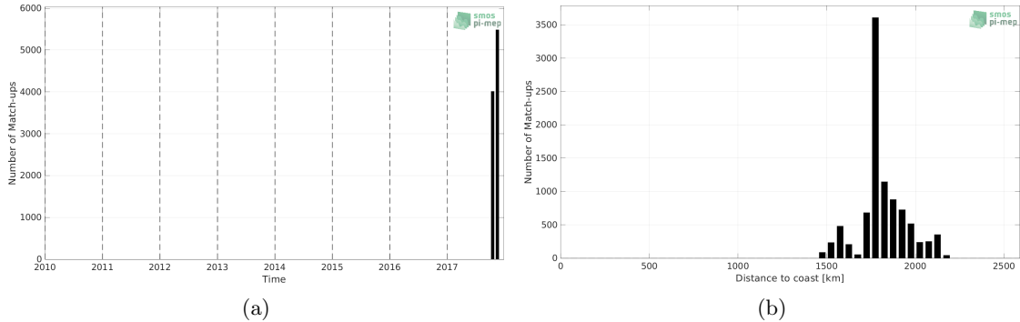
Figure 1: Number of match-ups between Sairdrone and SMOS and SMAP SSS L4 OI v1 - 7 Days (LOPS) SSS as a function of time (a) and as function of the distance to coast (b) over the SPURS 2 Pi-MEP region and for the full satellite product period.
