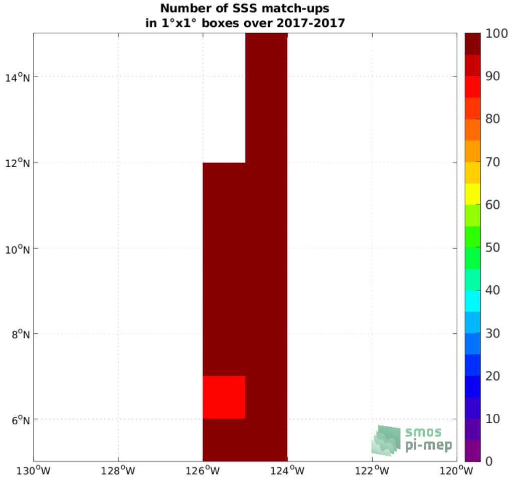
Figure 4: Number of SSS match-ups between Sairdrone SSS and the SMOS and SMAP SSS L4 OI v1 - 7 Days (LOPS) SSS product for the SPURS 2 Pi-MEP region over 1^\circ \times 1^\circ boxes and for the full satellite product period.
