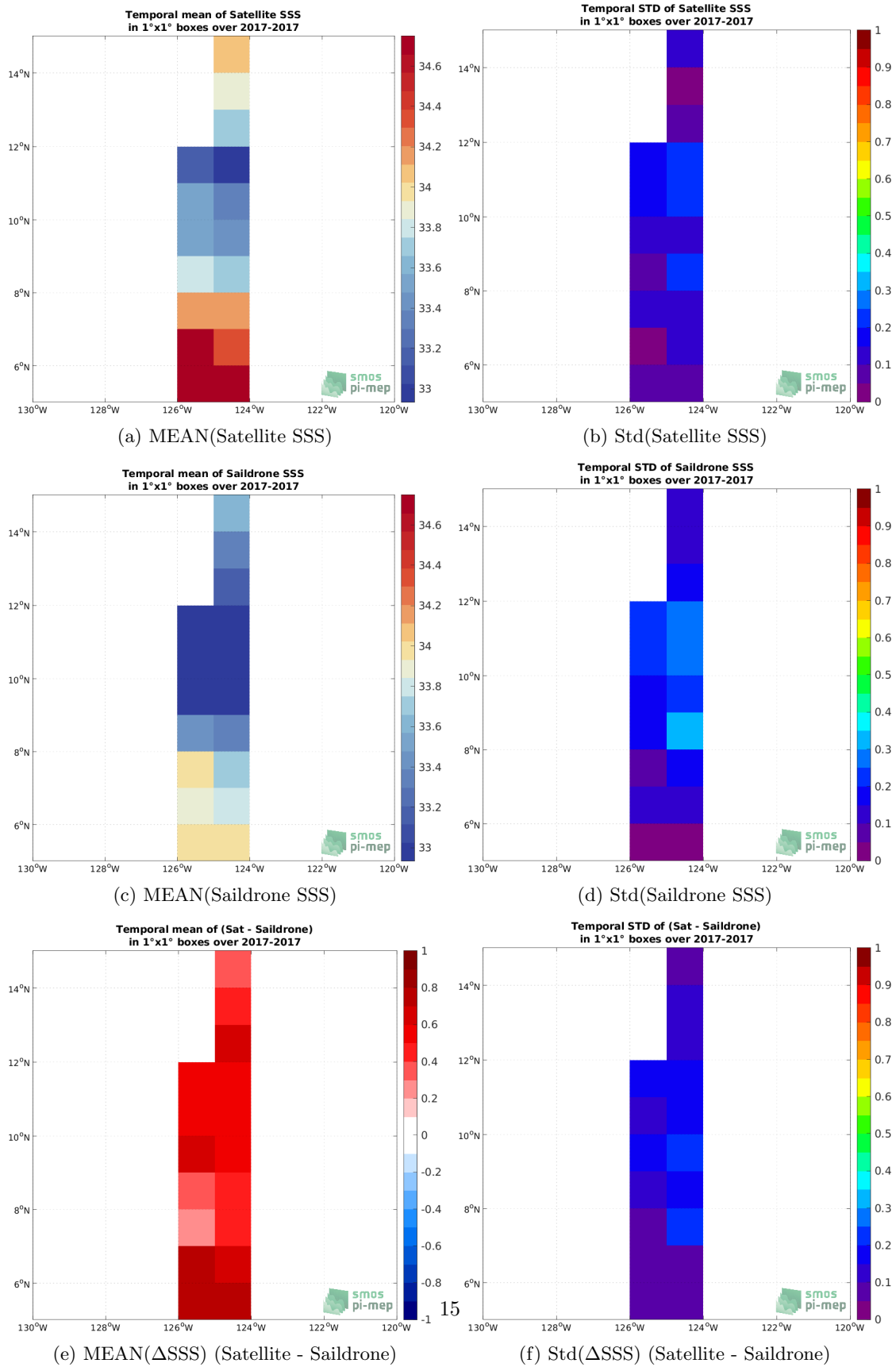
Figure 6: Temporal mean (left) and Std (right) of SSS from SMOS and SMAP SSS L4 OI v1 - 7 Days (LOPS) (top), Saildrone (middle), and of \Delta SSS (Satellite - Saildrone). Only match-up pairs are used to generate these maps.
