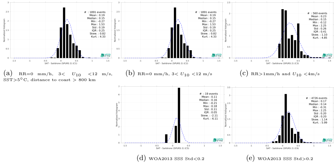
Figure 13: Normalized histogram of \Delta SSS (SMOS and SMAP SSS L4 OI v1 - 7 Days (LOPS) - Saildrone (SPURS 2)) for 5 different subdatasets corresponding to: RR=0 mm/h, 3 < U_{10} < 12 m/s, SST > 5°C, distance to coast > 800 km (a), RR=0 mm/h, 3 < U_{10} < 12 m/s (b), RR > 1mm/h and U_{10} < 4 m/s (c), WOA2013 SSS Std < 0.2 (d), WOA2013 SSS Std > 0.2 (e).
