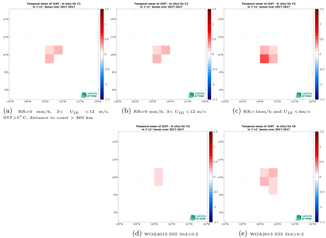
Figure 12: Temporal mean gridded over spatial boxes of size 1^\circ \times 1^\circ of \Delta SSS (SMOS and SMAP SSS L4 OI v1 - 7 Days (LOPS) - Saildrone (SPURS 2)) for 5 different subdatasets corresponding to:RR=0 mm/h, 3 < U_{10} < 12 m/s, SST >5^\circ\text{C} , distance to coast > 800 km (a), RR=0 mm/h, 3 < U_{10} < 12 m/s (b), RR >1 mm/h and U_{10} < 4 m/s (c), WOA2013 SSS Std <0.2 (d), WOA2013 SSS Std >0.2 (e).
