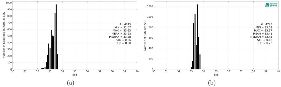
Figure 2: Histograms of SSS from Saildrone (SPURS 2) (a) and SMOS and SMAP SSS L4 OI v1 - 7 Days (LOPS) (b) considering all match-up pairs per bins of 0.1 over the SPURS 2 Pi-MEP region and for the full satellite product period.
