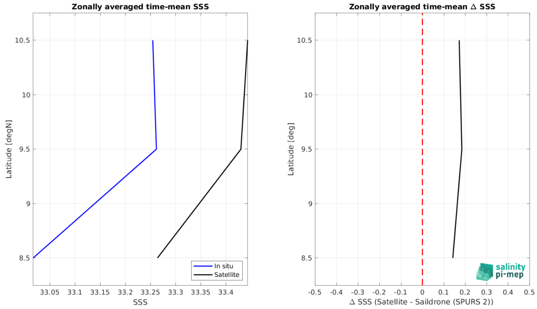
Figure 8: Left panel: Zonal mean SSS from SMOS and SMAP SSS L4 OI v1 - 7 Days (LOPS) satellite product (black) and from Sairdron (SPURS 2) (blue). Right panel: Zonal mean of \Delta SSS (Satellite - Sairdron (SPURS 2)) for all the collected Pi-MEP match-up pairs estimated over the full satellite product period.
