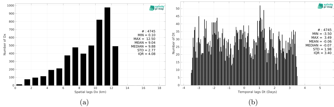
Figure 5: Histograms of the spatial (a) and temporal (b) lags between the location/time of the Saildrone (SPURS 2) measurement and the date of the corresponding SMOS and SMAP SSS L4 OI v1 - 7 Days (LOPS) SSS pixel.
