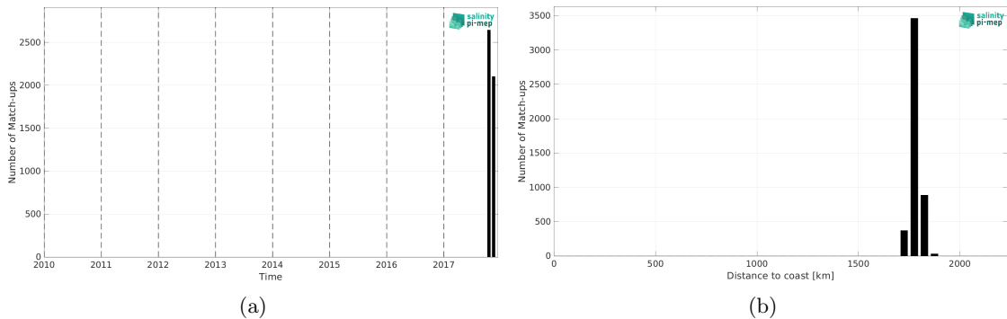
Figure 1: Number of match-ups between Saildrone (SPURS 2) and SMOS and SMAP SSS L4 OI v1 - 7 Days (LOPS) SSS as a function of time (a) and as function of the distance to coast (b) over the SPURS 2 Pi-MEP region and for the full satellite product period.
