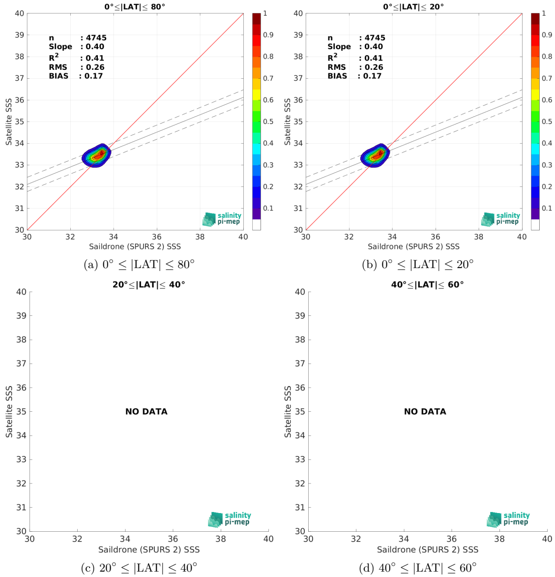
Figure 9: Contour maps of the concentration of SMOS and SMAP SSS L4 OI v1 - 7 Days (LOPS) SSS (y-axis) versus Saildrone (SPURS 2) SSS (x-axis) at match-up pairs for different latitude bands. For each plot, the red line shows x=y . The black thin and dashed lines indicate a linear fit through the data cloud and the \pm 95\% confidence levels, respectively. The number match-up pairs n , the slope and R^2 coefficient of the linear fit, the root mean square (RMS) and the mean bias between satellite and in situ data are indicated for each latitude band in each plots.
