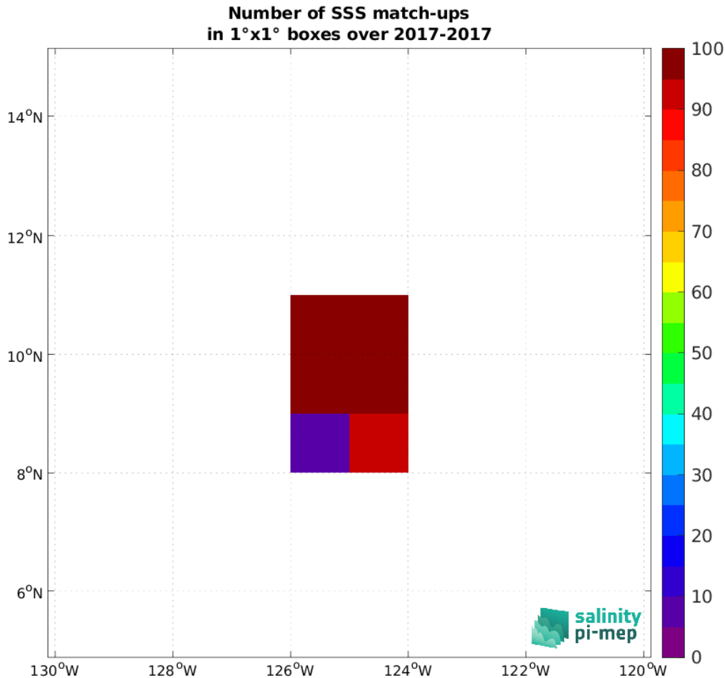
Figure 4: Number of SSS match-ups between Saildrone (SPURS 2) SSS and the SMOS and SMAP SSS L4 OI v1 - 7 Days (LOPS) SSS product for the SPURS 2 Pi-MEP region over 1^\circ \times 1^\circ boxes and for the full satellite product period.
