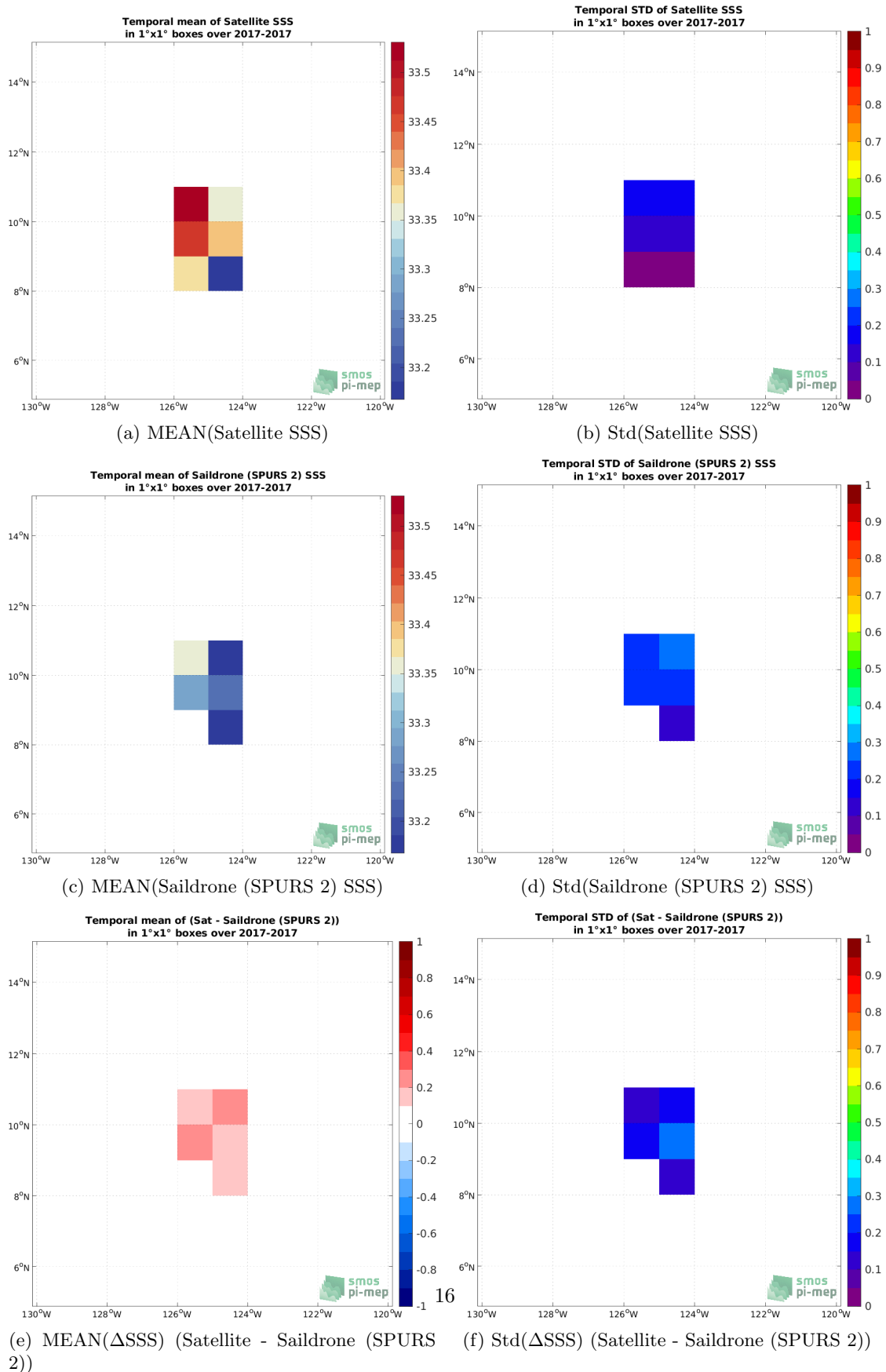
Figure 6: Temporal mean (left) and Std (right) of SSS from SMOS and SMAP SSS L4 OI v1 - 7 Days (LOPS) (top), Saildrone (SPURS 2) (middle), and of \Delta SSS (Satellite - Saildrone (SPURS 2)). Only match-up pairs are used to generate these maps.
