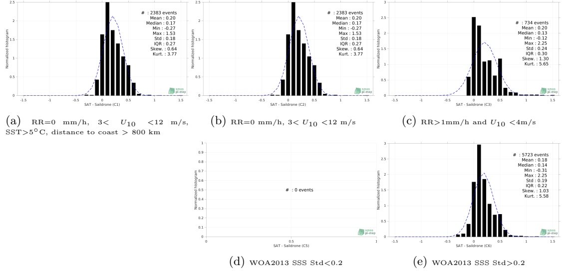
Figure 12: Normalized histogram of \Delta SSS (SMOS and SMAP SSS L4 OI v1 - 7 Days (LOPS) - Saildrone) for 5 different subdatasets corresponding to: RR=0 mm/h, 3 < U_{10} < 12 m/s, SST > 5°C, distance to coast > 800 km (a), RR=0 mm/h, 3 < U_{10} < 12 m/s (b), RR > 1mm/h and U_{10} < 4 m/s (c), WOA2013 SSS Std < 0.2 (d), WOA2013 SSS Std > 0.2 (e).
