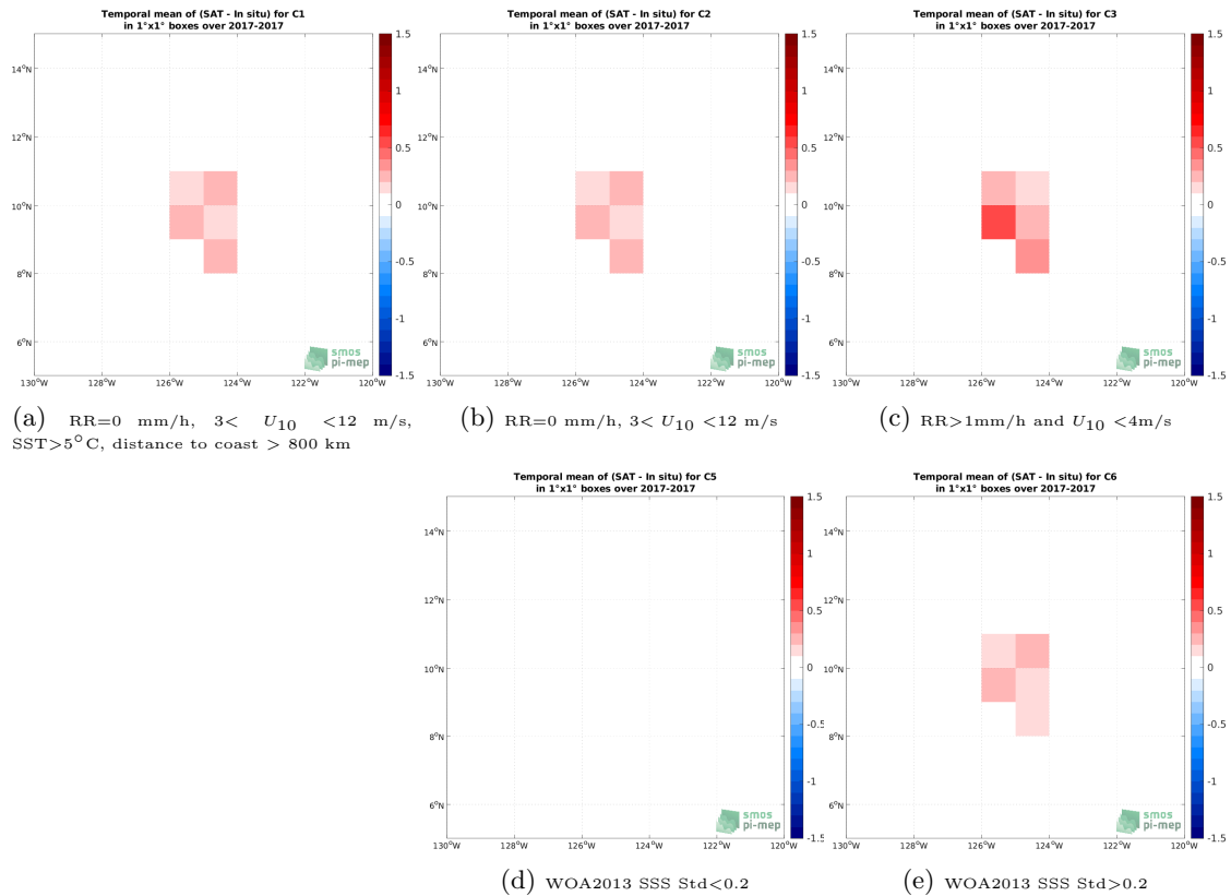
Figure 11: Temporal mean gridded over spatial boxes of size 1^\circ \times 1^\circ of \Delta\text{SSS} (SMOS and SMAP SSS L4 OI v1 - 7 Days (LOPS) - Sairdrone) for 5 different subdatasets corresponding to:RR=0 mm/h, 3 < U_{10} < 12 m/s, SST > 5^\circ\text{C} , distance to coast > 800 km (a), RR=0 mm/h, 3 < U_{10} < 12 m/s (b), RR > 1 mm/h and U_{10} < 4 m/s (c), WOA2013 SSS Std < 0.2 (d), WOA2013 SSS Std > 0.2 (e).
