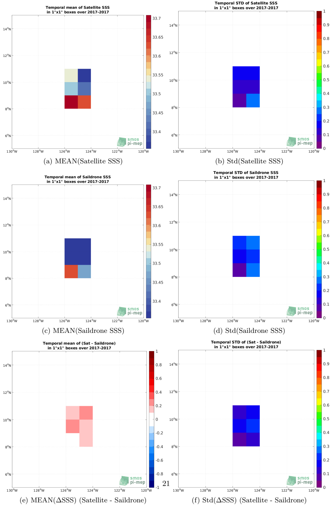
Figure 5: Temporal mean (left) and Std (right) of SSS from SMOS and SMAP SSS L4 OI v1 - 7 Days (LOPS) (top), Saildrone (middle), and of \Delta SSS (Satellite - Saildrone). Only match-up pairs are used to generate these maps.
