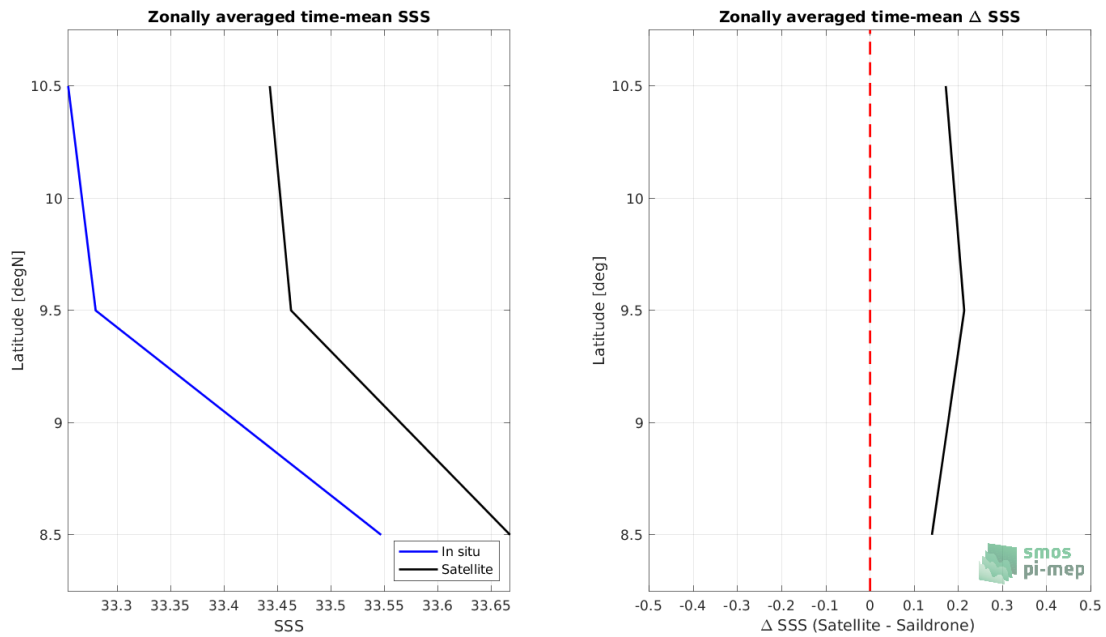
Figure 7: Left panel: Zonal mean SSS from SMOS and SMAP SSS L4 OI v1 - 7 Days (LOPS) satellite product (black) and from Sairdrone (blue). Right panel: Zonal mean of \Delta SSS (Satellite - Sairdrone) for all the collected Pi-MEP match-up pairs estimated over the full satellite product period.
