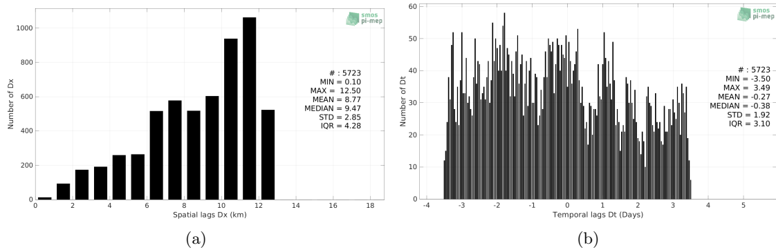
Figure 4: Histograms of the spatial (a) and temporal (b) lags between the location/time of the Saildrone measurement and the date of the corresponding SMOS and SMAP SSS L4 OI v1 - 7 Days (LOPS) SSS pixel.
