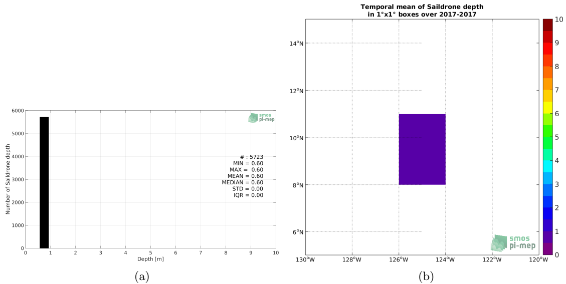
Figure 3: Histograms of the depth of the upper level SSS measurements from Sairdrone in the Match-up DataBase for the SPURS 2 Pi-MEP region (a) and temporal mean spatial distribution of pressure of the in situ SSS data over 1^\circ \times 1^\circ boxes and for the full satellite product period (b).
