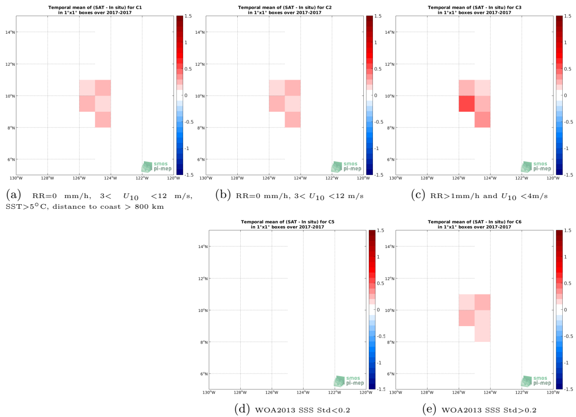
Figure 12: Temporal mean gridded over spatial boxes of size 1^\circ \times 1^\circ of \Delta\text{SSS} (SMOS and SMAP SSS L4 OI v1 - 7 Days (LOPS) - Saildrone) for 5 different subdatasets corresponding to:RR=0 mm/h, 3 < U_{10} < 12 m/s, SST >5^\circ\text{C} , distance to coast > 800 km (a), RR=0 mm/h, 3 < U_{10} < 12 m/s (b), RR >1 mm/h and U_{10} < 4 m/s (c), WOA2013 SSS Std <0.2 (d), WOA2013 SSS Std >0.2 (e).
