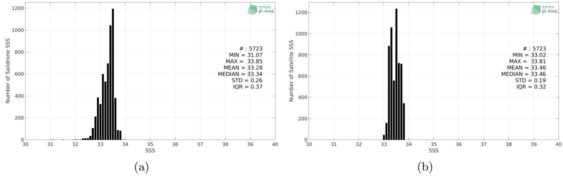
Figure 2: Histograms of SSS from Sairdrone (a) and SMOS and SMAP SSS L4 OI v1 - 7 Days (LOPS) (b) considering all match-up pairs per bins of 0.1 over the SPURS 2 Pi-MEP region and for the full satellite product period.
