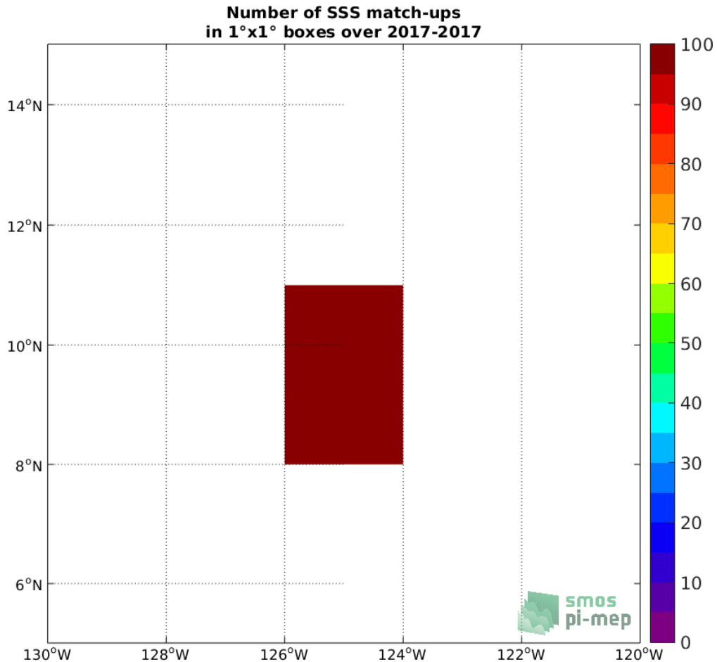
Figure 4: Number of SSS match-ups between Saildrone SSS and the SMOS and SMAP SSS L4 OI v1 - 7 Days (LOPS) SSS product for the SPURS 2 Pi-MEP region over 1^\circ \times 1^\circ boxes and for the full satellite product period.
