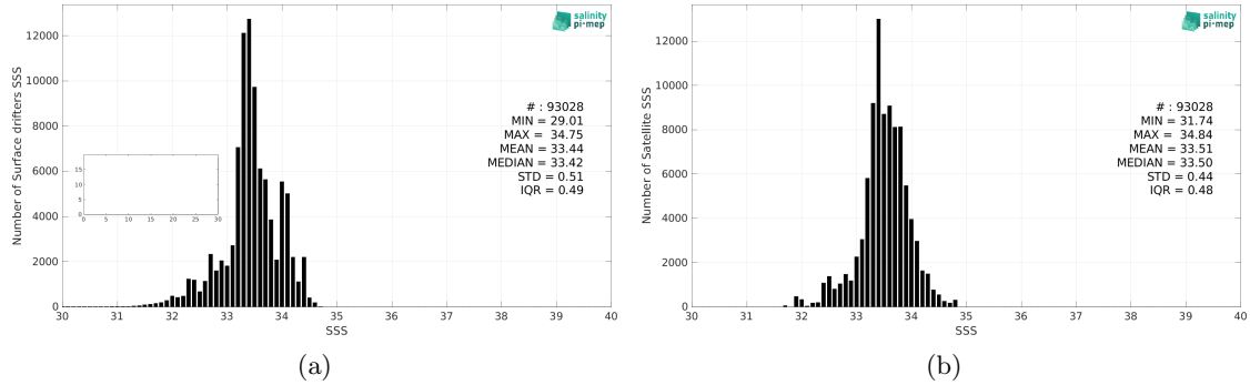
Figure 2: Histograms of SSS from Surface drifters (a) and SMOS and SMAP SSS L4 OI v1 - 7 Days (LOPS) (b) considering all match-up pairs per bins of 0.1 over the SPURS 2 Pi-MEP region and for the full satellite product period.
